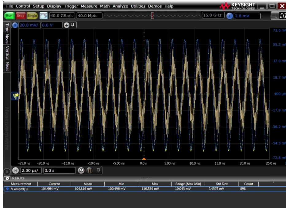
FIGURE 75. CALIBRATION TO PHASE MATCH ON KEYSIGHT SCOPE
