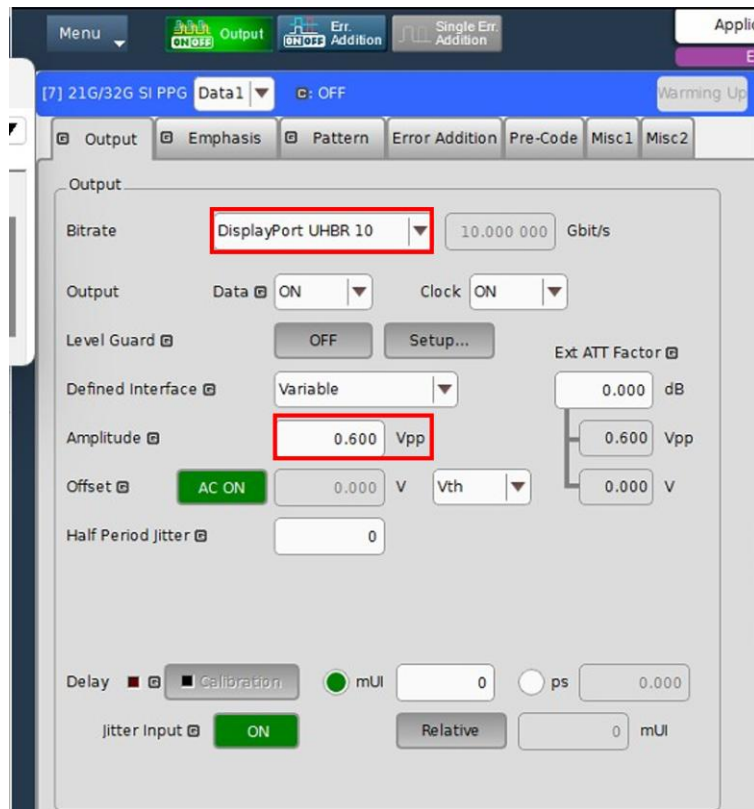
FIGURE 47. PPG OUTPUT SETTING
