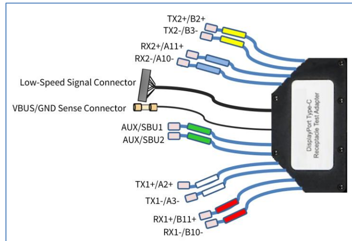
FIGURE 22. DISPLAYPORT USB TYPE-C RECEPTACLE FIXTURE CONNECTOR PIN ASSIGNMENTS
