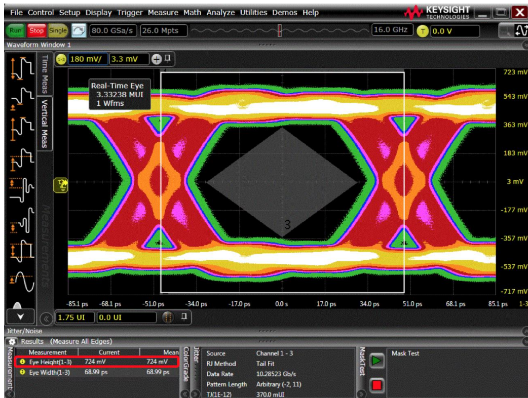
FIGURE 89. EYE MASK ON KEYSIGHT SCOPE
