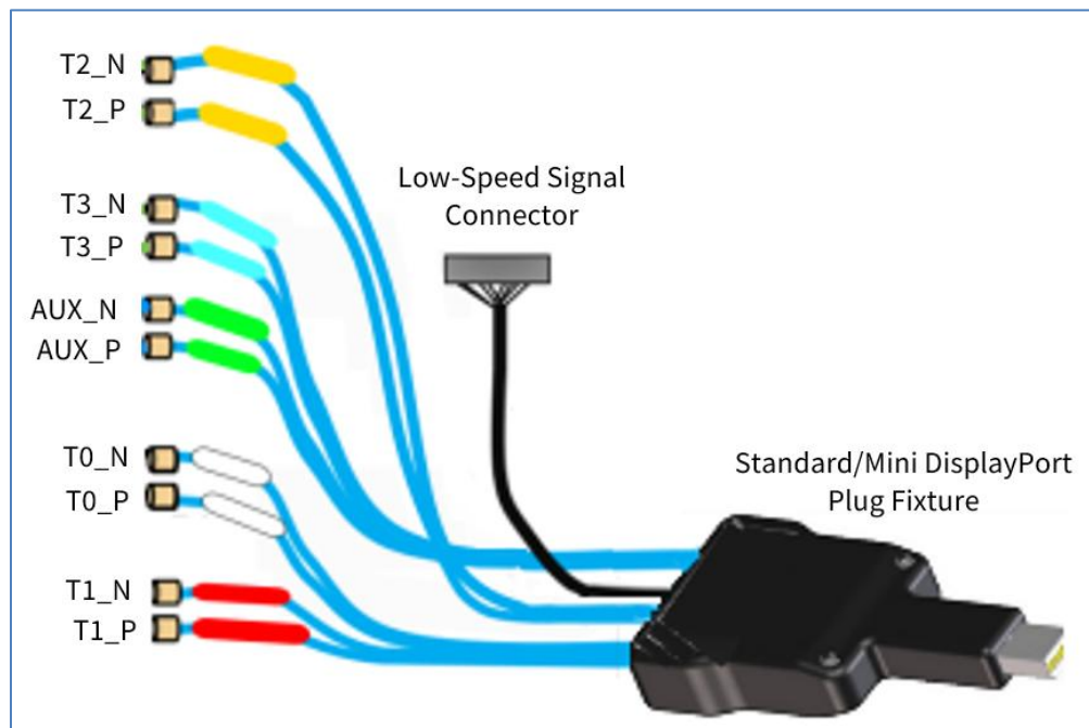
FIGURE 25. STANDARD/MINI DISPLAYPORT PLUG FIXTURE CONNECTOR PIN ASSIGNMENTS
