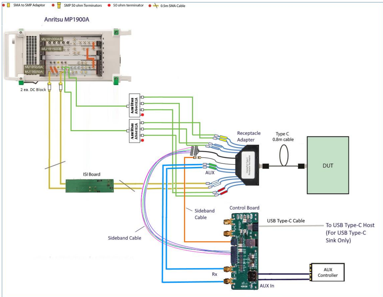
FIGURE 36. DISPLAYPORT USB TYPE-C MODE BER COMPLIANCE TEST SETUP FOR DP SINK DUT AT TP3_EQ AT 13.5G AND 20G
