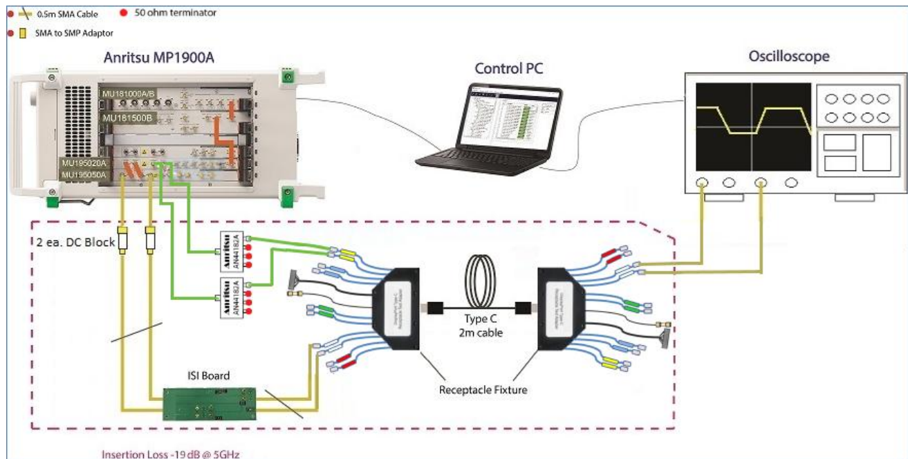
FIGURE 27. SETUP FOR TP3_EQ CALIBRATION AT 10G FOR DISPLAYPORT USB TYPE-C MODE
