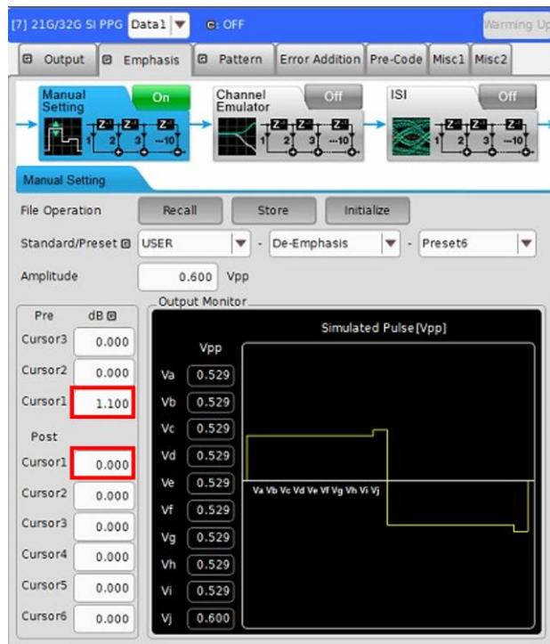
FIGURE 56. DEEMPHASIS CONFIGURATION (3)
