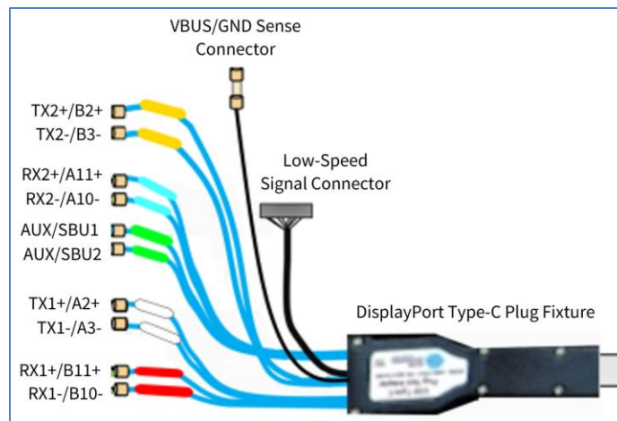
FIGURE 23. DISPLAYPORT USB TYPE-C PLUG FIXTURE CONNECTOR PIN ASSIGNMENTS
