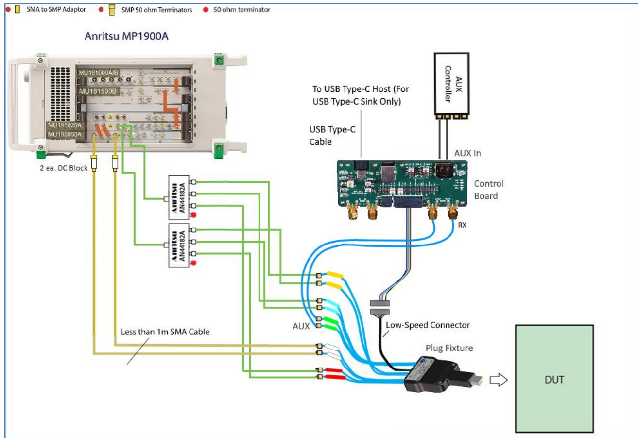
FIGURE 34. BER COMPLIANCE TEST SETUP FOR DP SINK DUT AT TP2 FOR STANDARD/MINI DISPLAYPORT MODE
