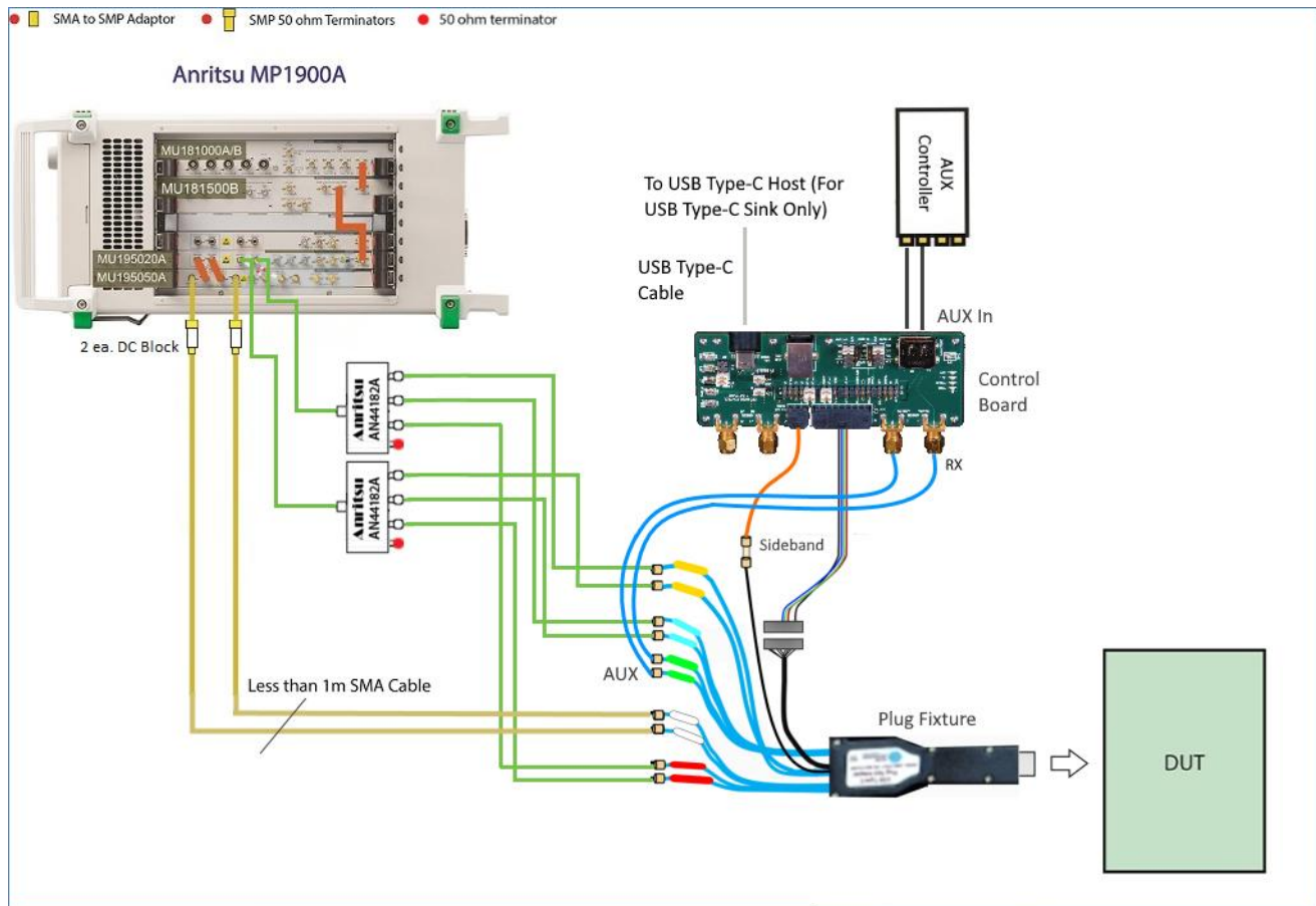
FIGURE 33. BER COMPLIANCE TEST SETUP FOR DP SINK DUT AT TP2 FOR DISPLAYPORT USB TYPE-C MODE
