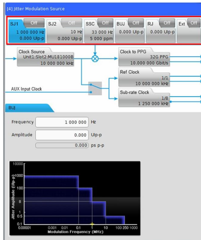
FIGURE 50. JITTER SOURCE SETTING
