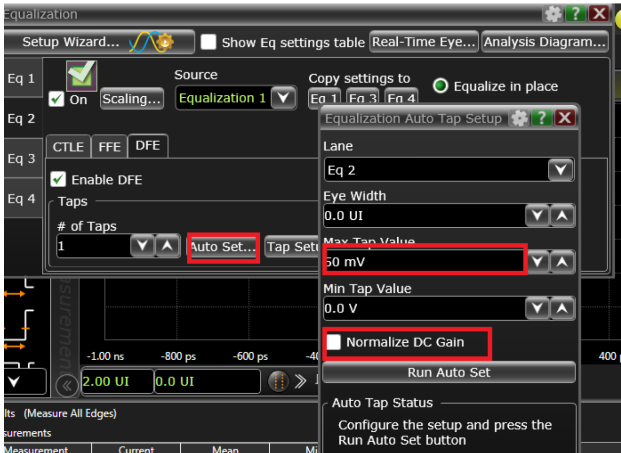
FIGURE 98. DFE SETTING
