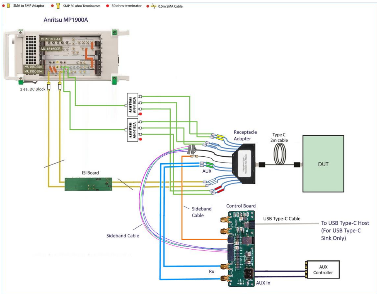
FIGURE 35. DISPLAYPORT USB TYPE-C MODE BER COMPLIANCE TEST SETUP FOR DP SINK DUT AT TP3_EQ AT 10G
