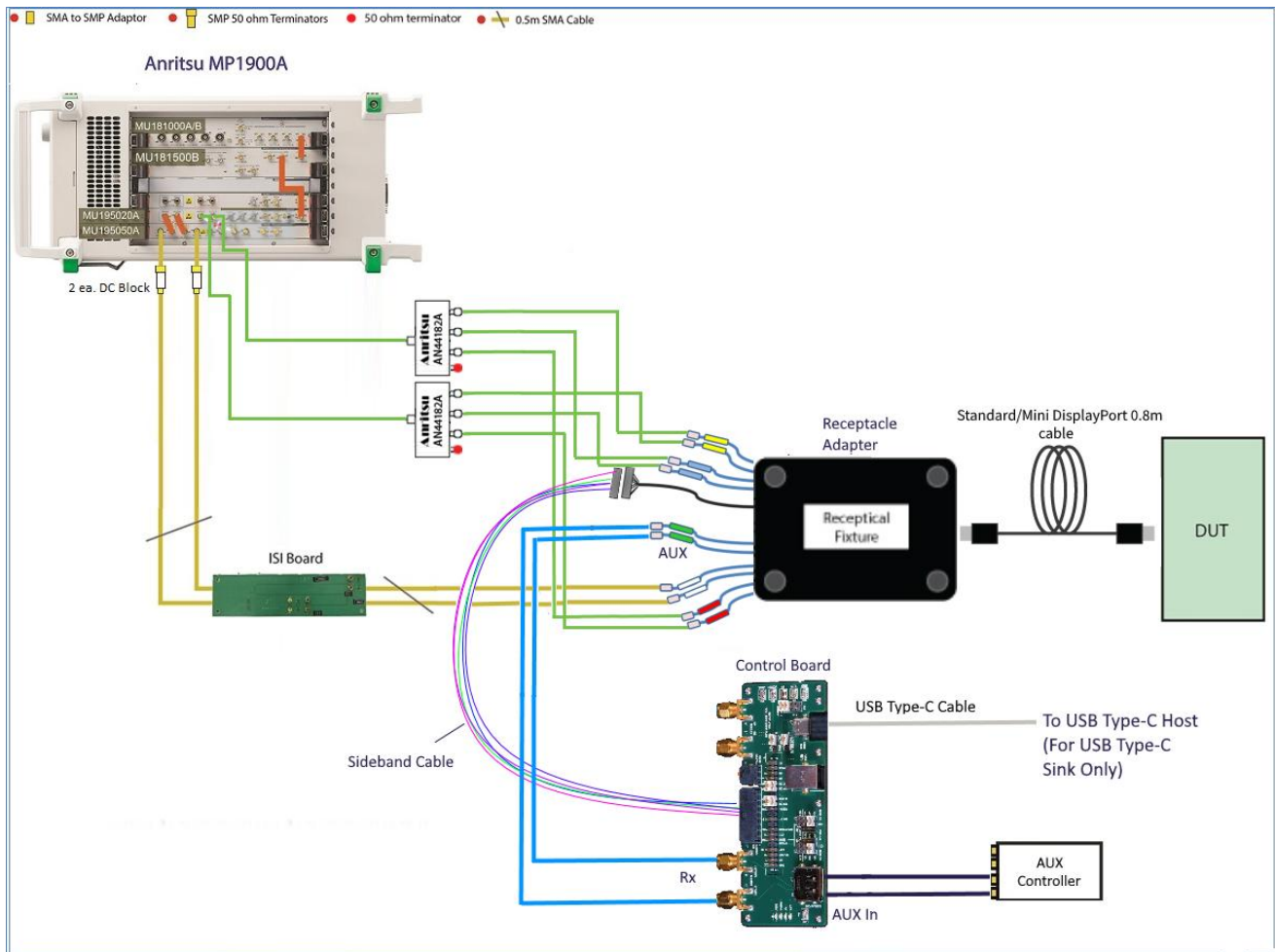
FIGURE 38. STANDARD/MINI DISPLAYPORT MODE BER COMPLIANCE TEST SETUP FOR DP SINK DUT AT TP3_EQ AT 13.5G AND 20G
