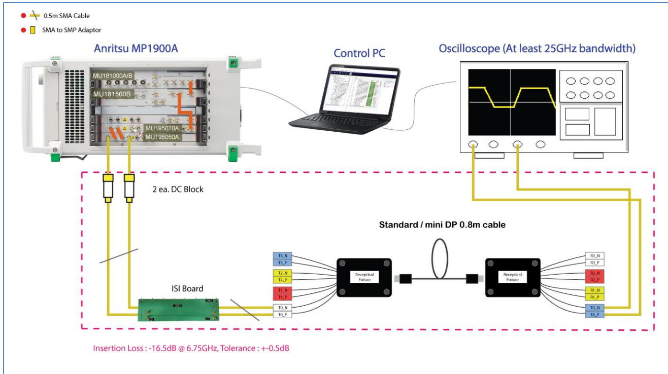
FIGURE 31. SETUP FOR TP3_EQ CALIBRATION AT 13.5G FOR STANDARD/MINI DISPLAYPORT MODE
