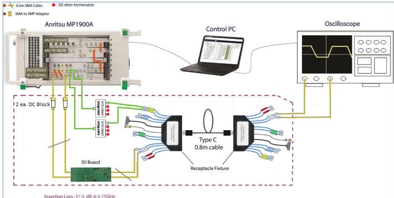
FIGURE 28. SETUP FOR TP3_EQ CALIBRATION AT 13.5G FOR DISPLAYPORT USB TYPE-C MODE
