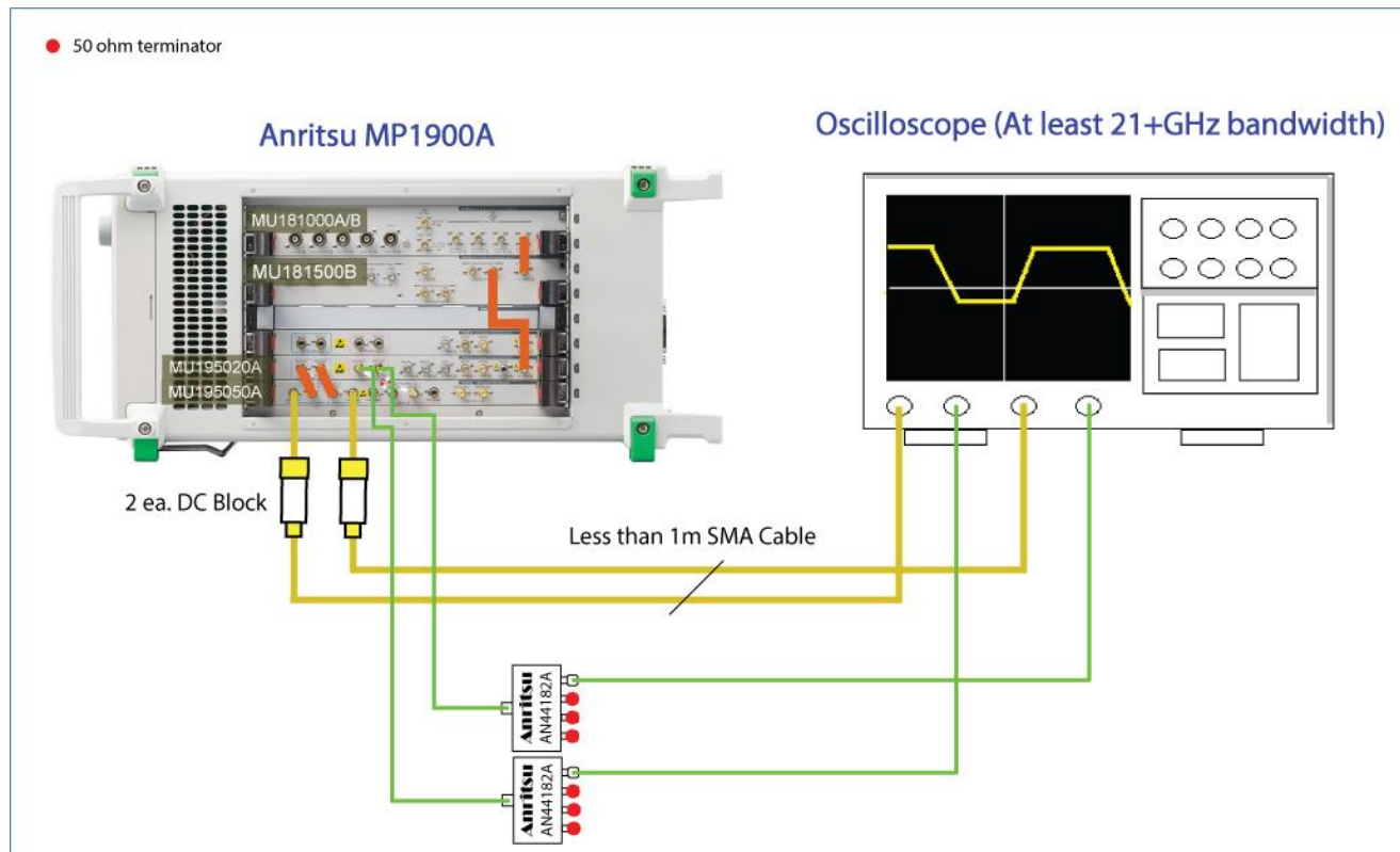
FIGURE 26. TYPICAL TP1 SINK CALIBRATION SETUP
