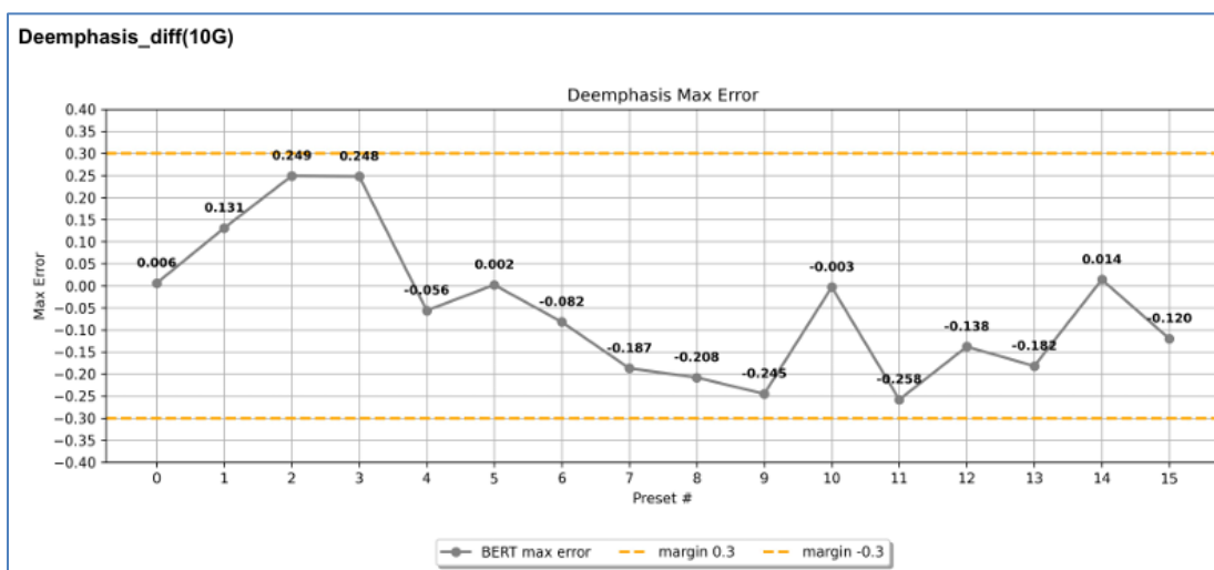
FIGURE 58. 10G PRESBOOT AND DEEMPHASIS PRESET CALIBRATION RESULT DIAGRAM EXAMPLE
