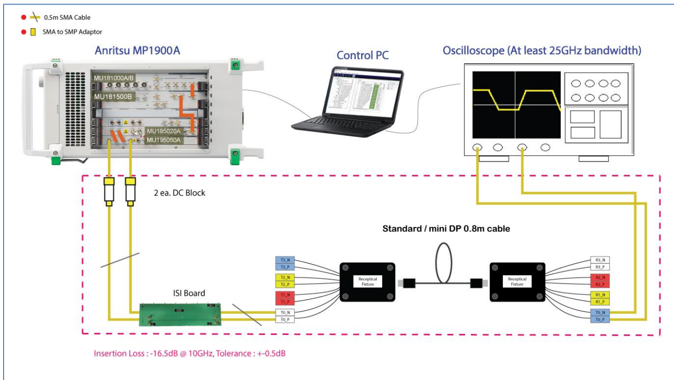
FIGURE 32. SETUP FOR TP3_EQ CALIBRATION AT 20G FOR STANDARD/MINI DISPLAYPORT MODE
