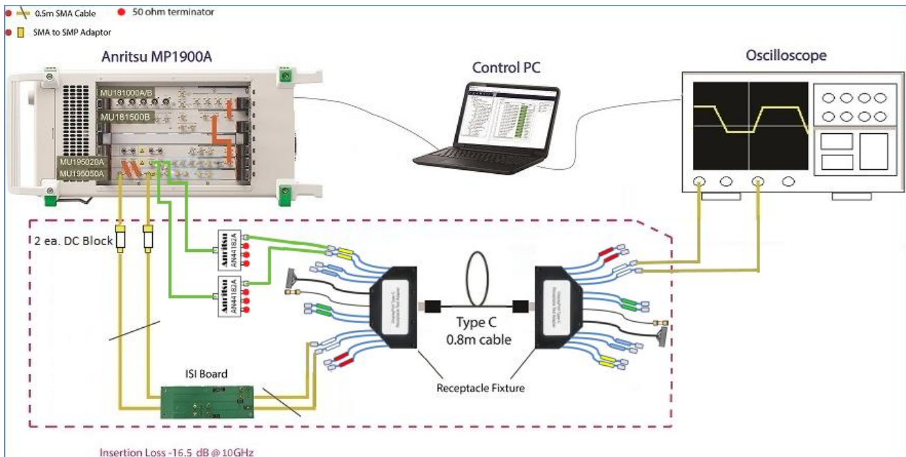
FIGURE 29. SETUP FOR TP3_EQ CALIBRATION AT 20G FOR DISPLAYPORT USB TYPE-C MODE
