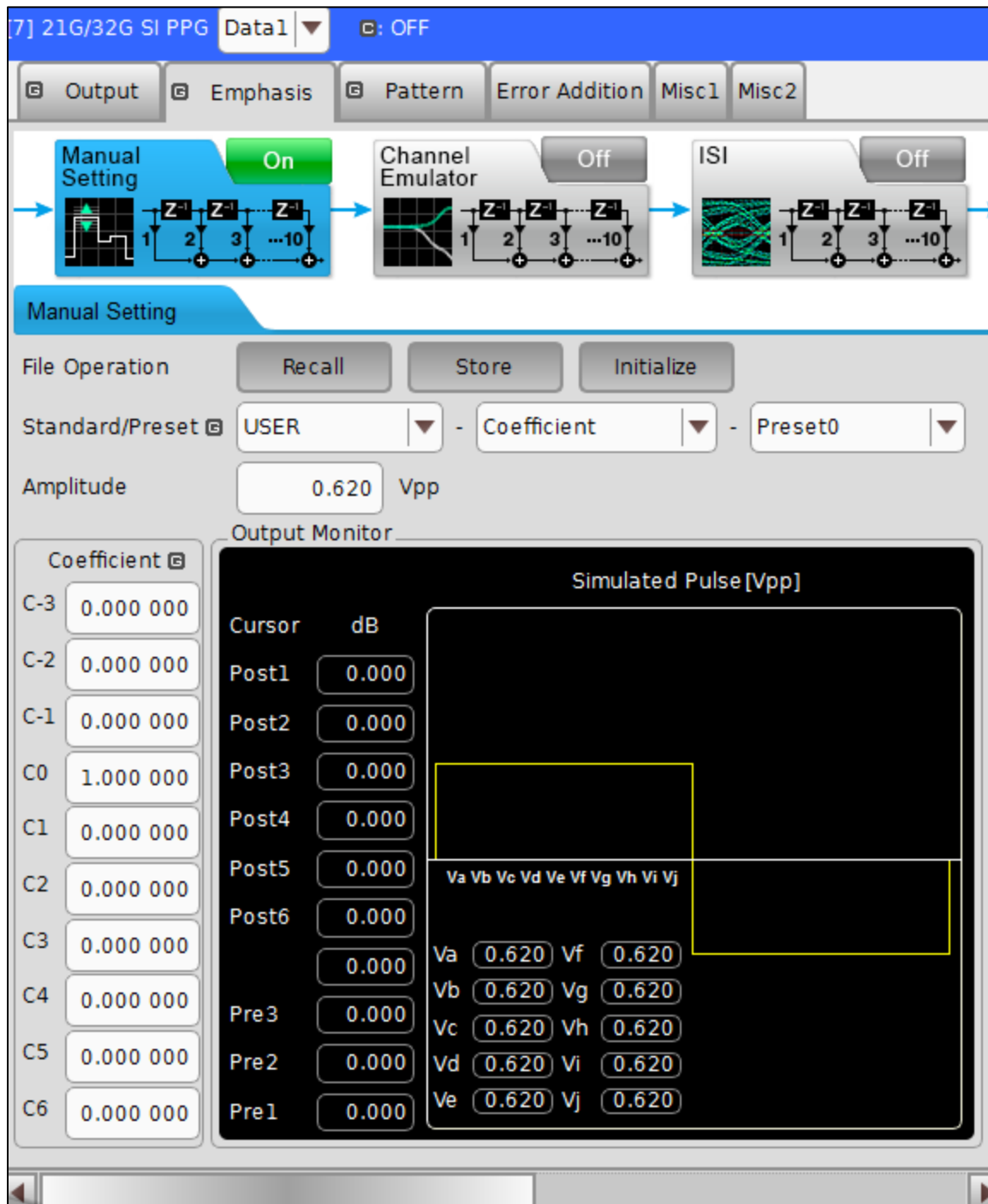
FIGURE 88. EYE AMPLITUDE
