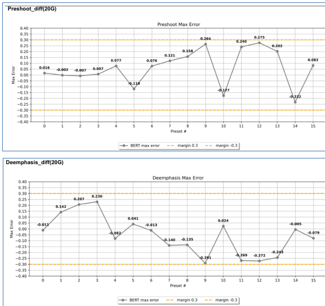
FIGURE 60. 20G PRESHOOT AND DEEMPHASIS PRESET CALIBRATION RESULT DIAGRAM EXAMPLE
