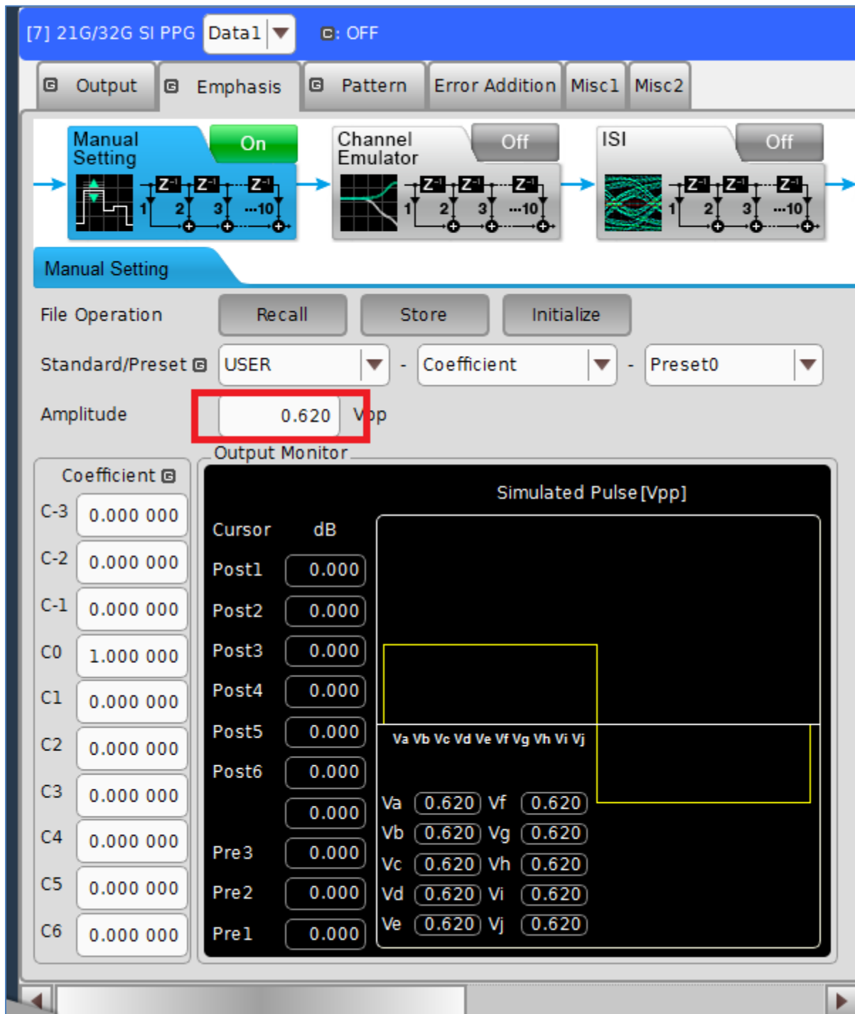
FIGURE 93. EYE AMPLITUDE
