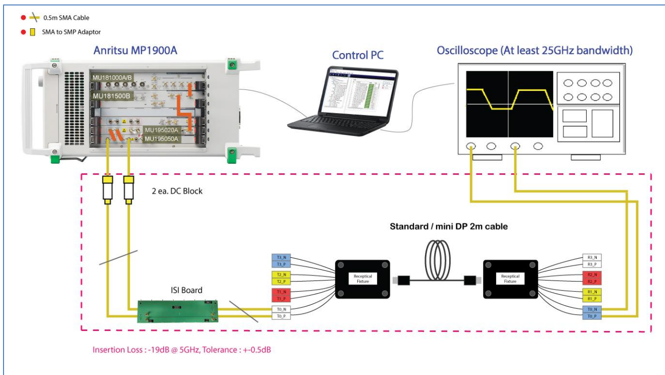
FIGURE 30. SETUP FOR TP3_EQ CALIBRATION AT 10G FOR STANDARD/MINI DISPLAYPORT MODE
