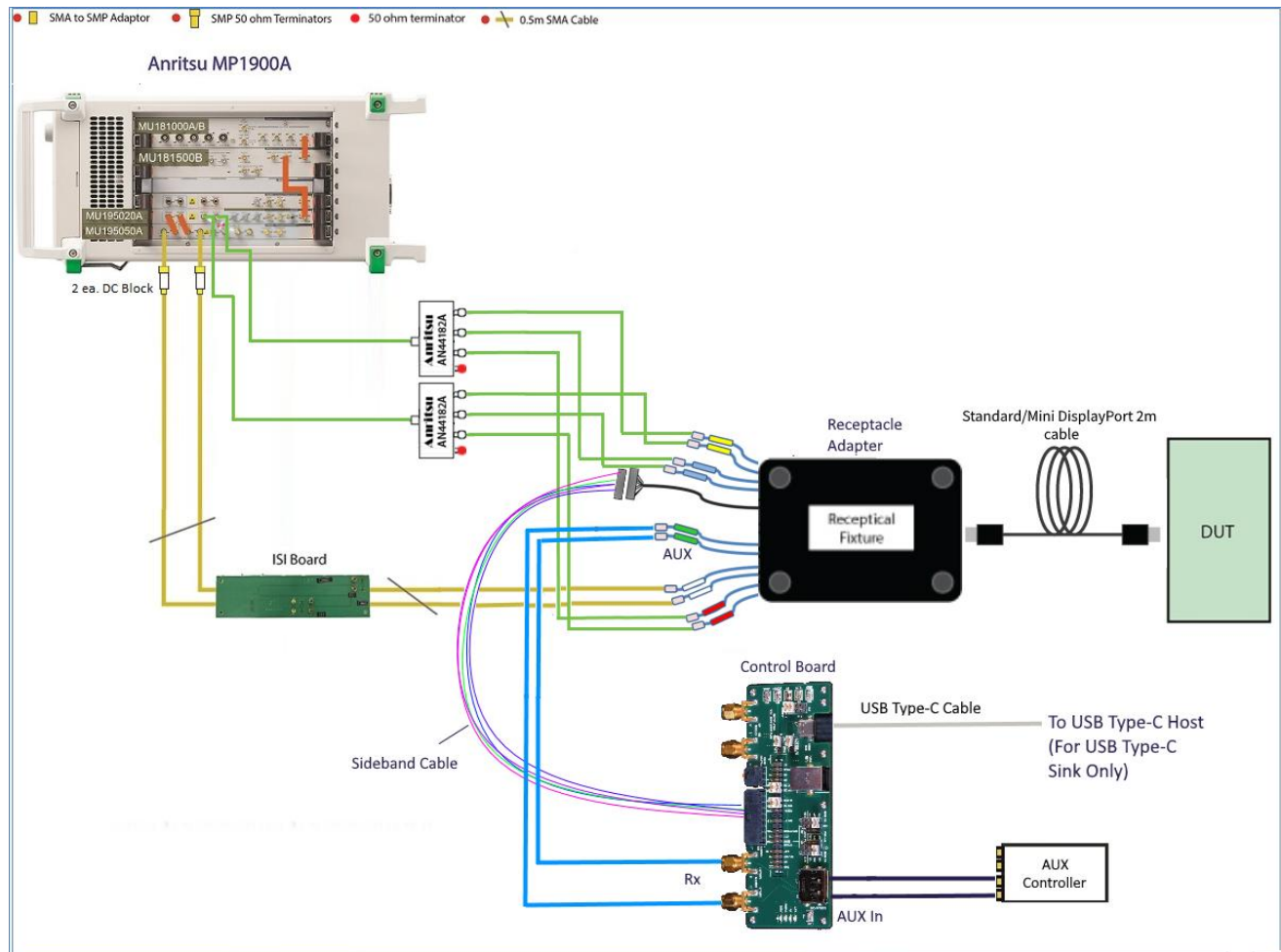
FIGURE 37. STANDARD/MINI DISPLAYPORT MODE BER COMPLIANCE TEST SETUP FOR DP SINK DUT AT TP3_EQ AT 10G
