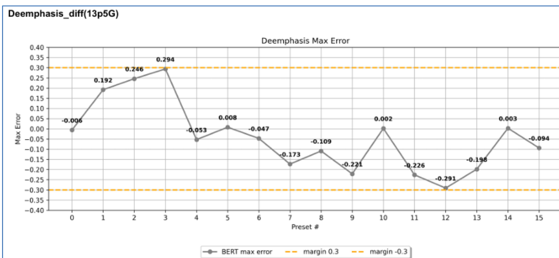
FIGURE 59. 13P5G PRESBOOT AND DEEMPHASIS PRESET CALIBRATION RESULT DIAGRAM EXAMPLE
