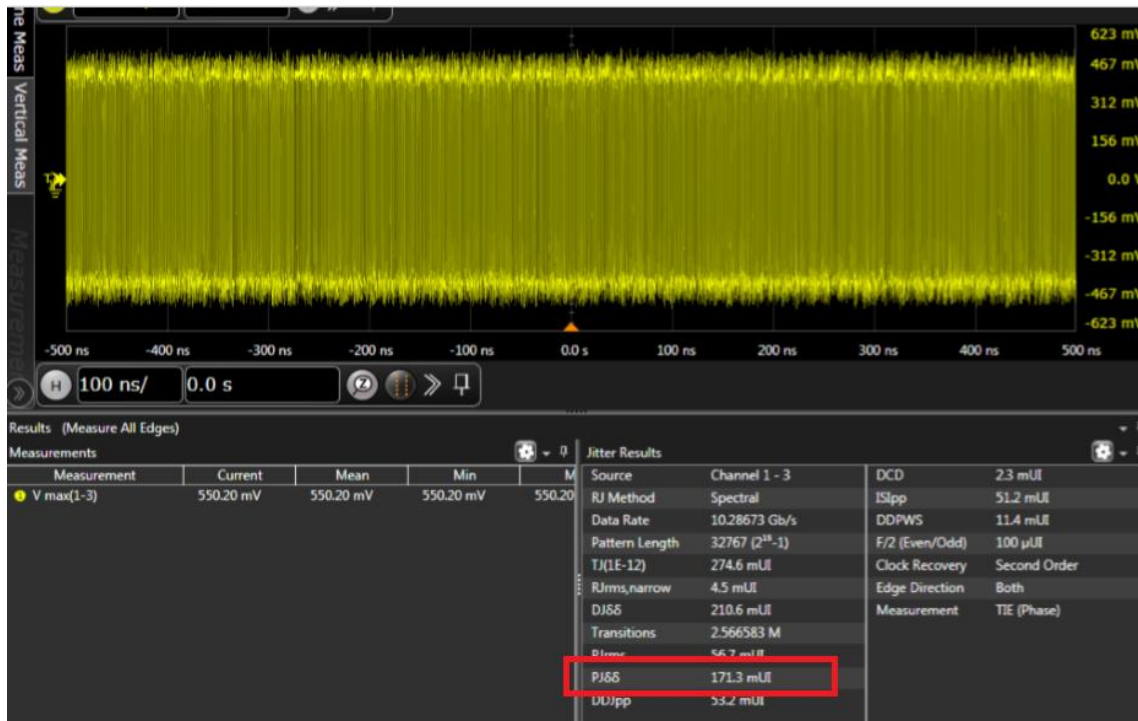
FIGURE 84. CALIBRATE SJ AMPLITUDE #2 ON KEYSIGHT SCOPE
