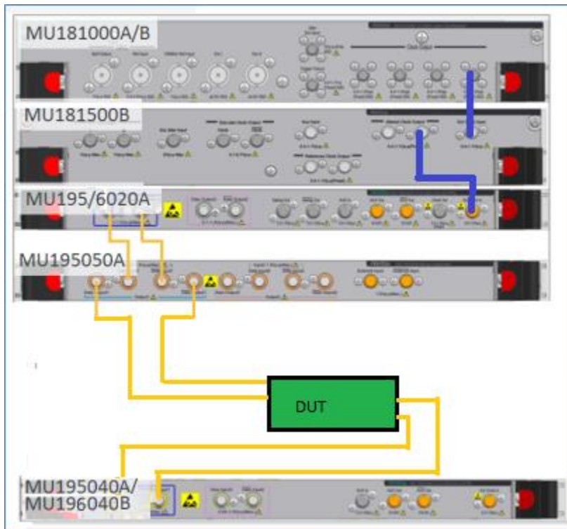
FIGURE 31. RECOMMENDED SETUP FOR DUT RX COMPLIANCE TESTING (NONE CHANNEL)
