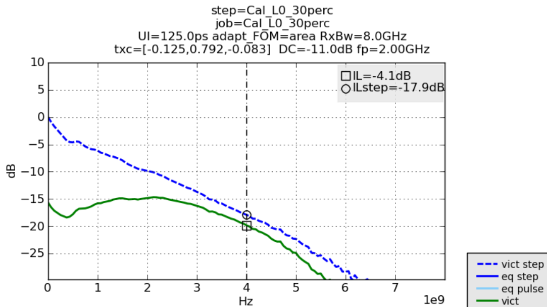
FIGURE 60. INSERTION LOSS AT 30% ISI (-17.9 dB)
