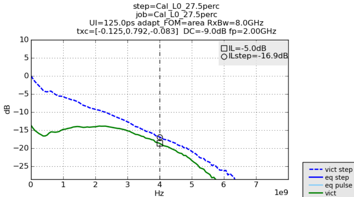
FIGURE 59. INSERTION LOSS AT 27.5% ISI (-16.9 dB)
