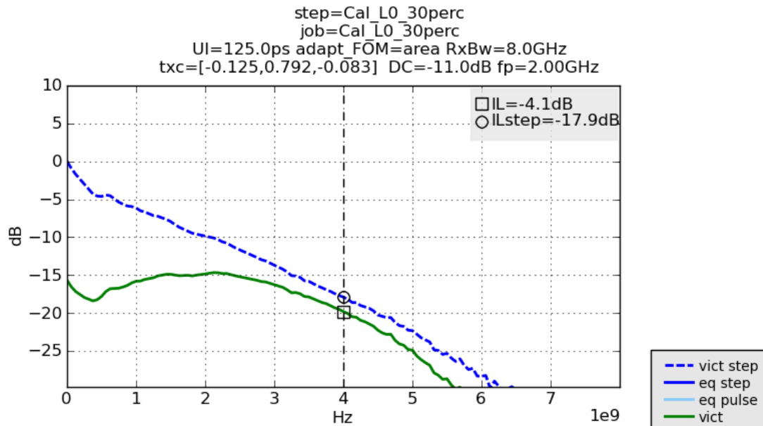
FIGURE 60. INSERTION LOSS AT 30% ISI (-17.9 dB)
