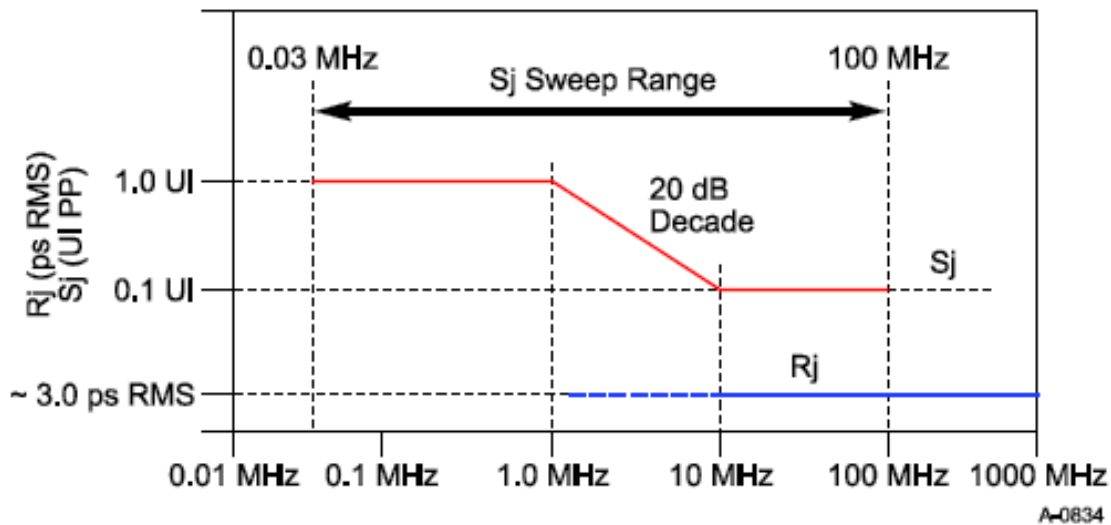
Figure 4-74: Swept Sj Mask
