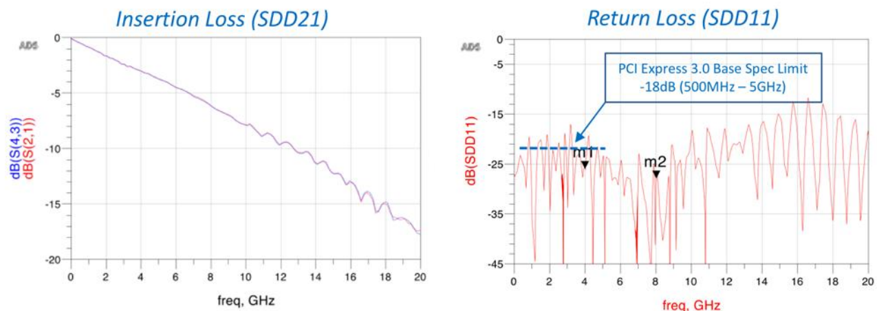
FIGURE 68. CLE1000-A2 VARIABLE ISI GENERATOR IL, RL AT 0% SETTING
