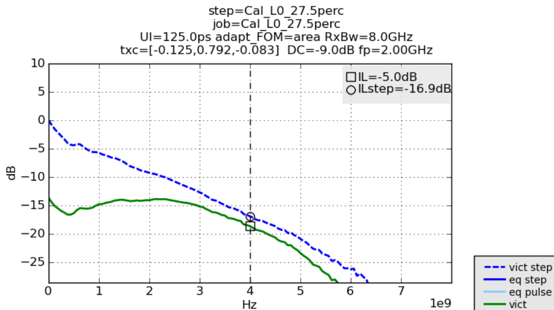
FIGURE 59. INSERTION LOSS AT 27.5% ISI (-16.9 dB)
