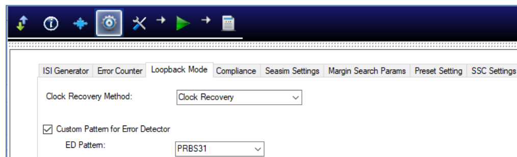
FIGURE 46. SET UP LOOPBACK TEST
