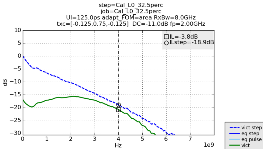
FIGURE 61. INSERTION LOSS AT 32.5% ISI (-18.9 dB) WITHIN TARGET
