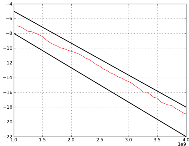
FIGURE 62. INSERTION LOSS CALIBRATION FOR LONG CHANNEL – IL FALLS BETWEEN REQUIRED MASK
