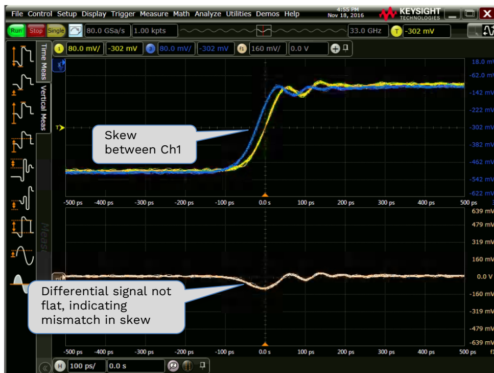
FIGURE 77. SCOPE DE-SKEW OSCILLOSCOPE DISPLAY
