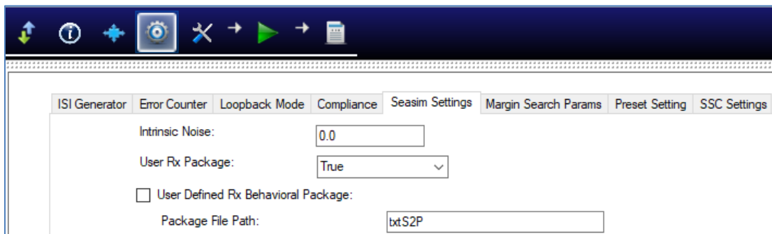
FIGURE 19. CONFIGURE SEASIM
