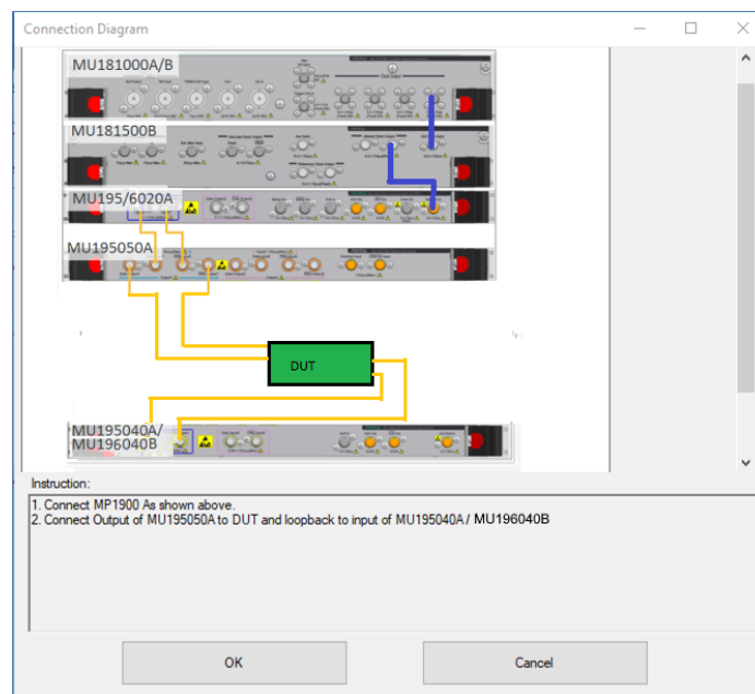
FIGURE 49. EXAMPLE CONNECTION POP-UP DIAGRAM FOR RX COMPLIANCE TEST
