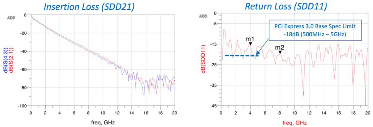
FIGURE 69. CLE1000-A2 VARIABLE ISI GENERATOR IL, RL AT 50% SETTING
