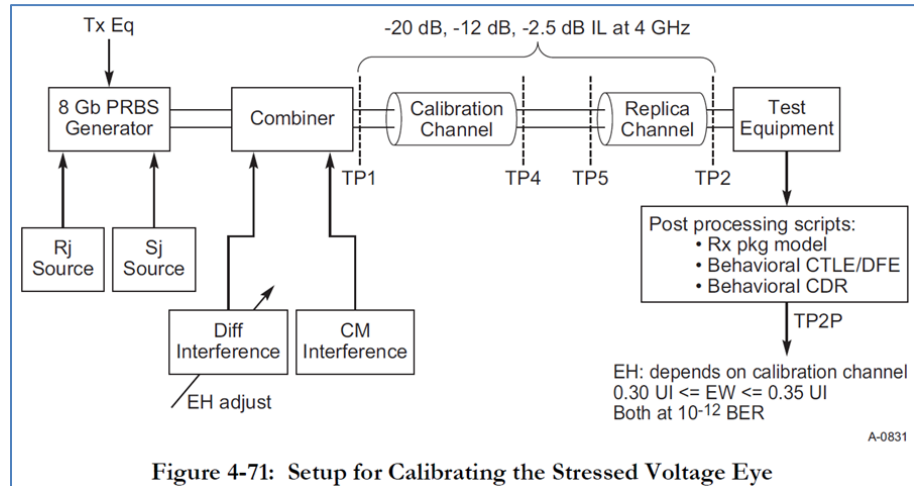
FIGURE 11. RX STRESSED VOLTAGE EYE CALIBRATION BLOCK DIAGRAM FROM PCIE GEN 3 BASE SPECIFICATION
