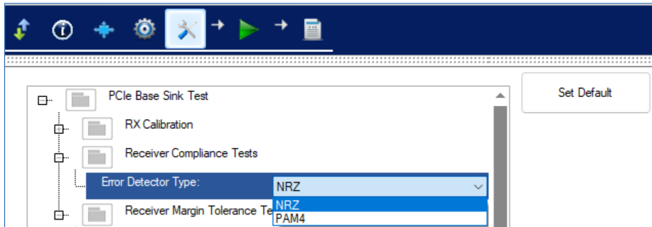
FIGURE 43. RECEIVER TEST PARAMETERS CONFIGURATION PAGE
