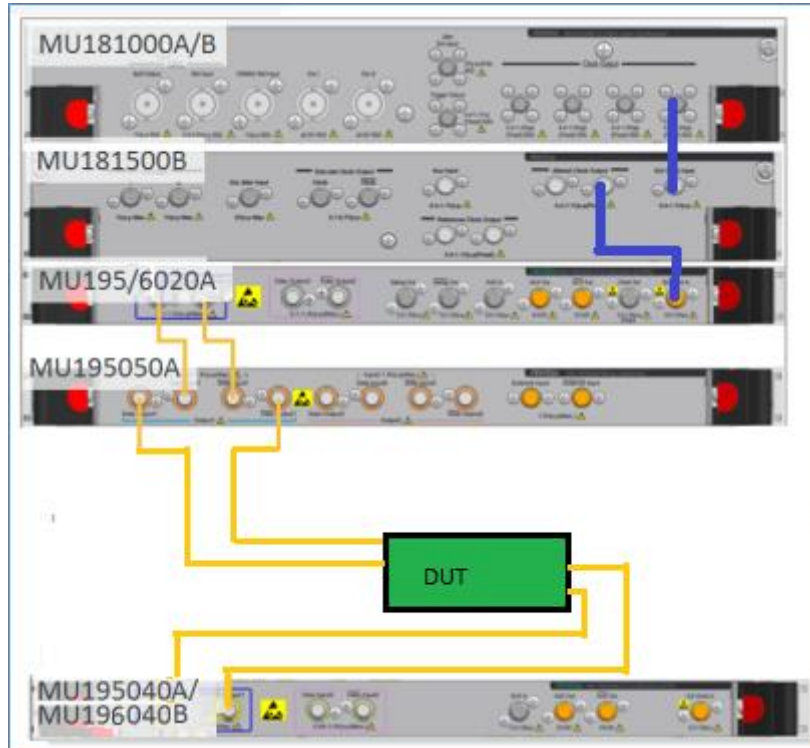
FIGURE 31. RECOMMENDED SETUP FOR DUT RX COMPLIANCE TESTING (NONE CHANNEL)
