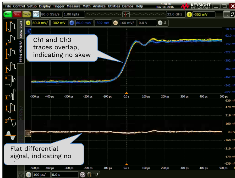
FIGURE 78. SCOPE DE-SKEW OSCILLOSCOPE DISPLAY DE-SKEWED
