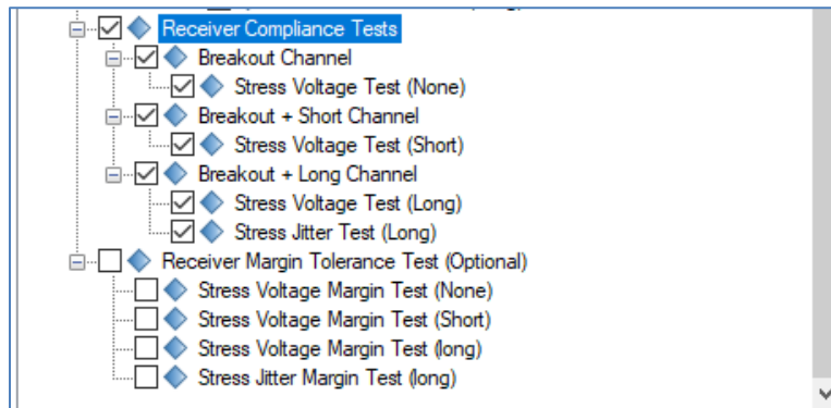
FIGURE 38. SELECT RX DUT TESTS
