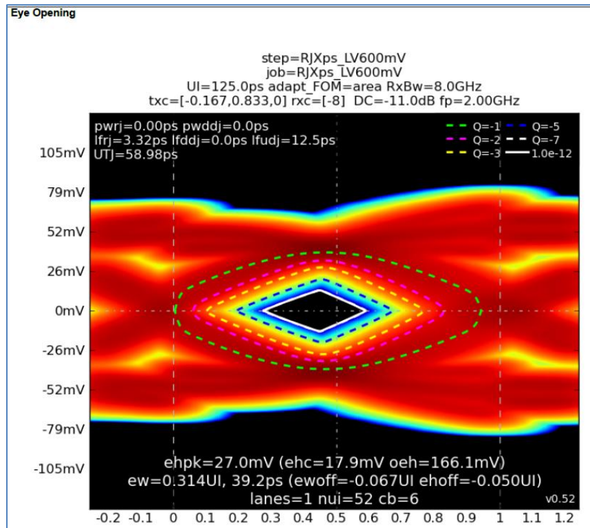
FIGURE 53. TEST RESULTS EXAMPLE
