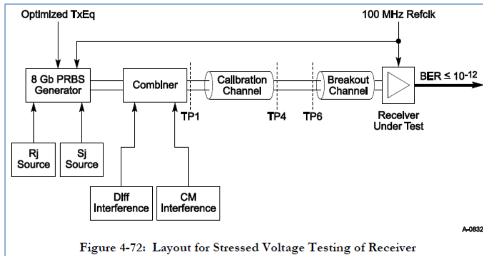
FIGURE 29. RX DUT STRESSED VOLTAGE TEST BLOCK DIAGRAM FROM PCIe GEN 3 BASE SPECIFICATION
