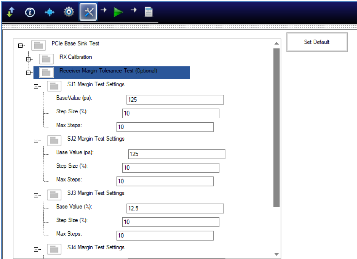
FIGURE 44. MARGIN TEST CONFIGURATION PAGE
