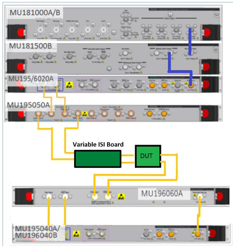
FIGURE 32. TYPICAL RECEIVER DUT TEST SETUP (USING MP1900A BERT)
