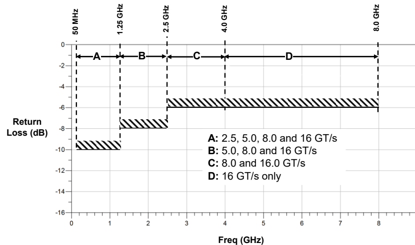
FIGURE 53. Differential Mode Return Loss Mask
