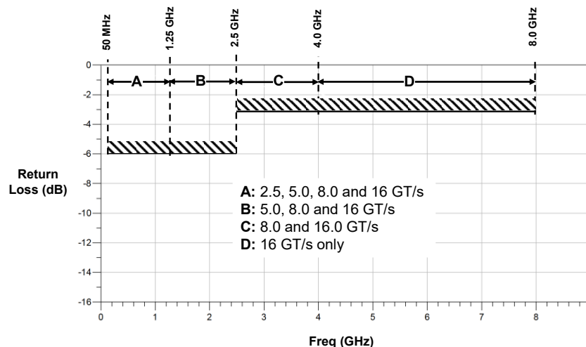
FIGURE 54. Common Mode Return Loss Mask
