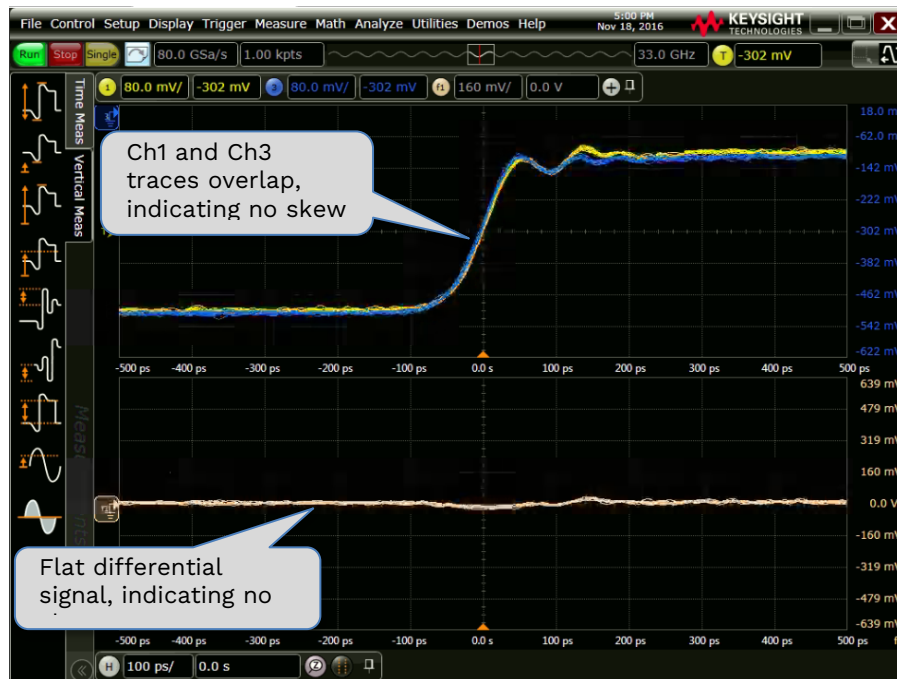
FIGURE 63. SCOPE DE-SKEW OSCILLOSCOPE DISPLAY DE-SKEWED
