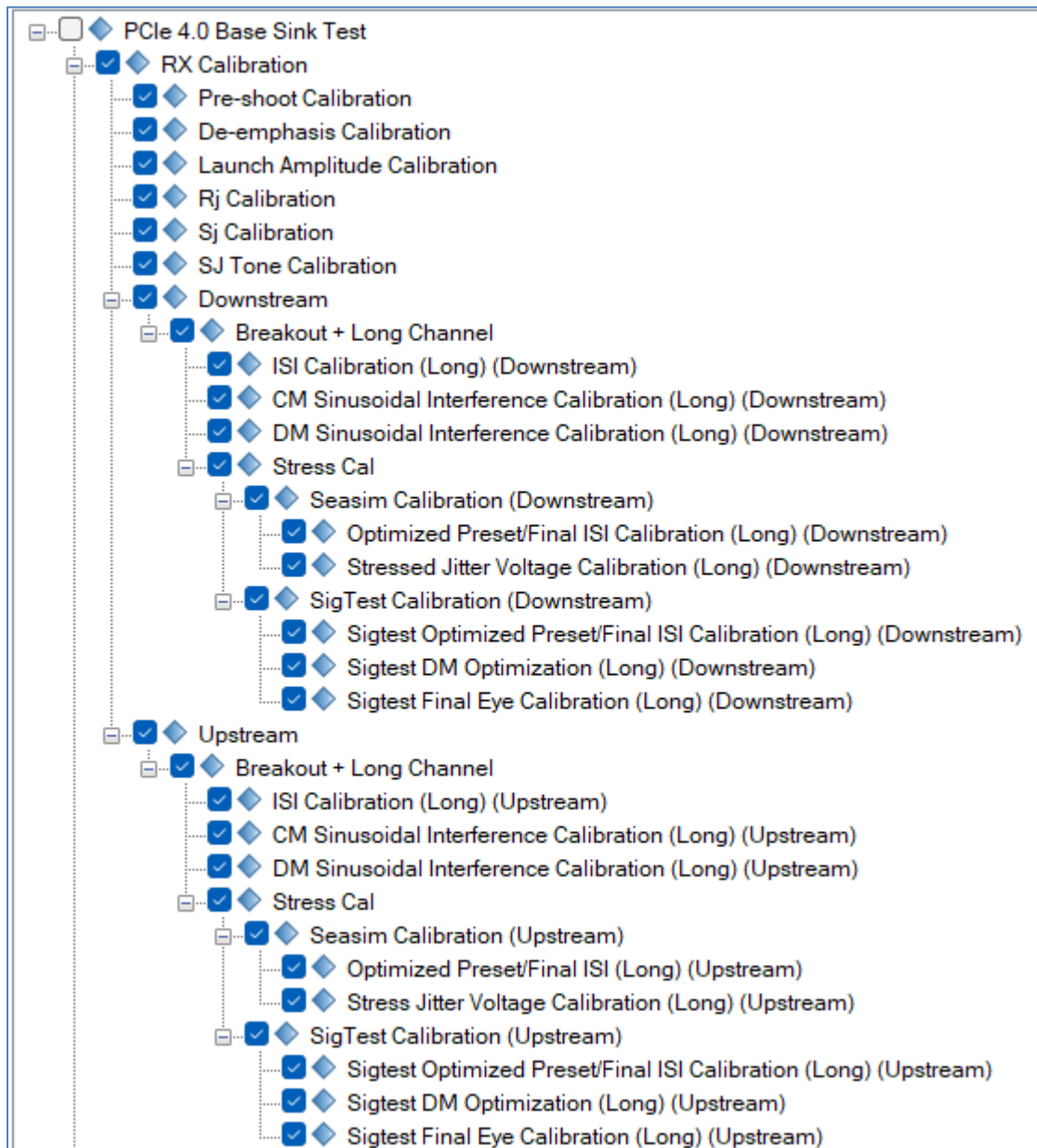
FIGURE 23. CALIBRATION SELECTION
