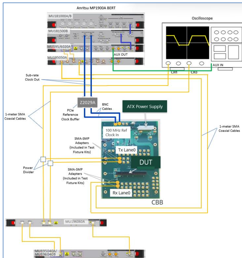
FIGURE 57. CONNECTION DIAGRAM FOR PCIe GEN 3/4 ADD-IN CARD DUT INITIAL TX EQ / TX LINK EQ RESPONSE TEST
