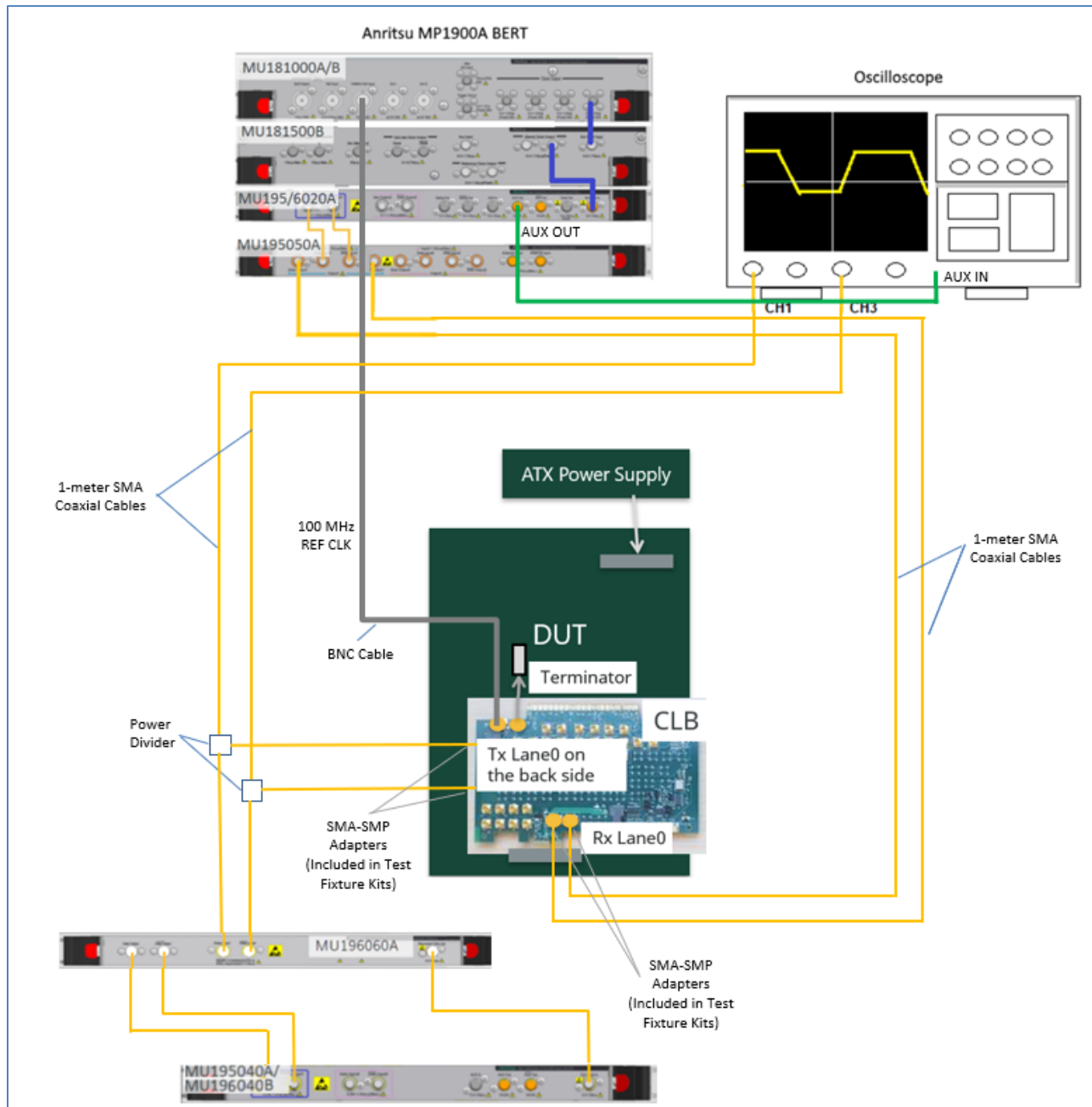
FIGURE 58. CONNECTION DIAGRAM FOR PCIe GEN 3/4 SYSTEM BOARD DUT TX LINK EQ RESPONSE TEST
