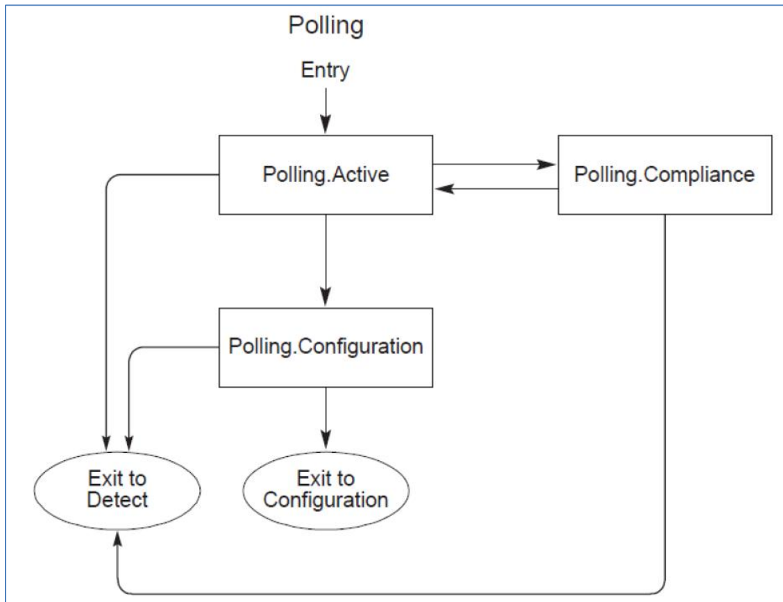
FIGURE 30. POLLING SUBSTATE MACHINE (FROM CTS)
