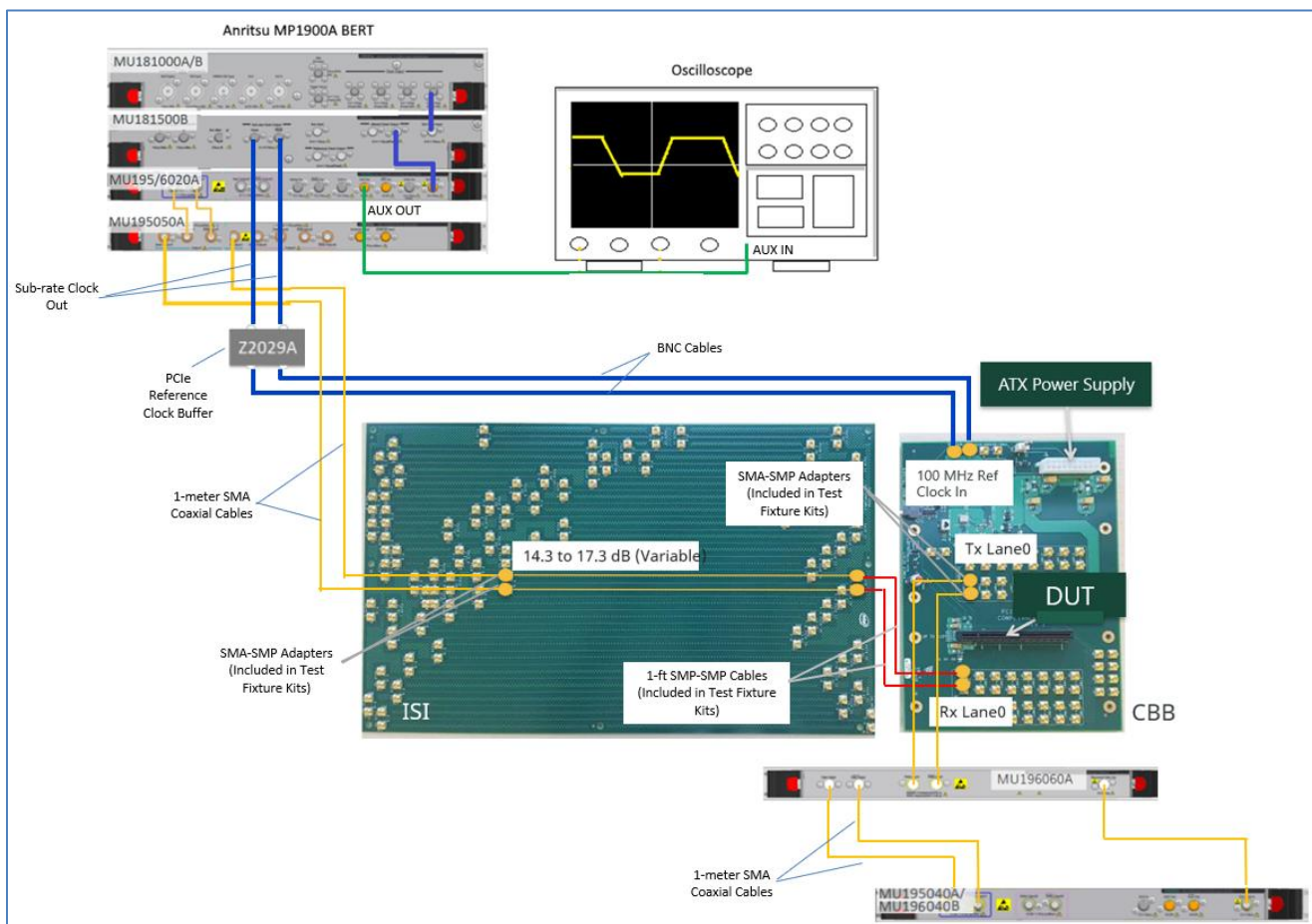
FIGURE 35. RECOMMENDED SETUP FOR DUT RX COMPLIANCE TESTING (PCIe GEN 4 ADD-IN CARD)
