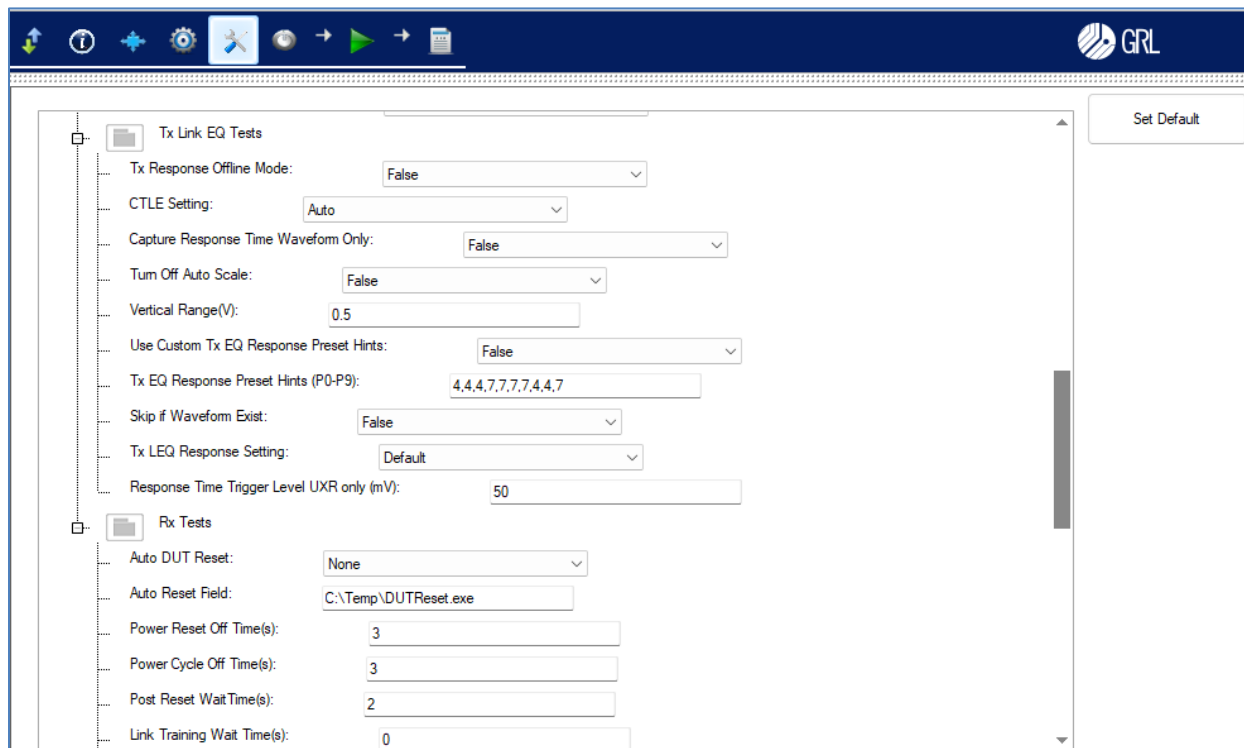
FIGURE 42. TEST PARAMETERS CONFIGURATION PAGE
