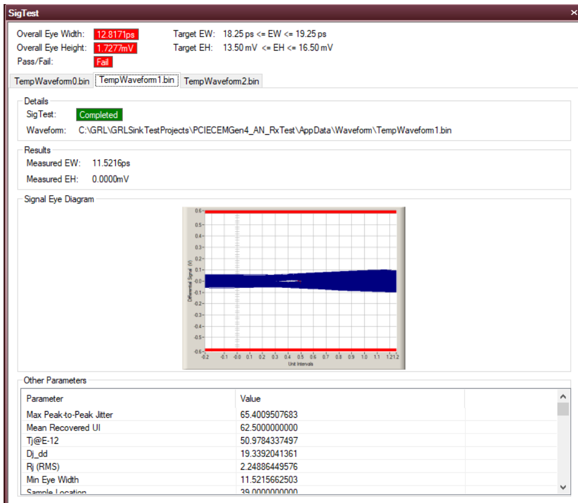
FIGURE 64. VIEWING SIGTEST ANALYSIS RESULTS
