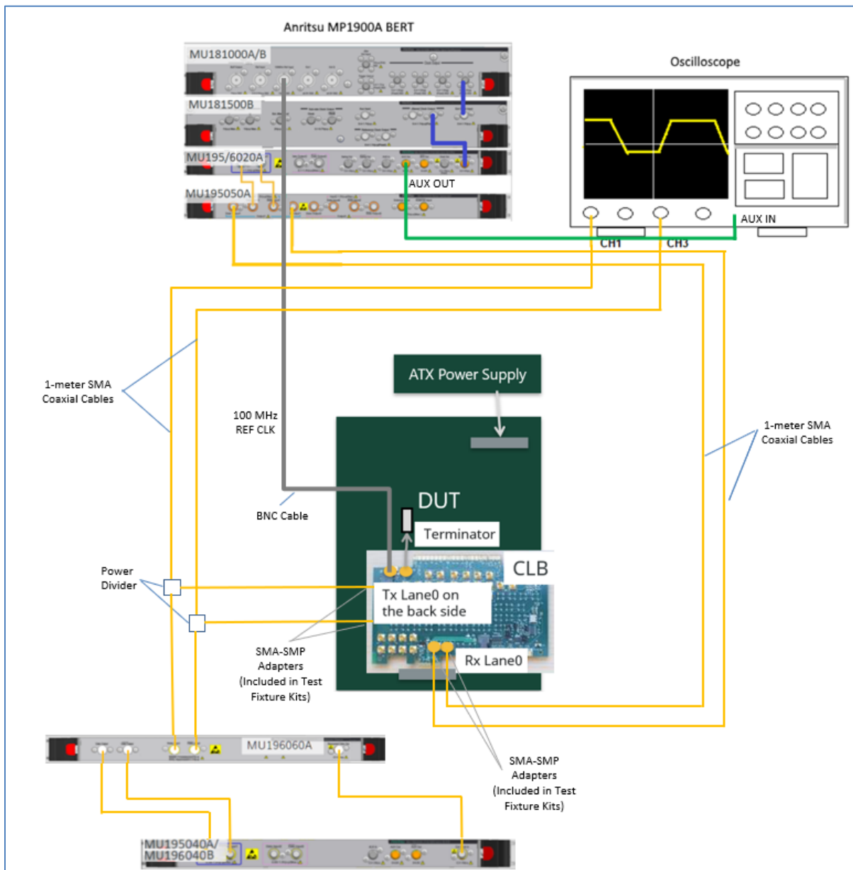
FIGURE 31. RECOMMENDED SETUP FOR DUT TX LINK EQ TESTING (PCIe GEN 3/4 SYSTEM BOARD)
