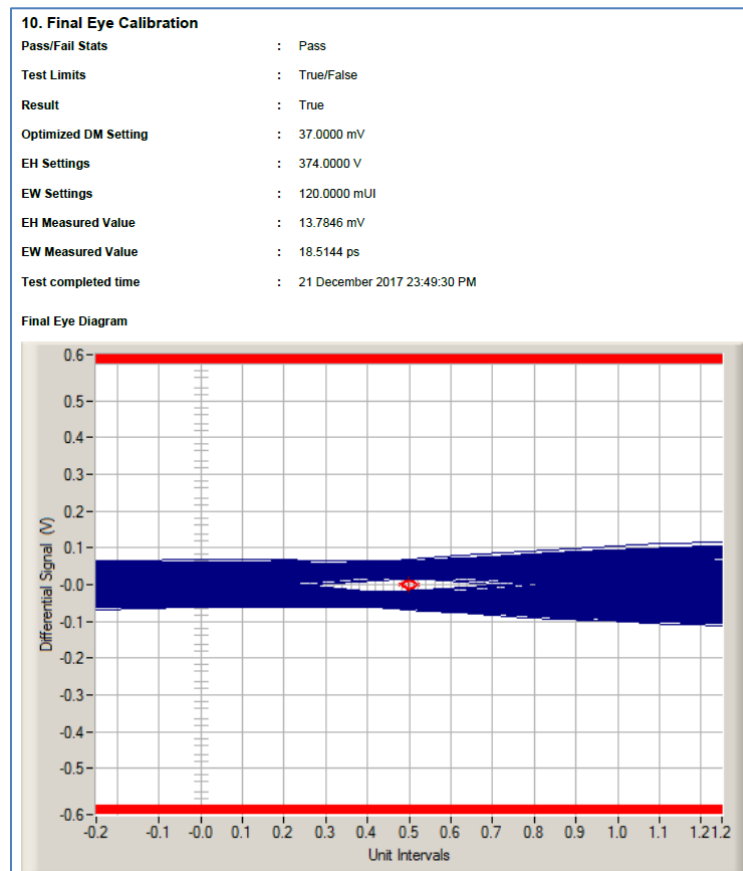
FIGURE 49. TEST RESULTS EXAMPLE
