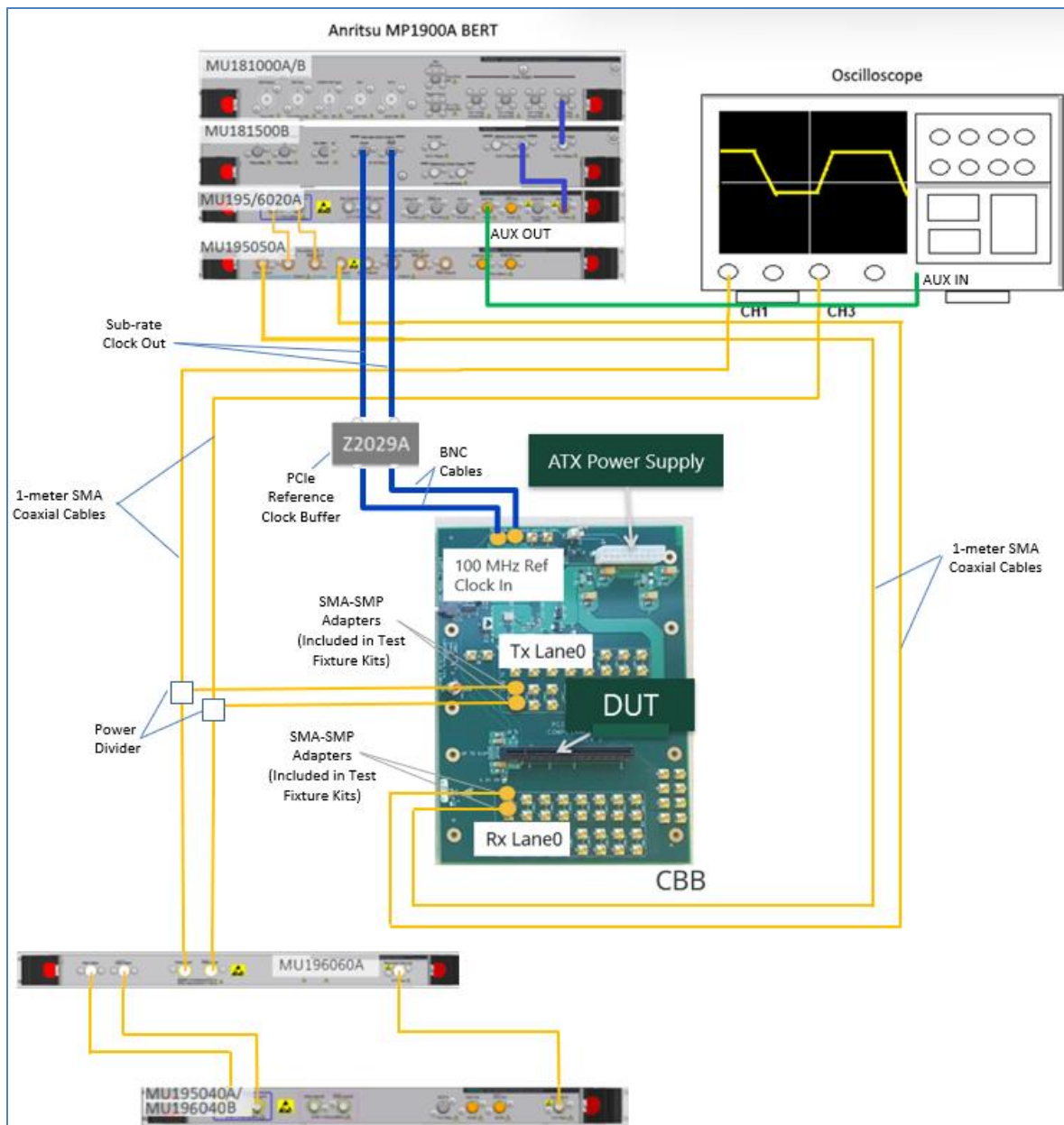
FIGURE 32. RECOMMENDED SETUP FOR DUT TX LINK EQ TESTING (PCIe GEN 3/4 ADD-IN CARD)
