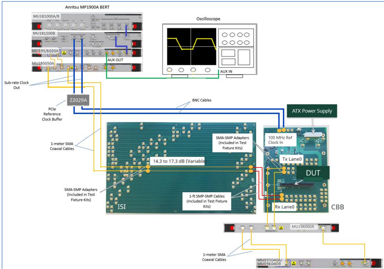
FIGURE 59. CONNECTION DIAGRAM FOR PCIe GEN 4 ADD-IN CARD DUT LOOPBACK TEST
