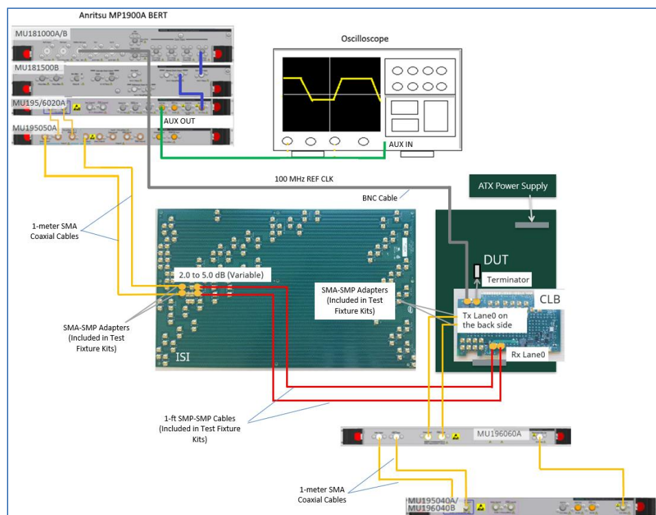
FIGURE 33. RECOMMENDED SETUP FOR DUT RX COMPLIANCE TESTING (PCIe GEN 4 SYSTEM BOARD)
