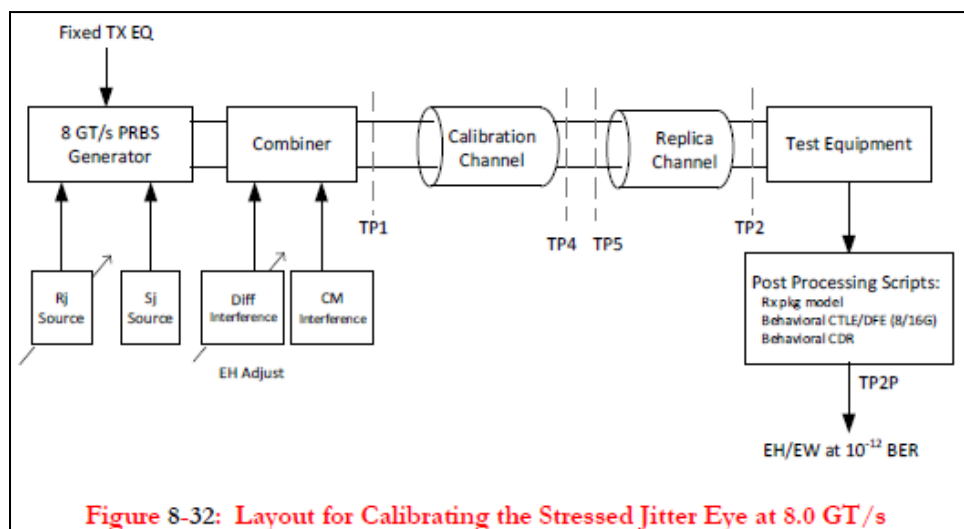
FIGURE 52. CTS RX CALIBRATION DIAGRAM FOR PCIe GEN 3
