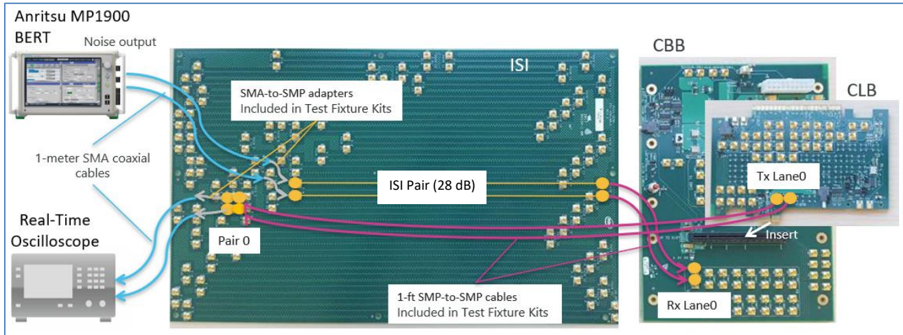
FIGURE 62. CONNECTION DIAGRAM FOR PCIe GEN 4 DM-I, CM-I AND EH/EW TP2 CALIBRATION
