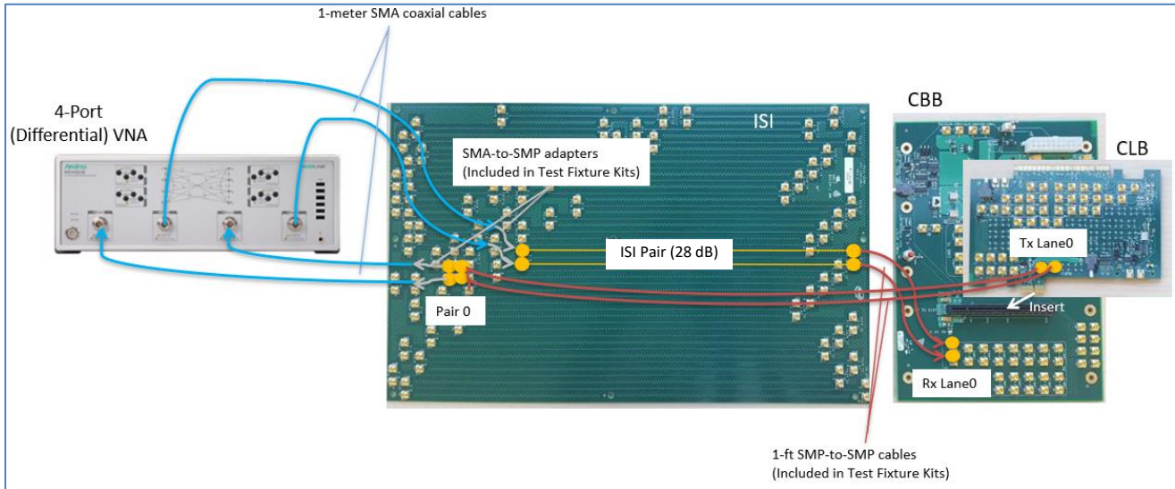
FIGURE 60. CONNECTION DIAGRAM FOR CHANNEL LOSS CALIBRATION
