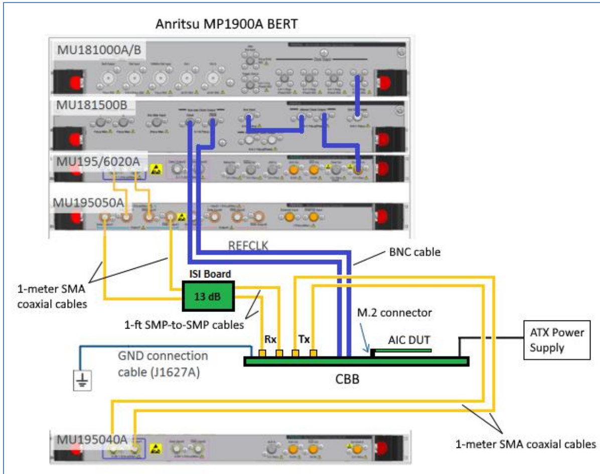
FIGURE 41. RECOMMENDED SETUP FOR DUT M.2 RX COMPLIANCE TESTING (PCIe GEN 3 ADD-IN CARD)
