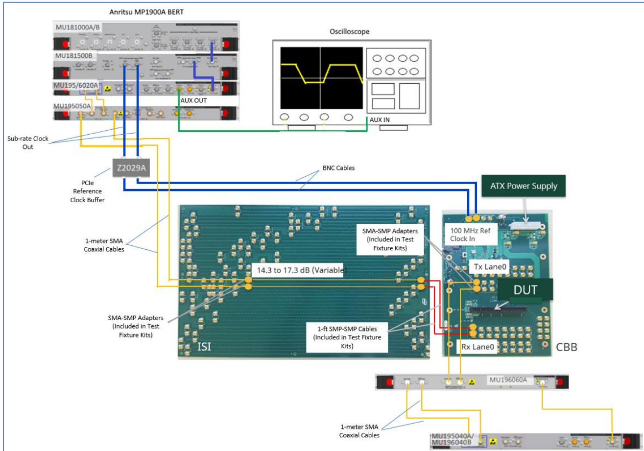
FIGURE 65. CONNECTION DIAGRAM FOR PCIe GEN 4 ADD-IN CARD DUT LOOPBACK TEST
