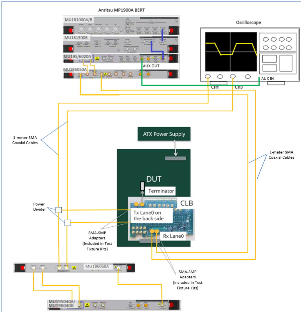
FIGURE 32. RECOMMENDED SETUP FOR DUT TX LINK EQ TESTING (PCIe GEN 3/4 SYSTEM BOARD) IN THE IR REFCLK MODE
