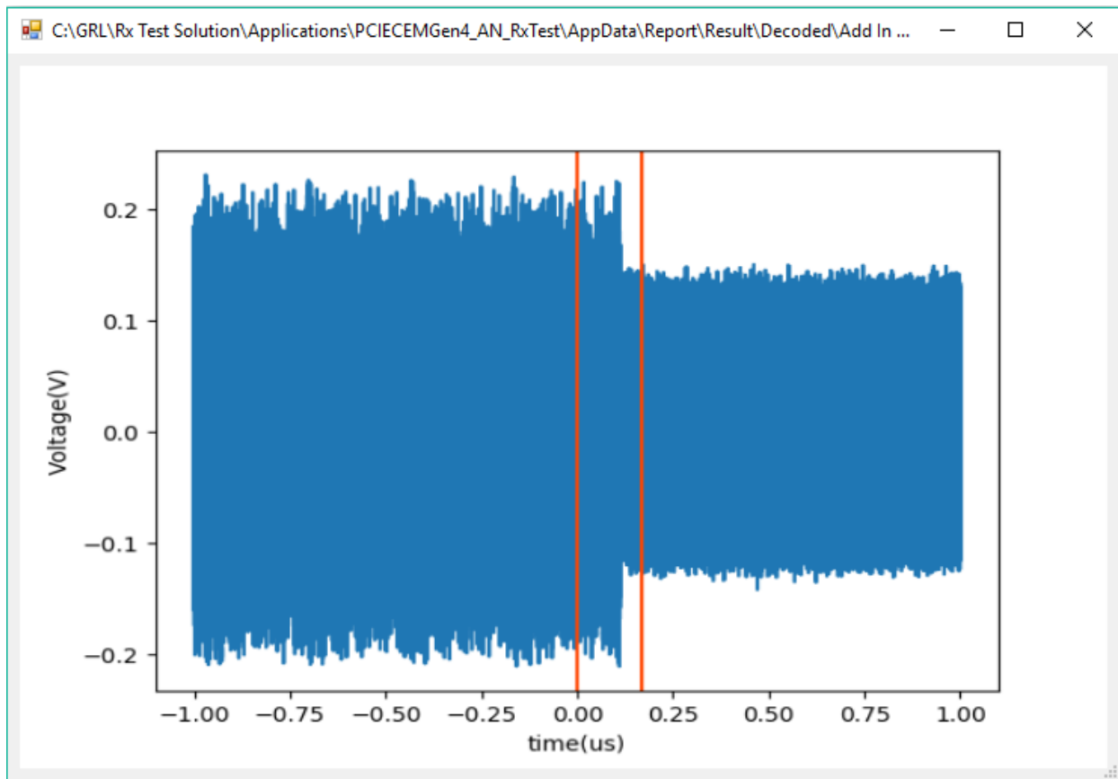
FIGURE 76. VIEWING TX LINK EQ TIME RESPONSE PRESET/CURSOR TEST TRACE FOR TRANSITION TIME
