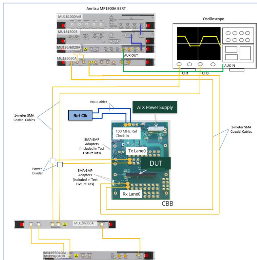
FIGURE 34. RECOMMENDED SETUP FOR DUT TX LINK EQ TESTING (PCIe GEN 3/4 ADD-IN CARD) IN THE IR REFCLK MODE
