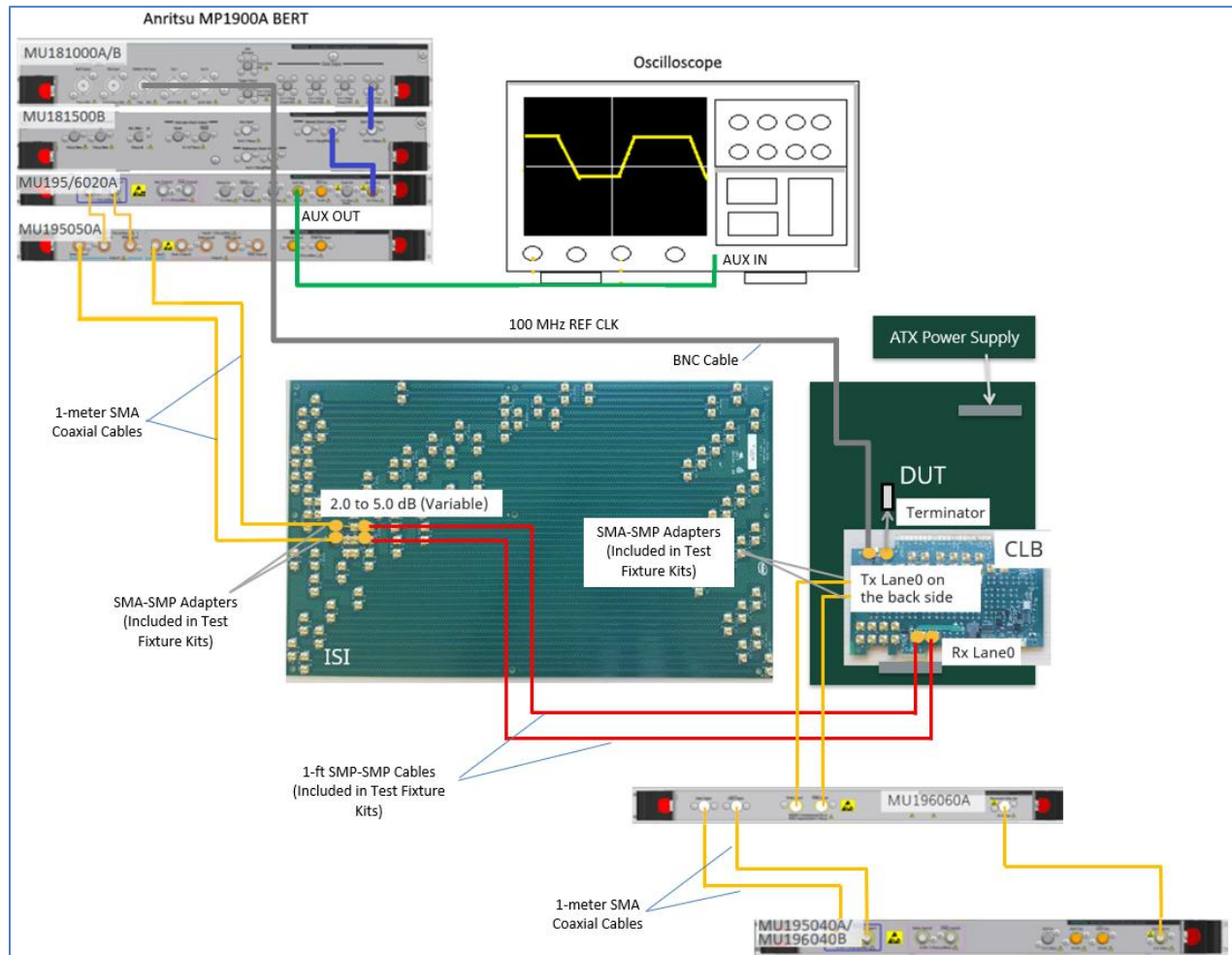
FIGURE 35. RECOMMENDED SETUP FOR DUT RX COMPLIANCE TESTING (PCIe GEN 4 SYSTEM BOARD)
