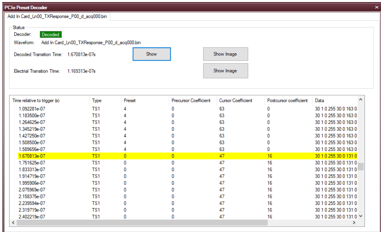
FIGURE 75. VIEWING TX LINK EQ TIME RESPONSE PRESET/CURSOR TEST RESULTS
