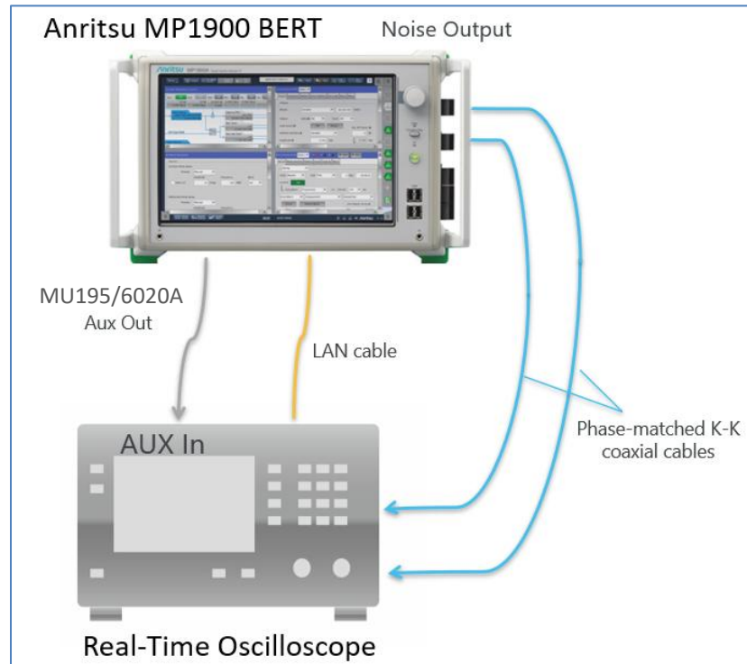
FIGURE 61. CONNECTION DIAGRAM FOR AMPLITUDE, PRESET, SJ AND RJ CALIBRATION
