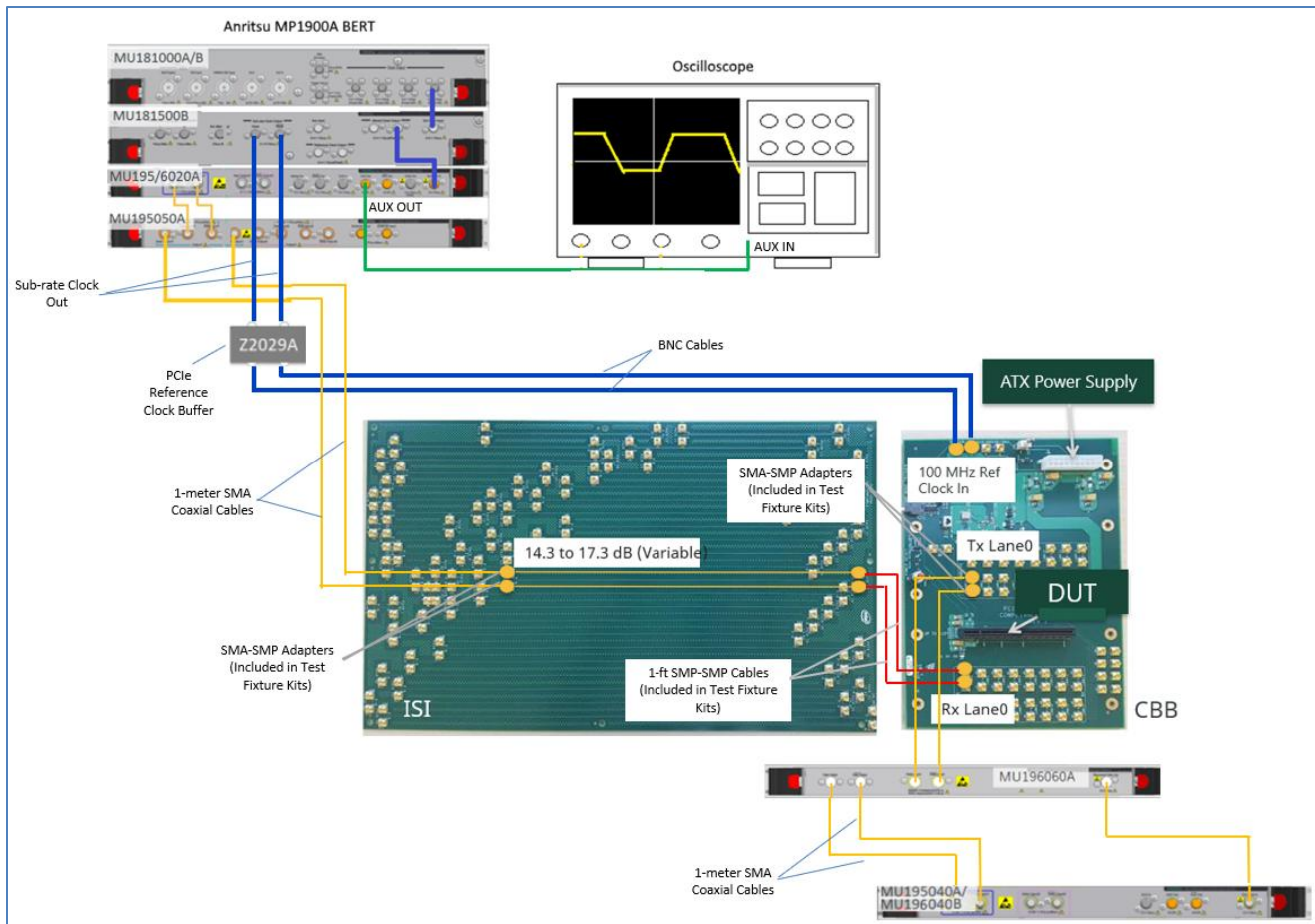
FIGURE 39. RECOMMENDED SETUP FOR DUT RX COMPLIANCE TESTING (PCIe GEN 4 ADD-IN CARD)
