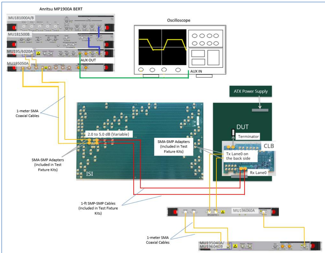
FIGURE 36. RECOMMENDED SETUP FOR DUT RX COMPLIANCE TESTING (PCIe GEN 4 SYSTEM BOARD) IN THE IR REFCLK MODE
