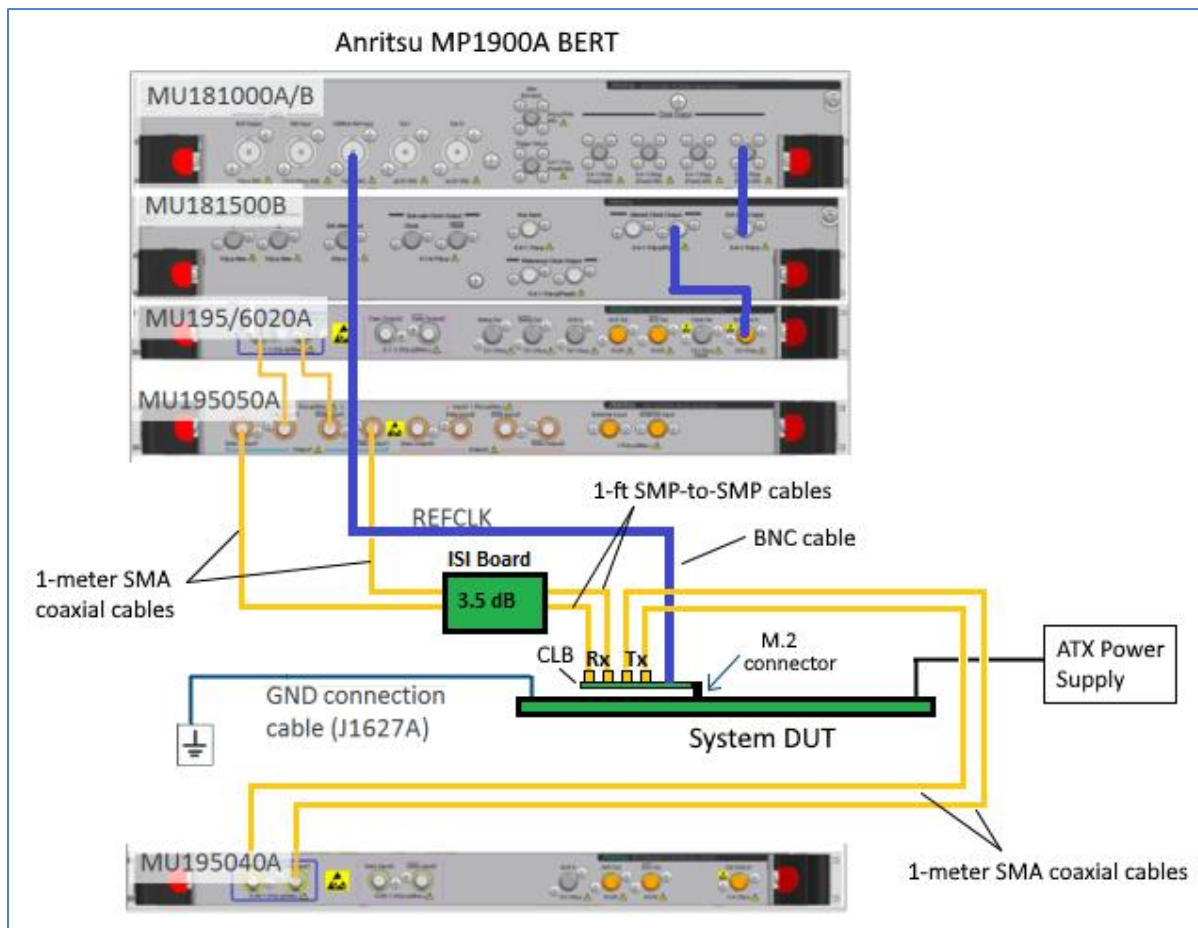
FIGURE 37. RECOMMENDED SETUP FOR DUT M.2 RX COMPLIANCE TESTING (PCIe GEN 3 SYSTEM BOARD)
