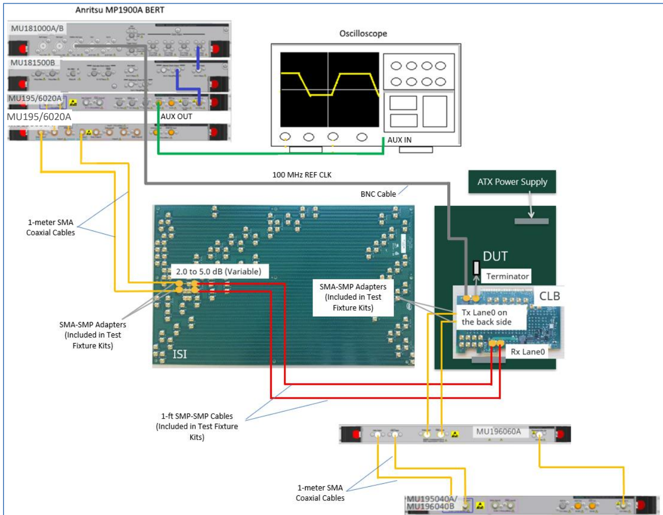
FIGURE 66. CONNECTION DIAGRAM FOR PCIe GEN 4 SYSTEM BOARD DUT LOOPBACK TEST
