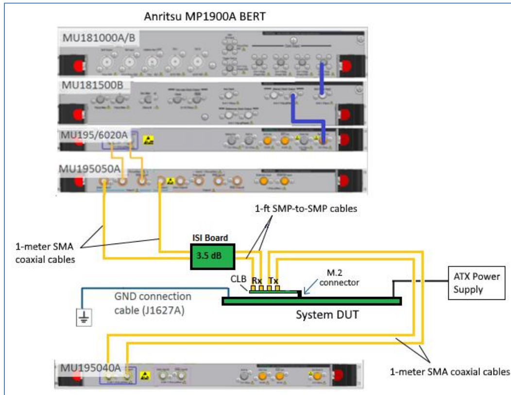
FIGURE 38. RECOMMENDED SETUP FOR DUT M.2 RX COMPLIANCE TESTING (PCIe GEN 3 SYSTEM BOARD) IN THE IR REFCLK MODE
