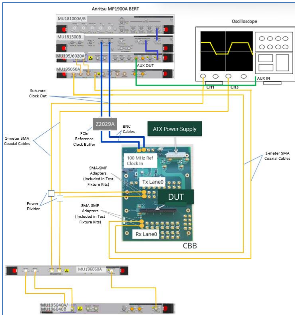
FIGURE 33. RECOMMENDED SETUP FOR DUT TX LINK EQ TESTING (PCI-E GEN 3/4 ADD-IN CARD)
