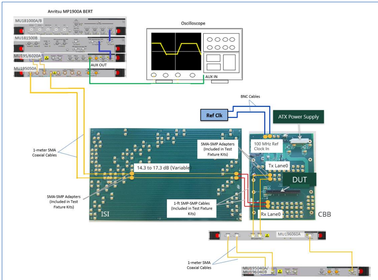
FIGURE 40. RECOMMENDED SETUP FOR DUT RX COMPLIANCE TESTING (PCIe GEN 4 ADD-IN CARD) IN THE IR REFCLK MODE
