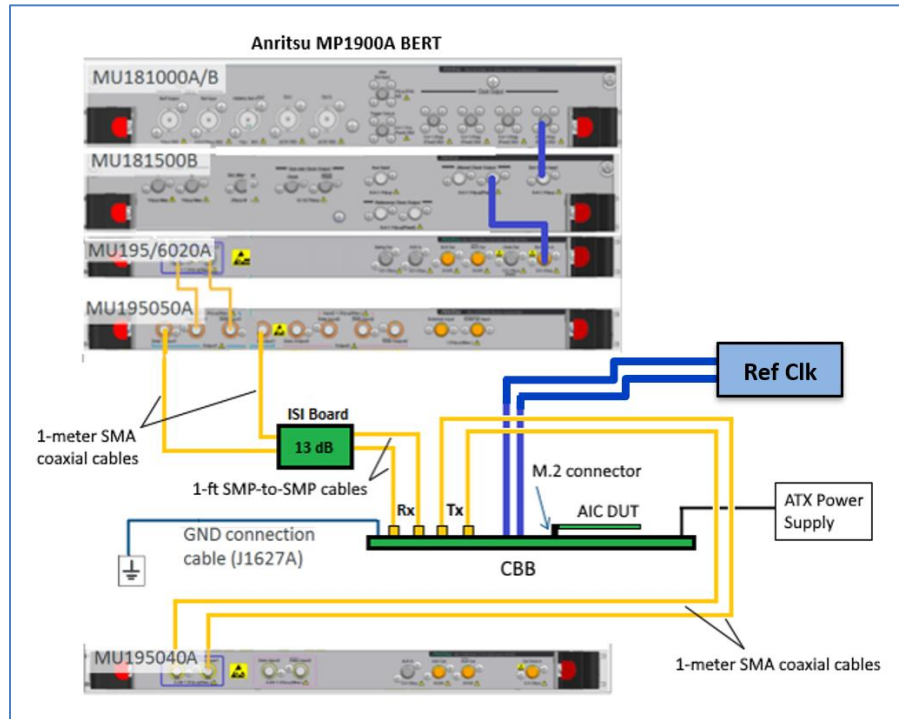
FIGURE 42. RECOMMENDED SETUP FOR DUT M.2 RX COMPLIANCE TESTING (PCIe GEN 3 ADD-IN CARD) IN THE IR REFCLK MODE
