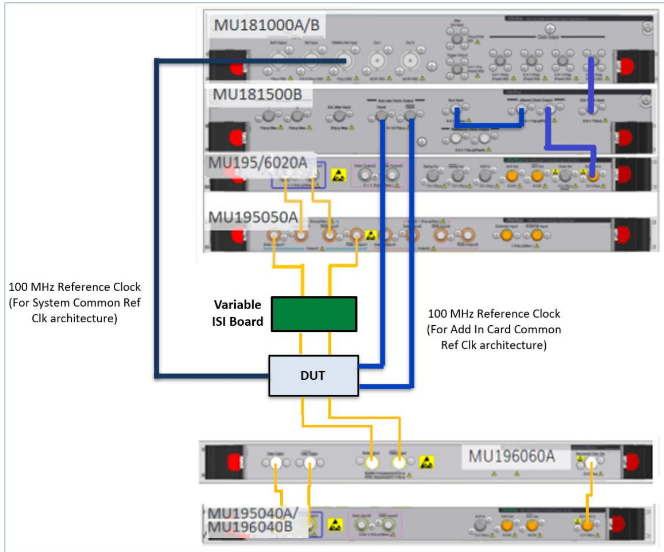
FIGURE 31. TYPICAL RECEIVER DUT TEST SETUP
