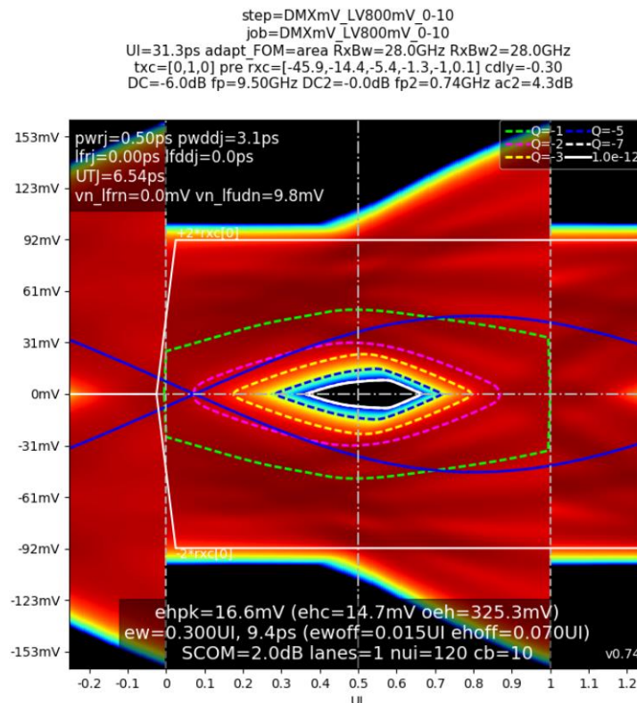
FIGURE 29. FINAL CALIBRATED STRESSED EYE DIAGRAM EXAMPLE
