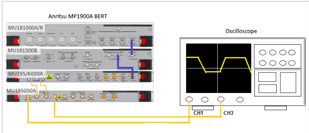
FIGURE 21. TYPICAL SETUP FOR TP1 CALIBRATION
