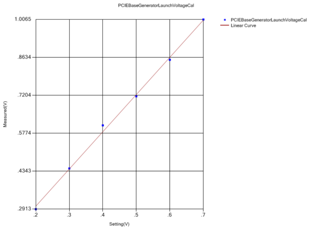
FIGURE 39. CALIBRATION RESULTS EXAMPLE
