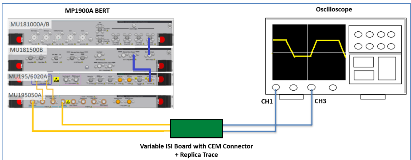
FIGURE 27. TYPICAL SETUP FOR TP2 CALIBRATION
