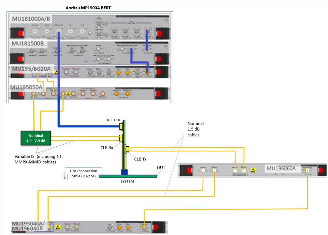
FIGURE 31. RECOMMENDED SETUP FOR DUT RX COMPLIANCE TESTING (PCIe GEN 5 SYSTEM BOARD)
