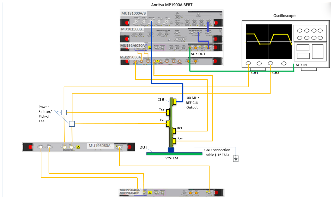
FIGURE 29. RECOMMENDED SETUP FOR DUT TxRx LINK EQ TESTING (PCIe GEN 5 SYSTEM BOARD)
