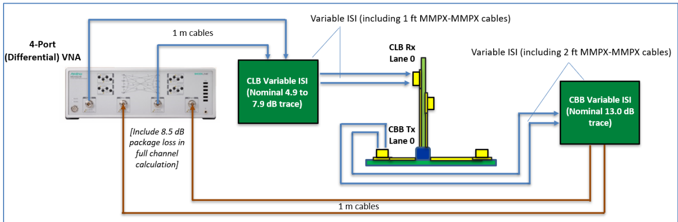
FIGURE 51. CONNECTION DIAGRAM FOR CHANNEL LOSS CALIBRATION (SYSTEM BOARD)
