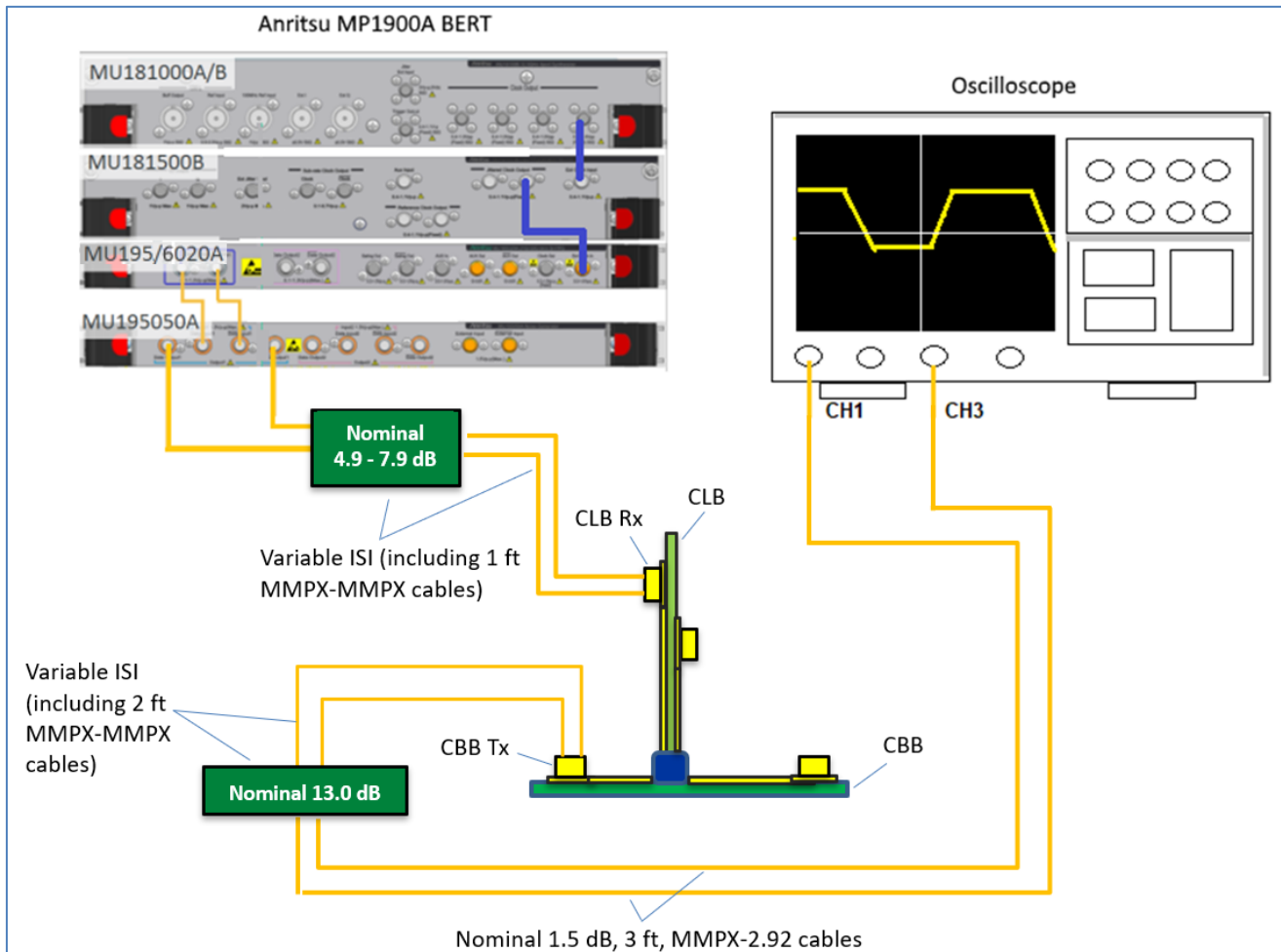
FIGURE 10. RECOMMENDED SETUP FOR TP2 LONG CHANNEL RX CALIBRATION (PCIe GEN 5 SYSTEM BOARD)
