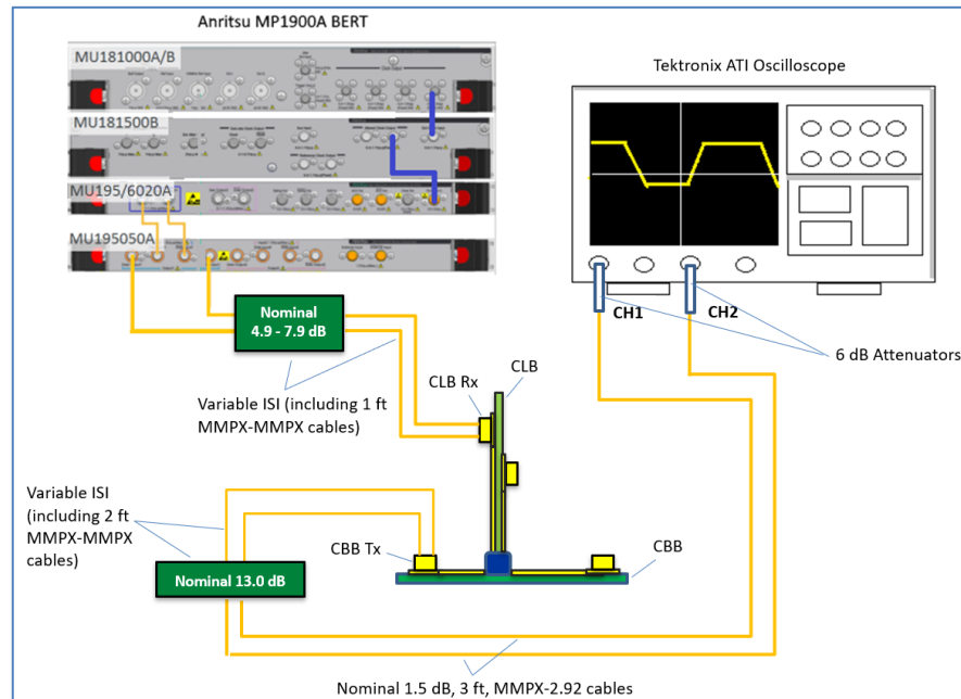
FIGURE 53. CONNECTION DIAGRAM FOR PCIe GEN 5 DM-I, CM-I AND EH/EW TP2 CALIBRATION (FOR SYSTEM BOARD)
