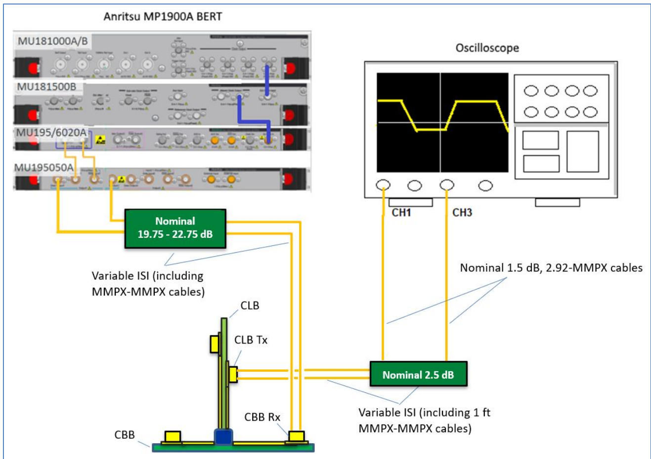
FIGURE 12. RECOMMENDED SETUP FOR TP2 LONG CHANNEL RX CALIBRATION (PCIe GEN 5 ADD-IN CARD)
