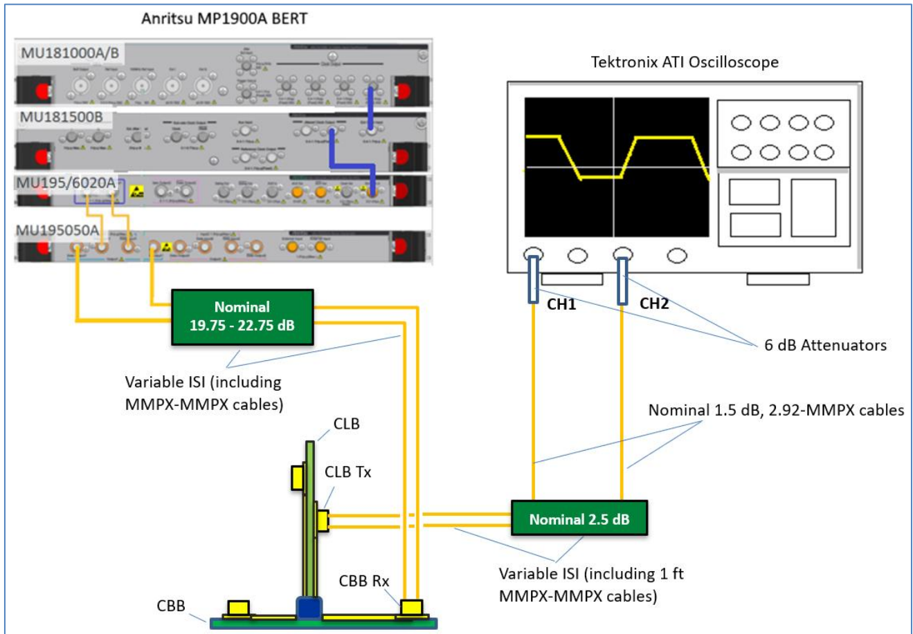
FIGURE 13. RECOMMENDED SETUP FOR TP2 LONG CHANNEL RX CALIBRATION (PCIe GEN 5 ADD-IN CARD) USING TEKTRONIX ATI SCOPE
