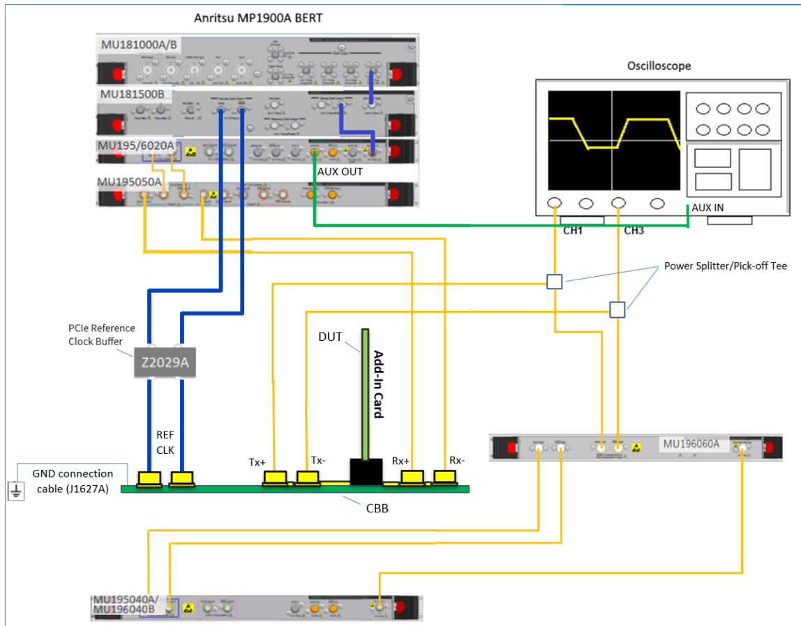
FIGURE 30. RECOMMENDED SETUP FOR DUT TxRx LINK EQ TESTING (PCIe GEN 5 ADD-IN CARD)
