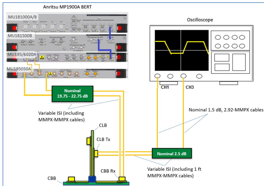
FIGURE 54. CONNECTION DIAGRAM FOR PCIe GEN 5 DM-I, CM-I AND EH/EW TP2 CALIBRATION (FOR ADD-IN CARD)
