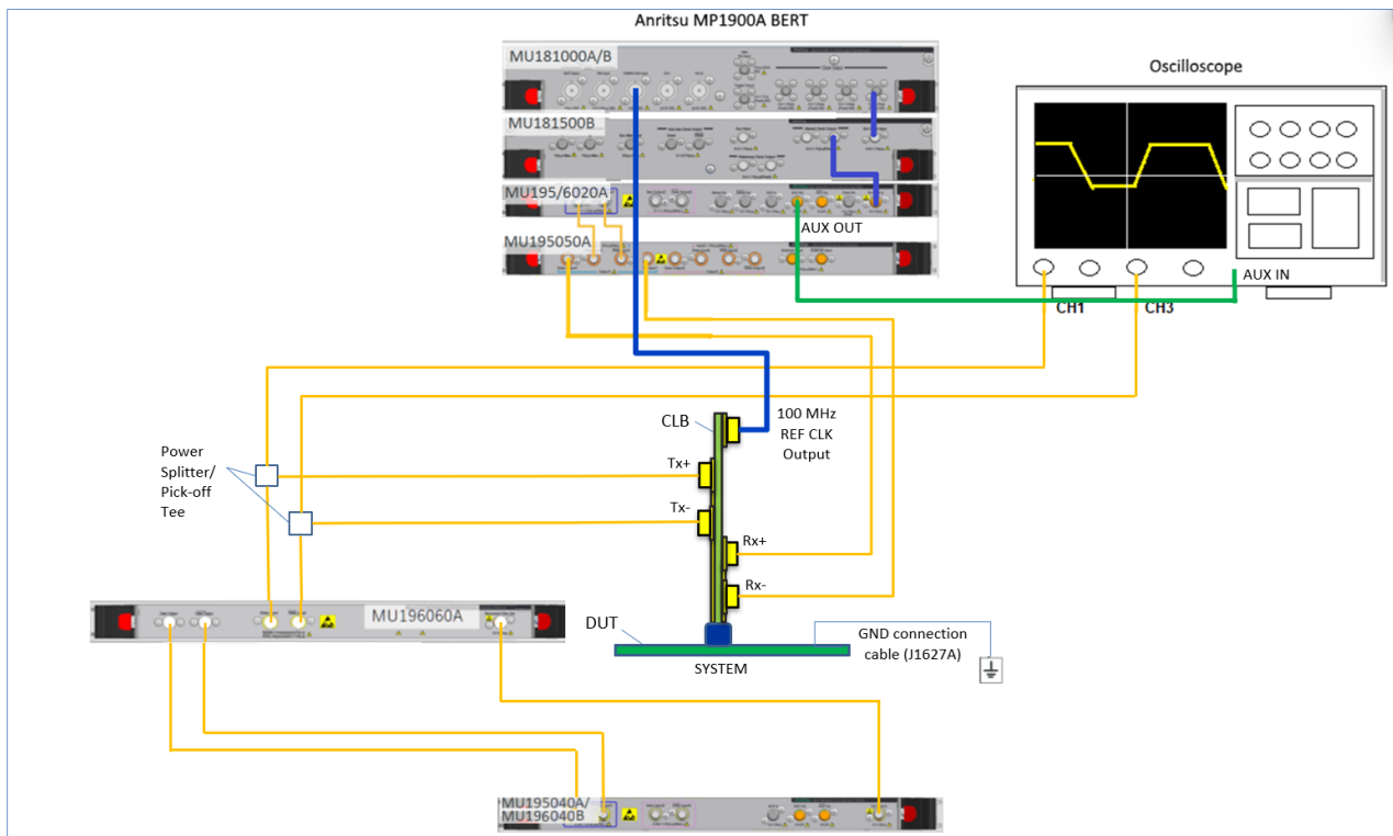
FIGURE 56. CONNECTION DIAGRAM FOR PCIe GEN 5 SYSTEM BOARD DUT TX LINK EQ RESPONSE TEST
