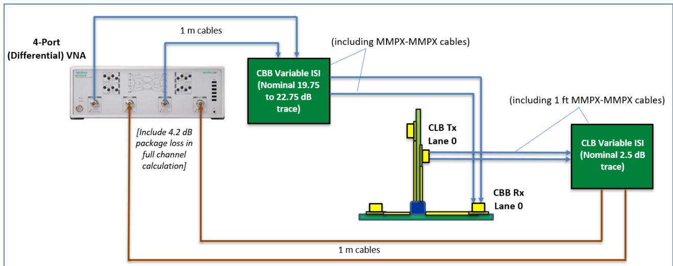
FIGURE 50. CONNECTION DIAGRAM FOR CHANNEL LOSS CALIBRATION (ADD-IN CARD)
