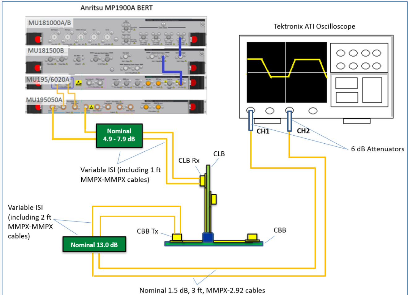
FIGURE 11. RECOMMENDED SETUP FOR TP2 LONG CHANNEL RX CALIBRATION (PCIe GEN 5 SYSTEM BOARD) USING TEKTRONIX ATI SCOPE
