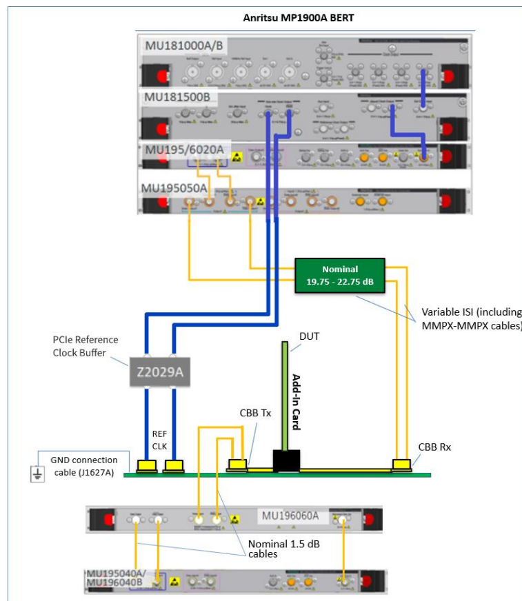
FIGURE 32. RECOMMENDED SETUP FOR DUT RX COMPLIANCE TESTING (PCIe GEN 5 ADD-IN CARD)
