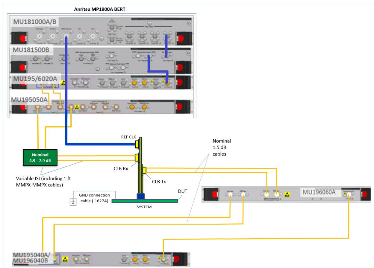
FIGURE 58. CONNECTION DIAGRAM FOR PCIe GEN 5 SYSTEM BOARD DUT LOOPBACK TEST
