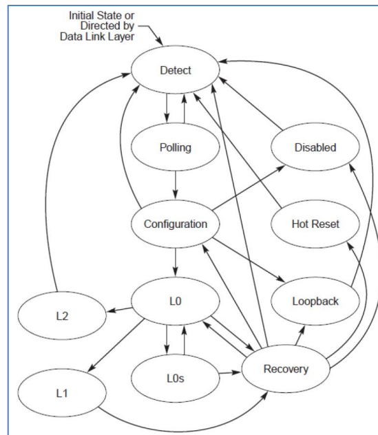
FIGURE 27. MAIN STATE DIAGRAM FOR LINK TRAINING AND STATUS STATE MACHINE (FROM PHY TEST SPECIFICATION)
