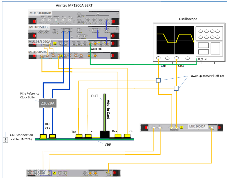
FIGURE 55. CONNECTION DIAGRAM FOR PCIe GEN 5 ADD-IN CARD DUT INITIAL TX EQ / TX LINK EQ RESPONSE TEST
