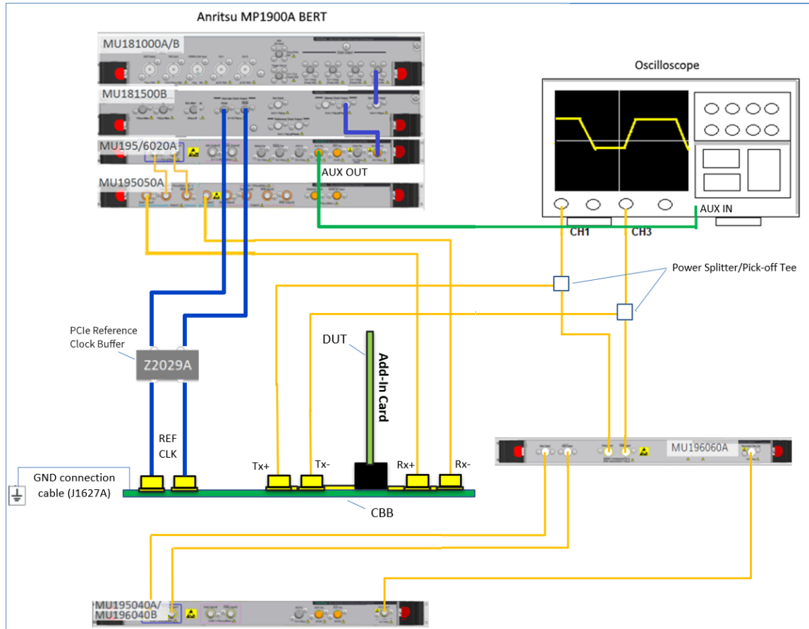
FIGURE 31. RECOMMENDED SETUP FOR DUT TXRX LINK EQ TESTING (PCIe GEN 5 ADD-IN CARD)
