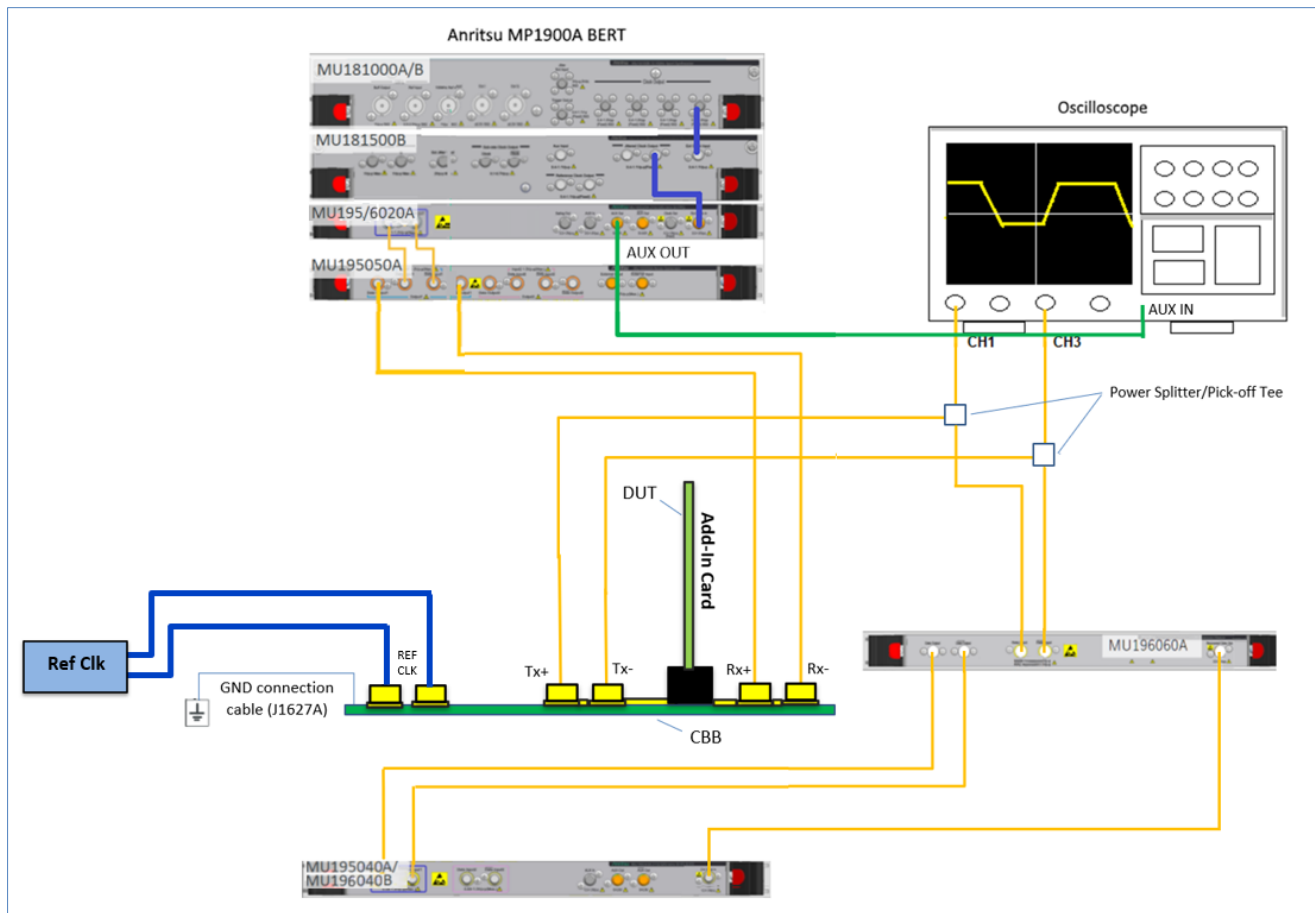
FIGURE 32. RECOMMENDED SETUP FOR DUT TxRx LINK EQ TESTING (PCIe GEN 5 ADD-IN CARD) IN THE IR REFCLK MODE
