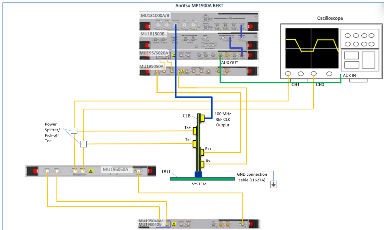
FIGURE 60. CONNECTION DIAGRAM FOR PCIe GEN 5 SYSTEM BOARD DUT TX LINK EQ RESPONSE TEST
