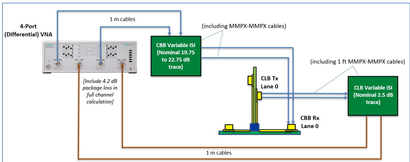
FIGURE 54. CONNECTION DIAGRAM FOR CHANNEL LOSS CALIBRATION (ADD-IN CARD)
