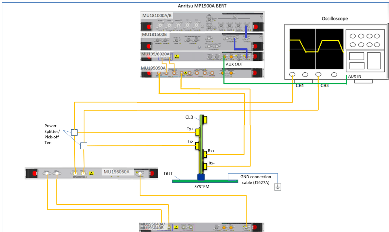
FIGURE 30. RECOMMENDED SETUP FOR DUT TXRX LINK EQ TESTING (PCIe GEN 5 SYSTEM BOARD) IN THE IR REFCLK MODE
