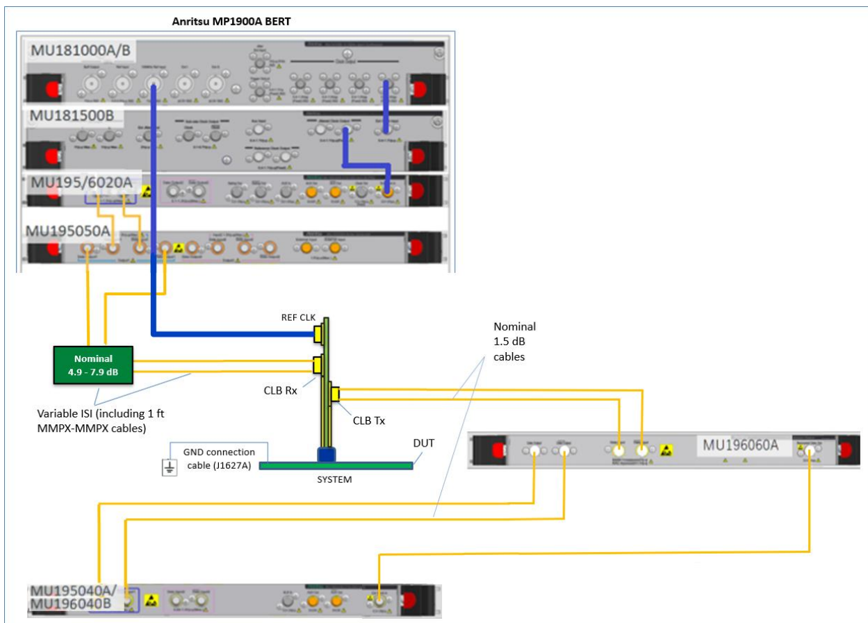
FIGURE 62. CONNECTION DIAGRAM FOR PCIe GEN 5 SYSTEM BOARD DUT LOOPBACK TEST
