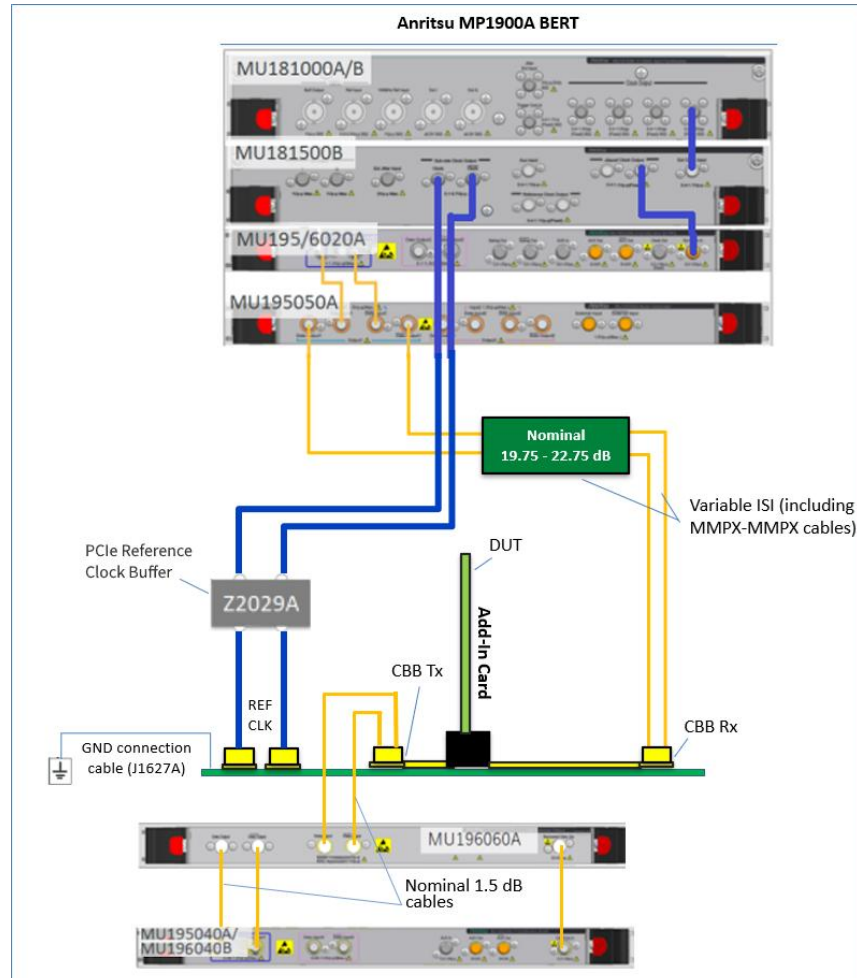
FIGURE 35. RECOMMENDED SETUP FOR DUT RX COMPLIANCE TESTING (PCIe GEN 5 ADD-IN CARD)
