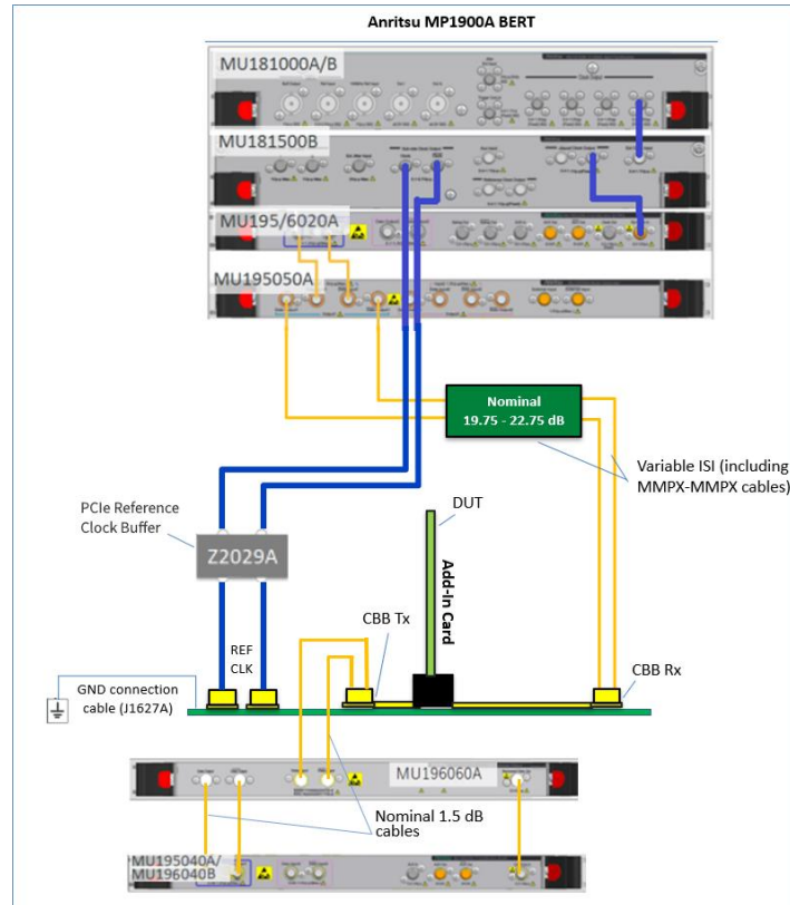
FIGURE 61. CONNECTION DIAGRAM FOR PCIe GEN 5 ADD-IN CARD DUT LOOPBACK TEST
