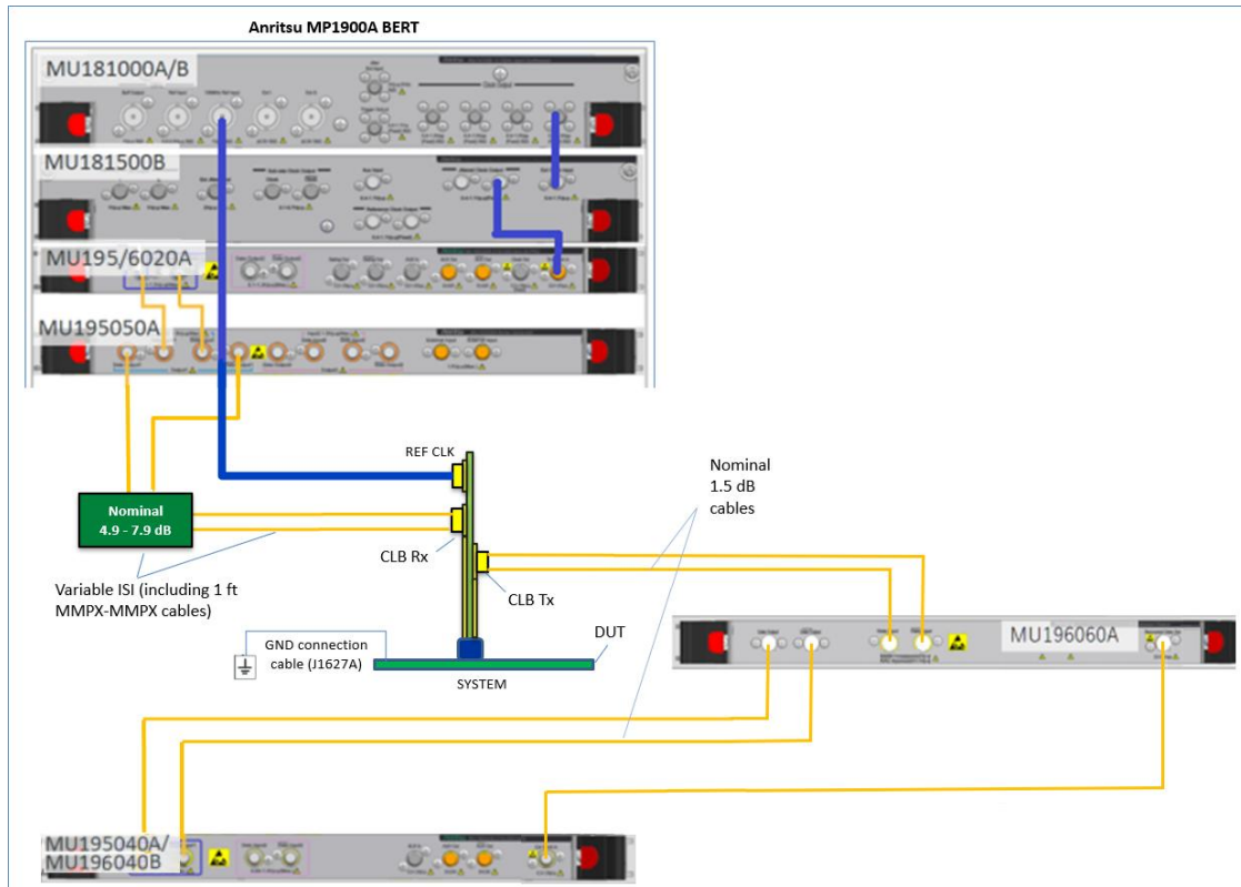
FIGURE 33. RECOMMENDED SETUP FOR DUT RX COMPLIANCE TESTING (PCIe GEN 5 SYSTEM BOARD)
