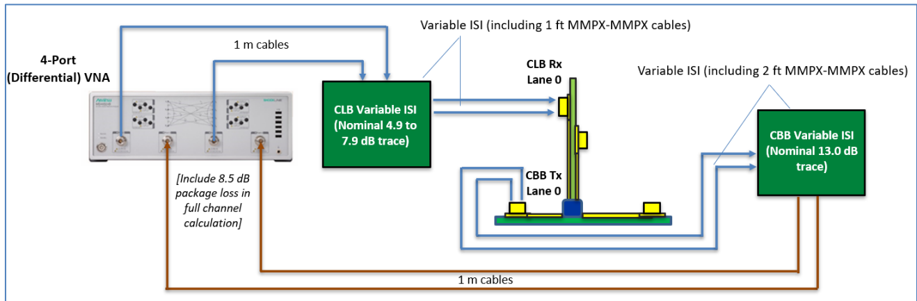
FIGURE 55. CONNECTION DIAGRAM FOR CHANNEL LOSS CALIBRATION (SYSTEM BOARD)
