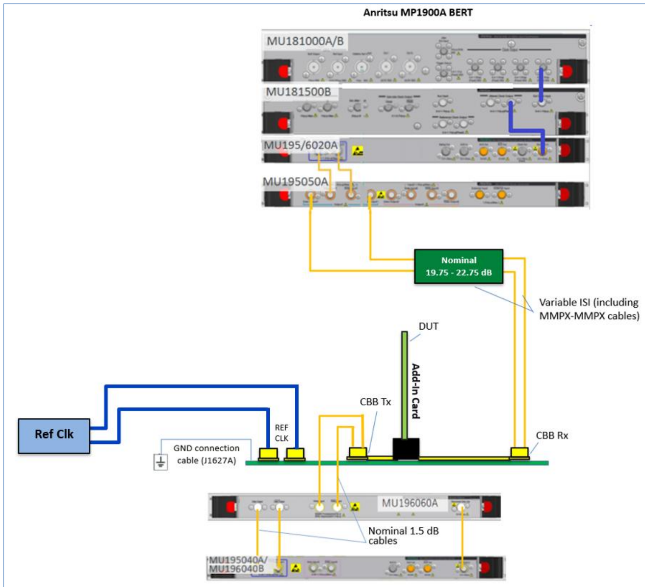
FIGURE 36. RECOMMENDED SETUP FOR DUT RX COMPLIANCE TESTING (PCIe GEN 5 ADD-IN CARD) IN THE IR REFCLK MODE
