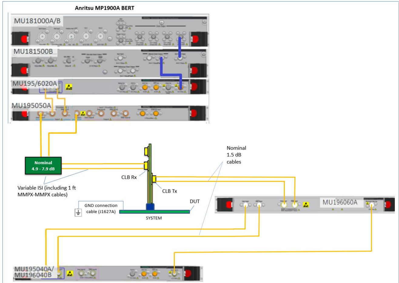
FIGURE 34. RECOMMENDED SETUP FOR DUT RX COMPLIANCE TESTING (PCIe GEN 5 SYSTEM BOARD) IN THE IR REFCLK MODE
