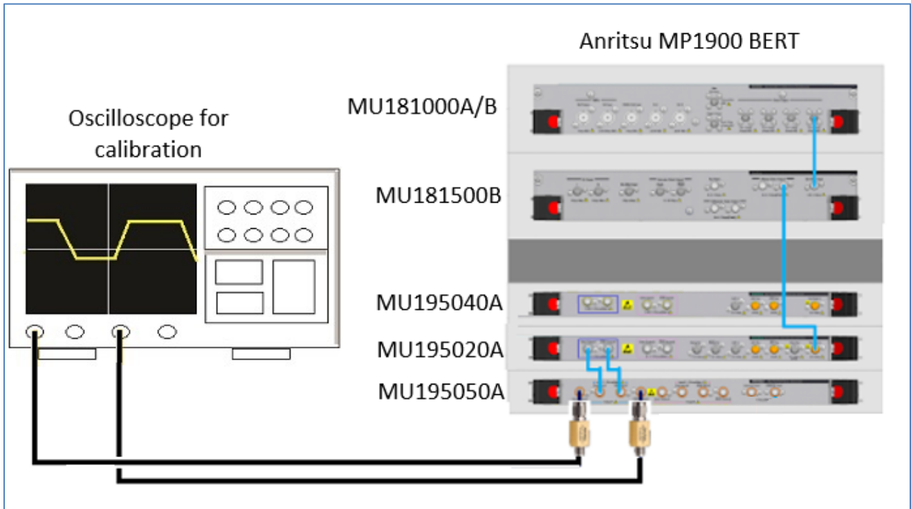
FIGURE 9. SIGNAL AMPLITUDE AND JITTER CALIBRATION SETUP
