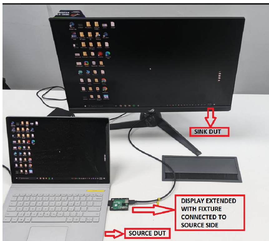
FIGURE 3.8: DISPLAY EXTENDED WITH GRL-C2-DP-AUX-SNIF BOARD TEST FIXTURE CONNECTED TO THE SOURCE SIDE
