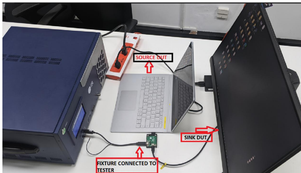
FIGURE 3.9: DISPLAY EXTENDED WITH GRL-C2-DP-AUX-SNIF BOARD TEST FIXTURE CONNECTED TO THE SOURCE SIDE AND GRL-USB-PD-C2-EPR TEST CONTROLLER USING GRL-SPL-EPR CABLE
