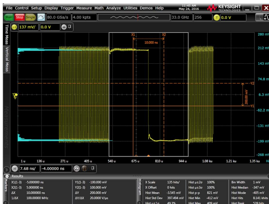
FIGURE 44. OSCILLOSCOPE SETUP FOR AMPLITUDE AND DE-EMPHASIS
