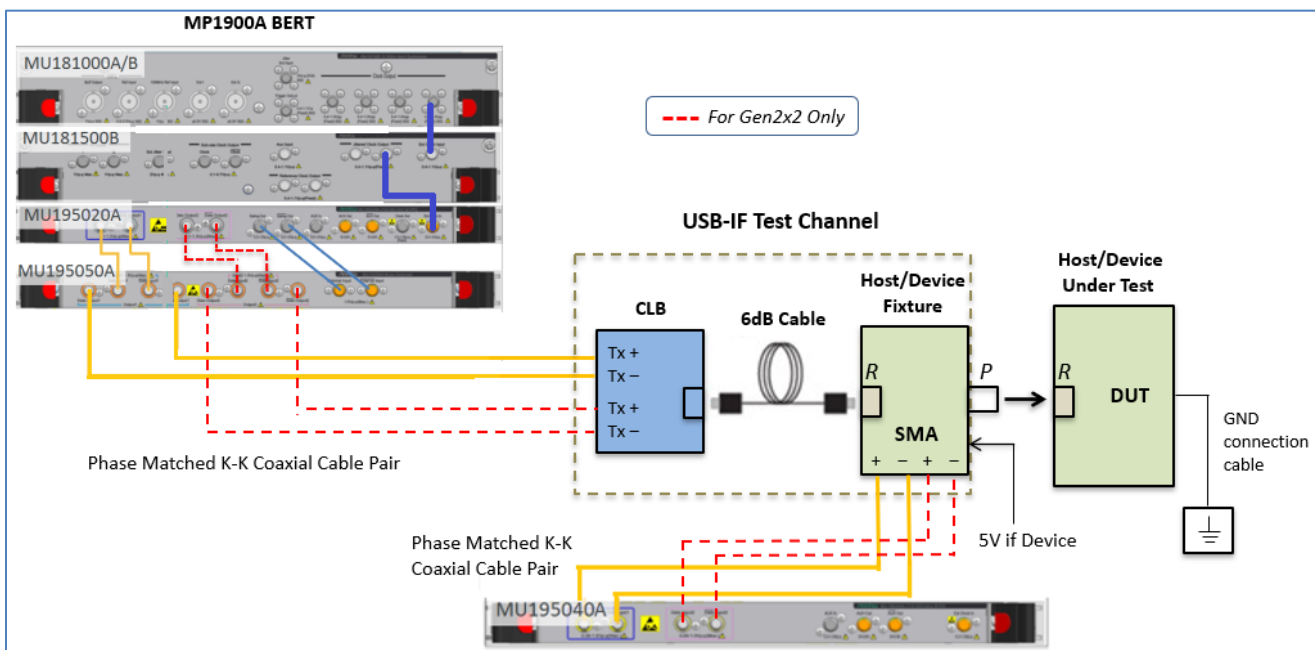
FIGURE 30. TEST SETUP FOR 10GT/S (ALL CONNECTOR TYPES)
