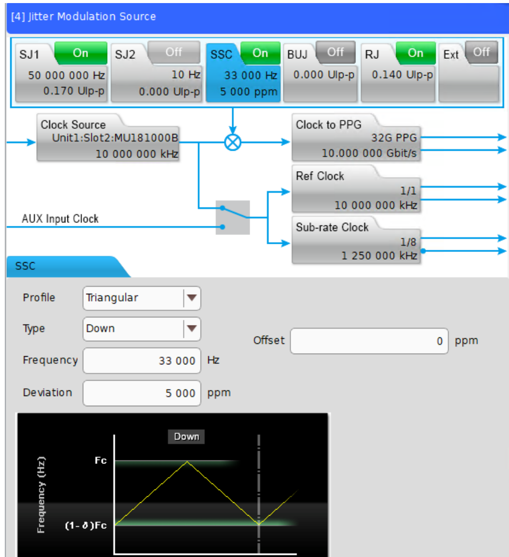
FIGURE 51. SSC SETUP
