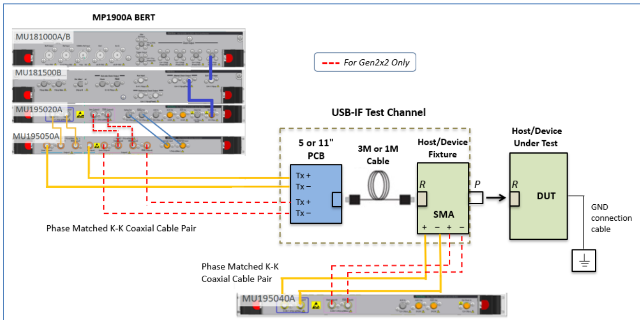
FIGURE 28. TEST SETUP FOR 5GT/S USB TYPE-A OR USB TYPE-B MICRO
