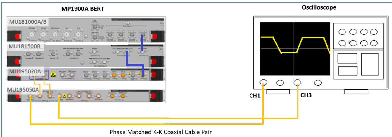
FIGURE 12. CALIBRATION SETUP FOR SWING AND DE-EMPHASIS
