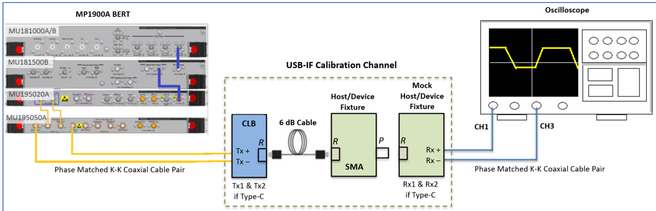
FIGURE 15. CALIBRATION SETUP FOR 10GT/S (ALL CONNECTOR TYPES) USING MP1900A BERT
