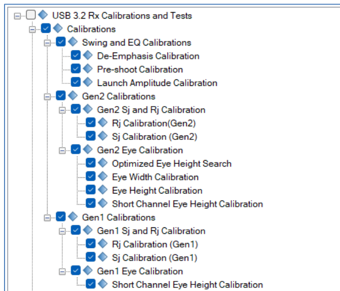
FIGURE 21. SELECT CALIBRATION
