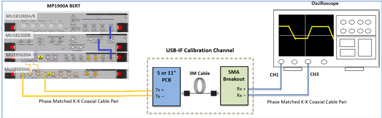
FIGURE 13. CALIBRATION SETUP FOR 5GT/S USB TYPE-A OR USB TYPE-B MICRO
