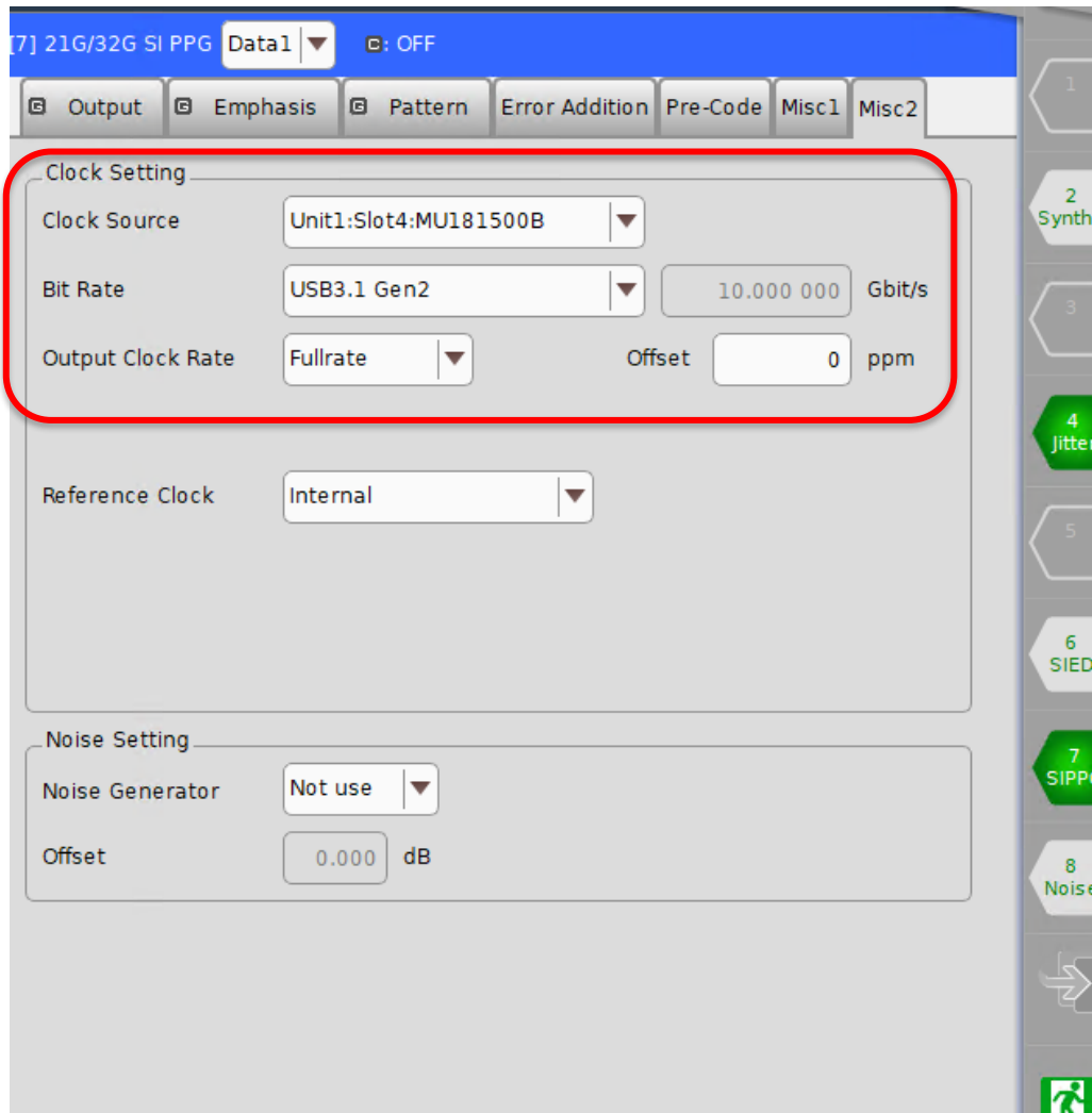
FIGURE 49. CLOCK SETTING
