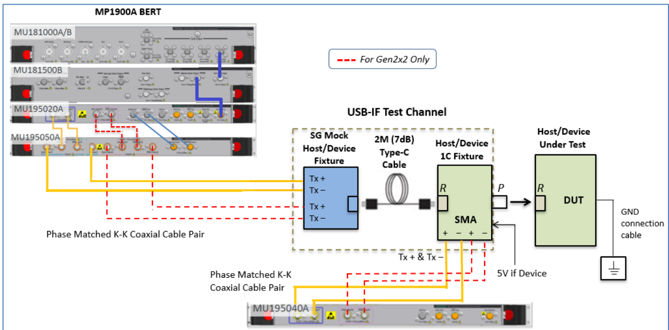
FIGURE 29. TEST SETUP FOR 5GT/S USB TYPE-C
