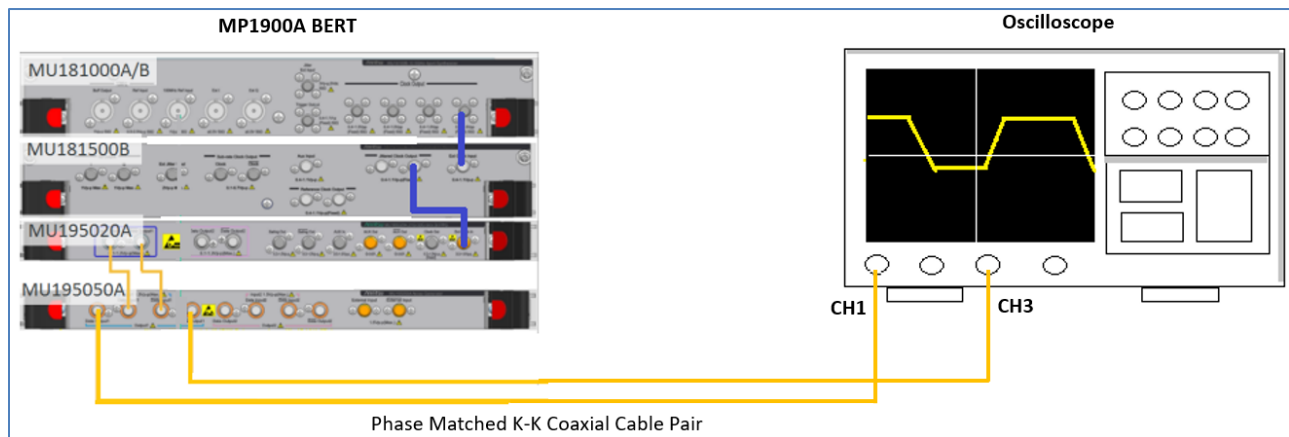
FIGURE 14. CALIBRATION SETUP FOR 5GT/S USB TYPE-C
