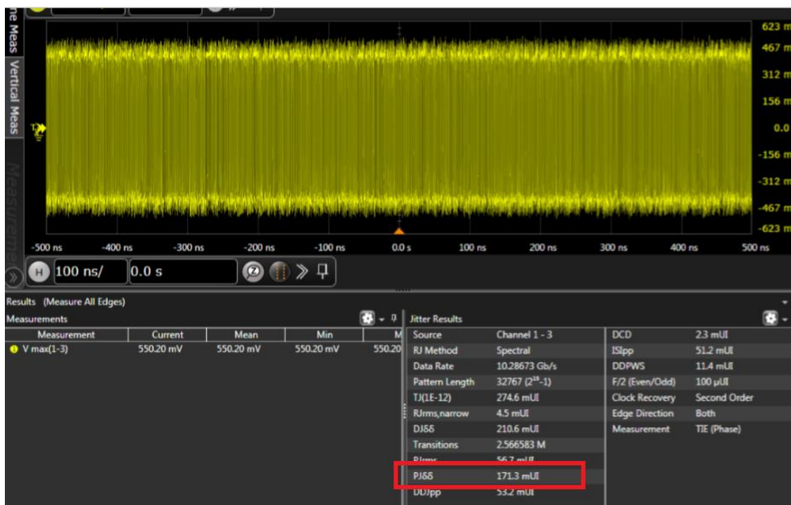
FIGURE 64. CALIBRATE SJ AMPLITUDE #2 ON KEYSIGHT SCOPE
