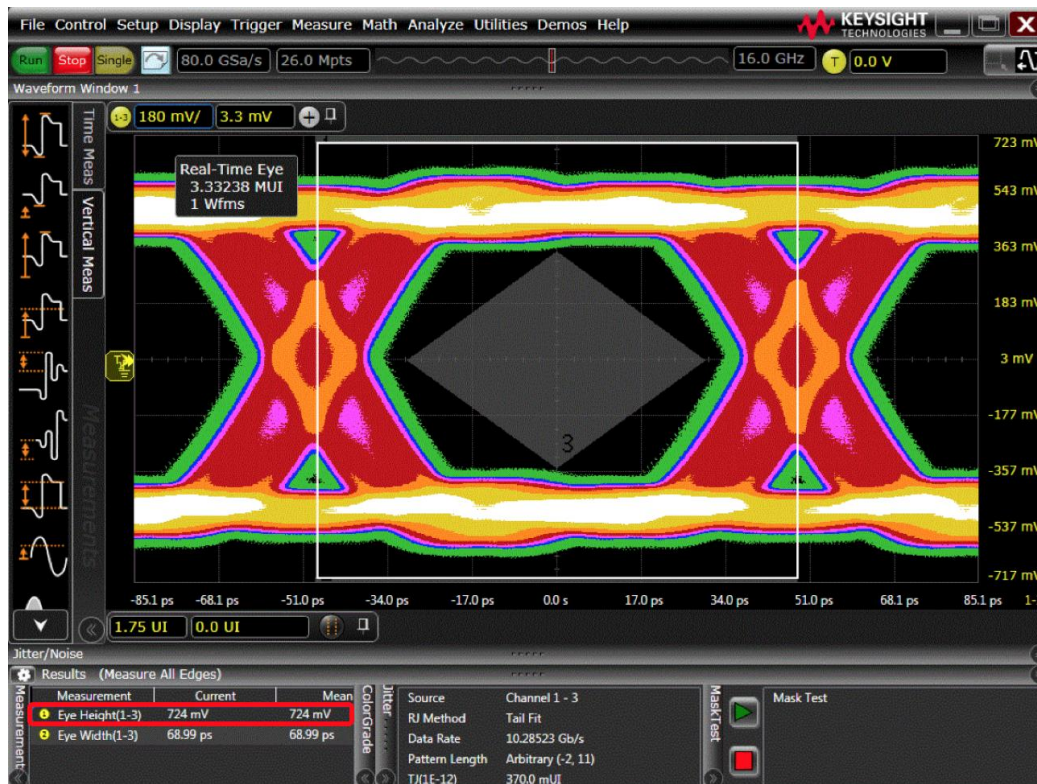
FIGURE 69. EYE MASK ON KEYSIGHT SCOPE
