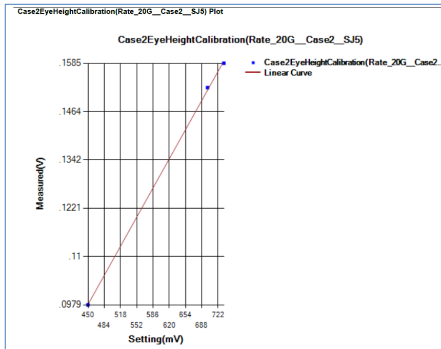
FIGURE 37. CALIBRATION/TEST RESULT DETAILS EXAMPLE
