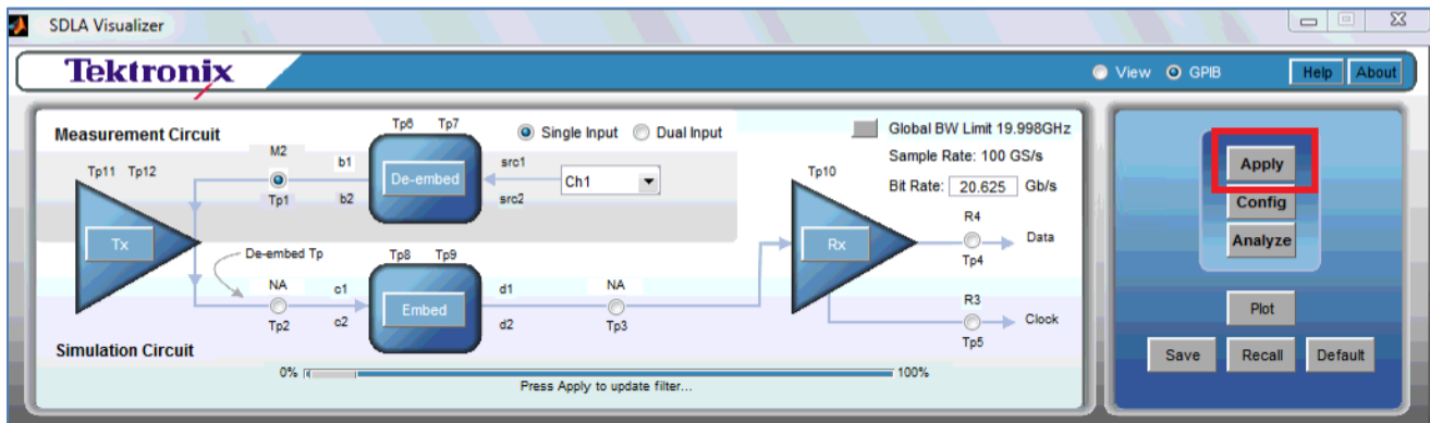
FIGURE 100. CREATE SMA CABLE DE-EMBEDDING FILES – #6
