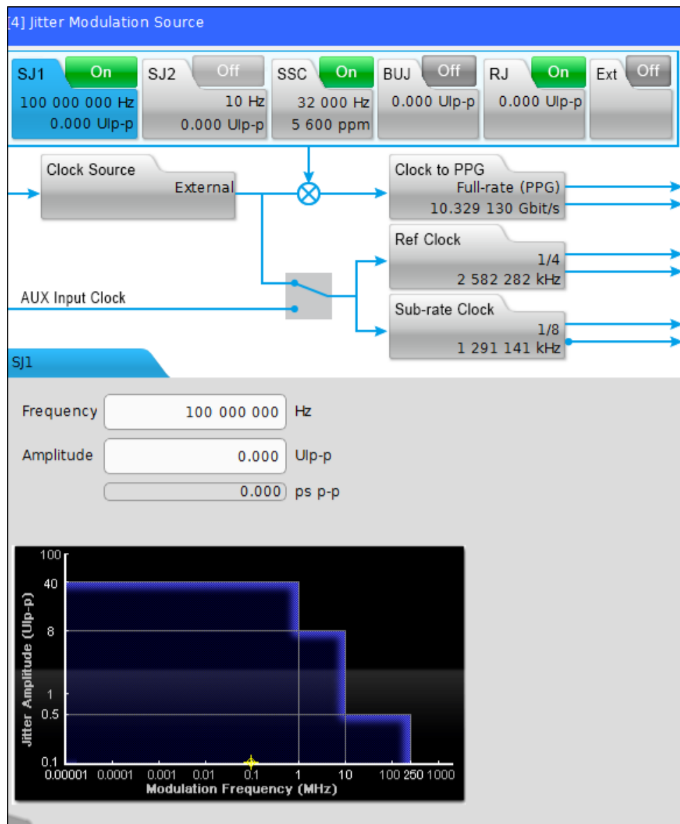
FIGURE 59. JITTER AMPLITUDES
