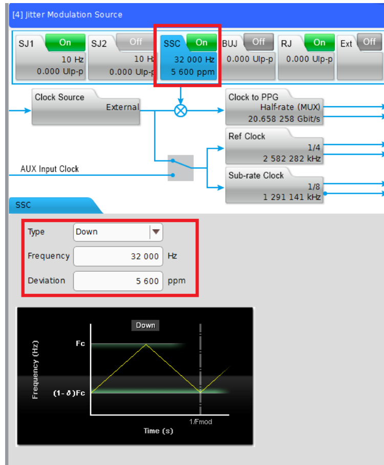
FIGURE 44. PPG EMPHASIS SETTING
