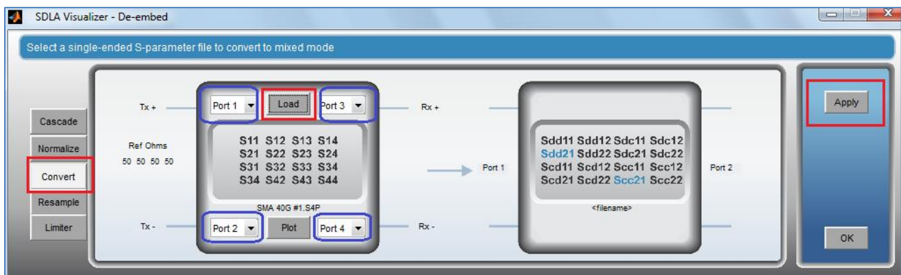
FIGURE 93. CONVERT TO MIXED MODE S-PARAMETERS
