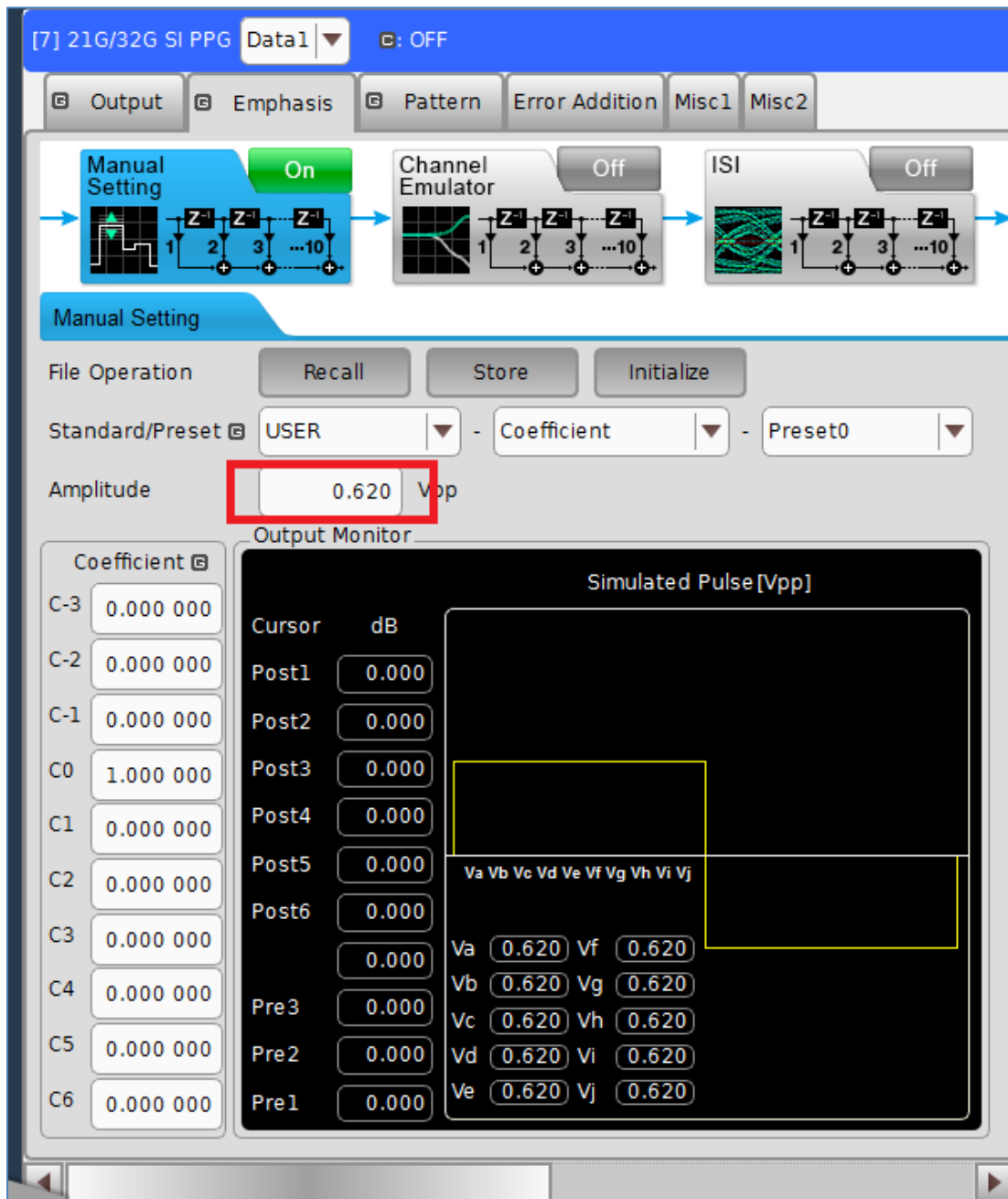
FIGURE 73. EYE AMPLITUDE
