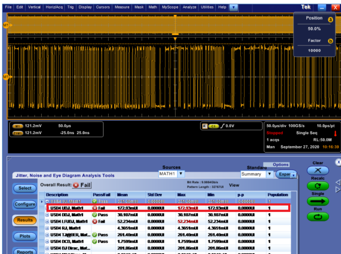
FIGURE 65. CALIBRATE SJ AMPLITUDE #2 ON TEKTRONIX SCOPE
