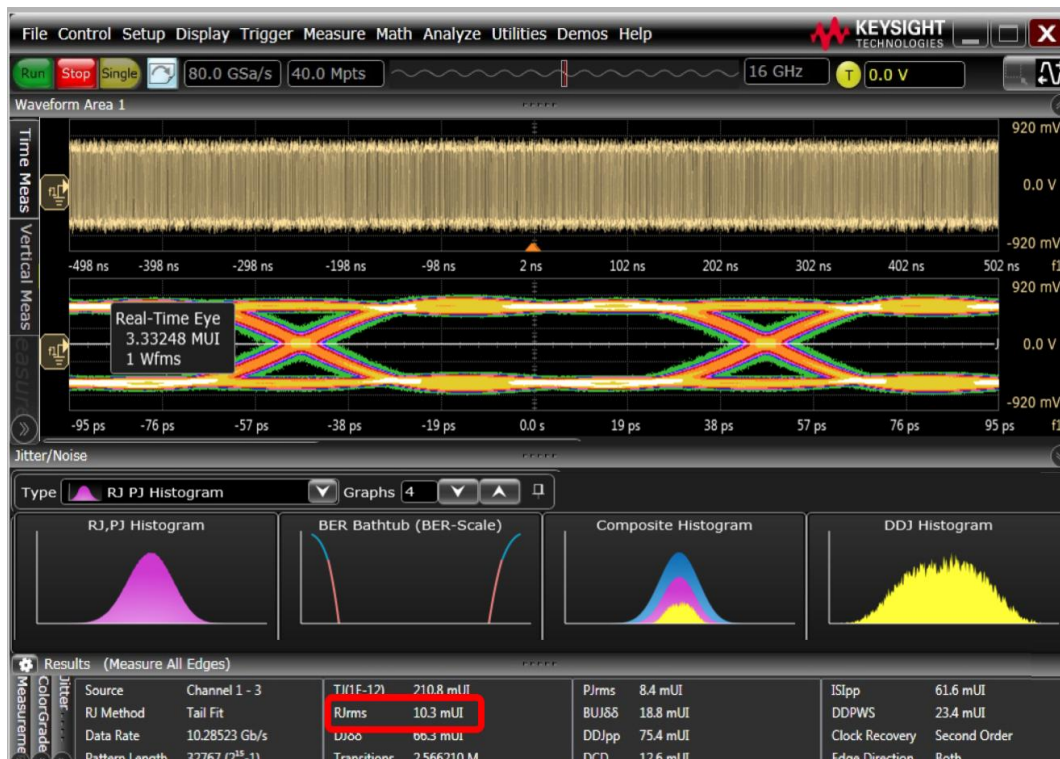
FIGURE 61. CALIBRATE RJ AMPLITUDE #2 ON KEYSIGHT SCOPE
