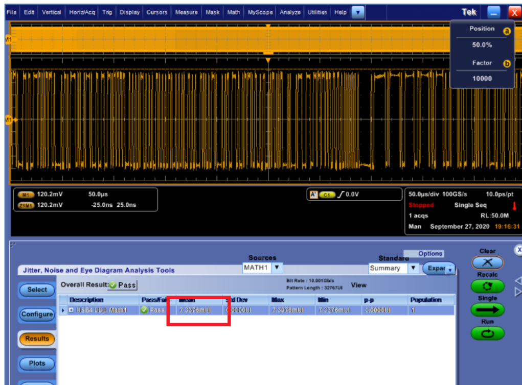
FIGURE 54. OPTIMIZED PRESET (MINIMUM DDJPP) MEASUREMENT ON TEKTRONIX SCOPE
