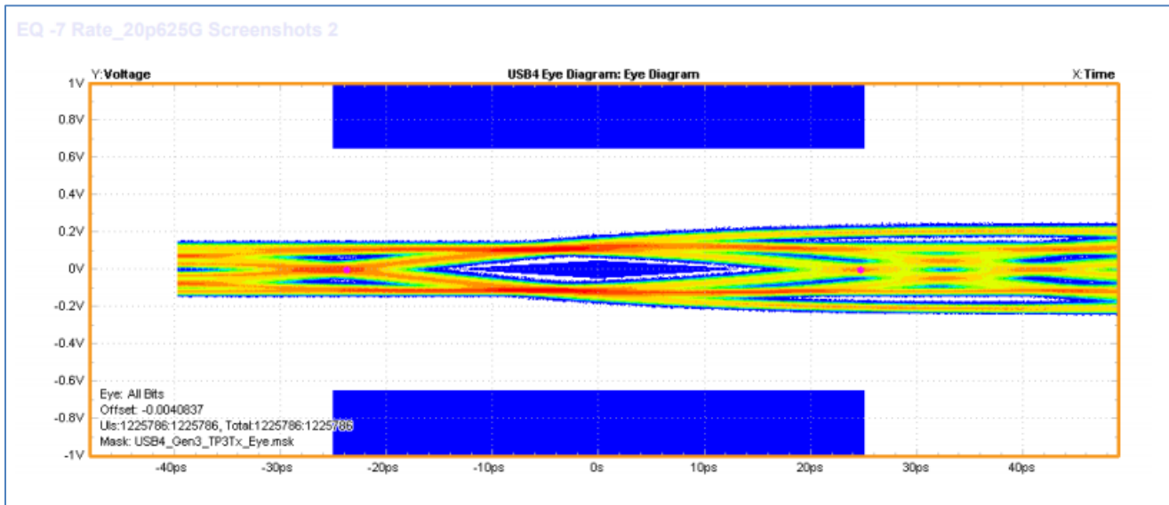
FIGURE 74. EYE AMPLITUDE MEASUREMENTS
