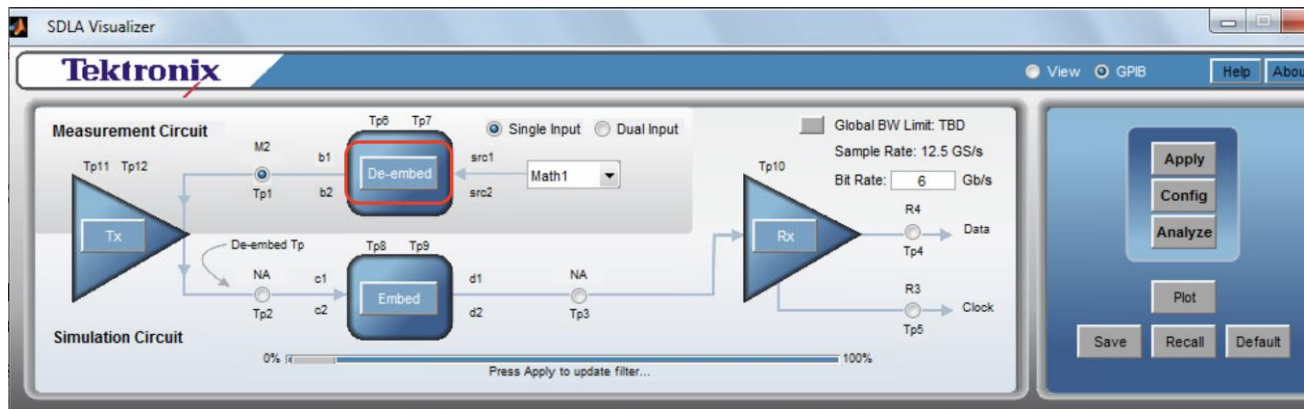
FIGURE 95. CREATE SMA CABLE DE-EMBEDDING FILES – #1
