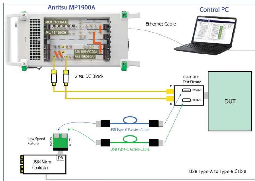
FIGURE 25. Rx BER TEST SETUP AT TP3' (USING USB4 MICROCONTROLLER)
