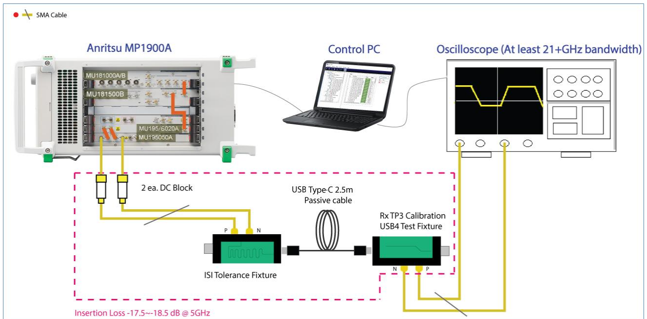
FIGURE 11. SETUP FOR TP3 (CASE 2) CALIBRATION AT 10G OR 10.3125G
