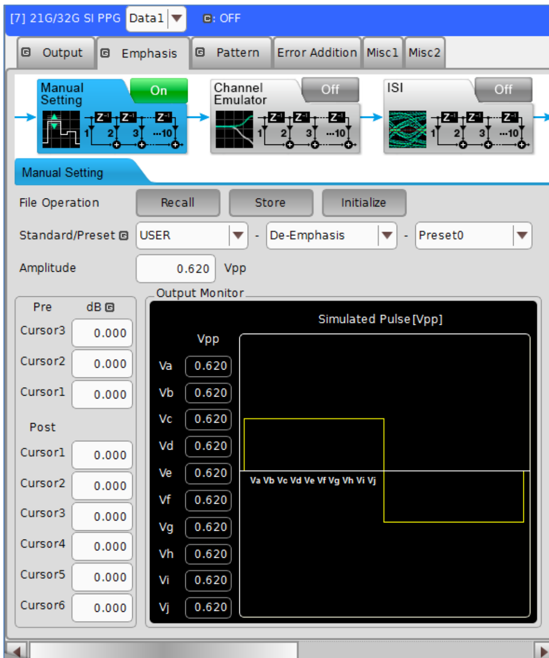
FIGURE 82. EYE AMPLITUDE
