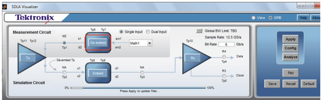
FIGURE 100. CREATE SMA CABLE DE-EMBEDDING FILES – #1
