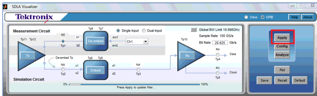
FIGURE 105. CREATE SMA CABLE DE-EMBEDDING FILES – #6
