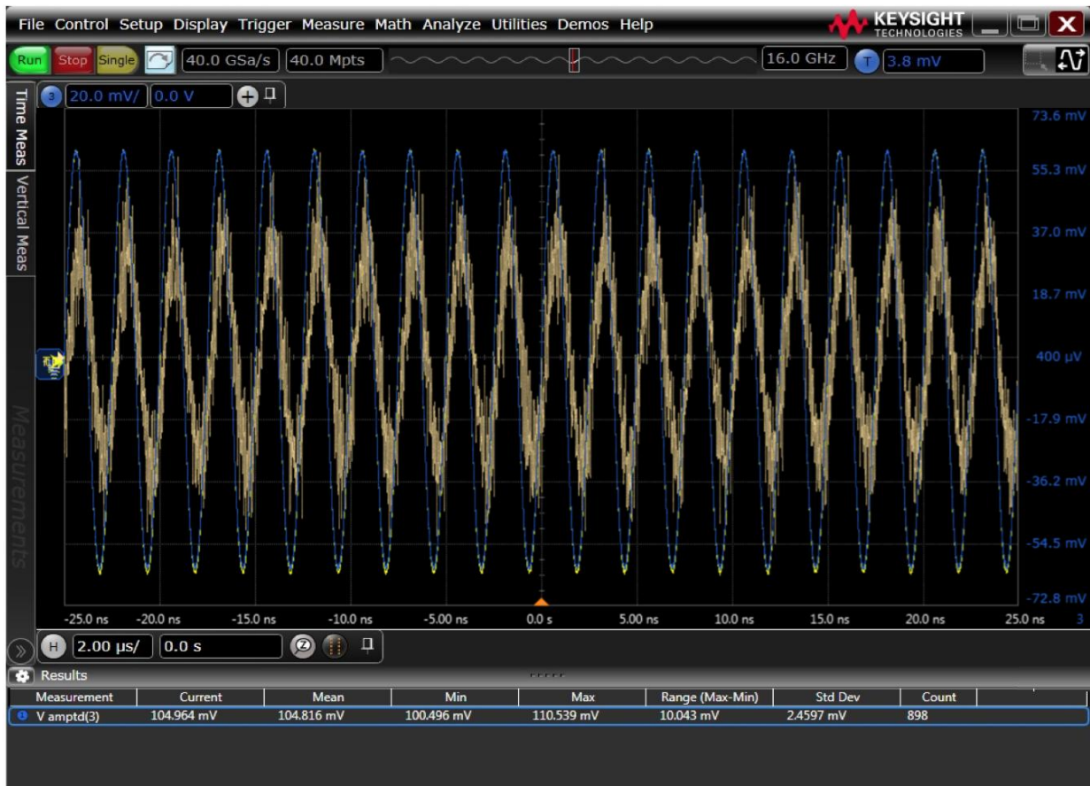
FIGURE 63. CALIBRATE ACCM PEAK-TO-PEAK AMPLITUDE
