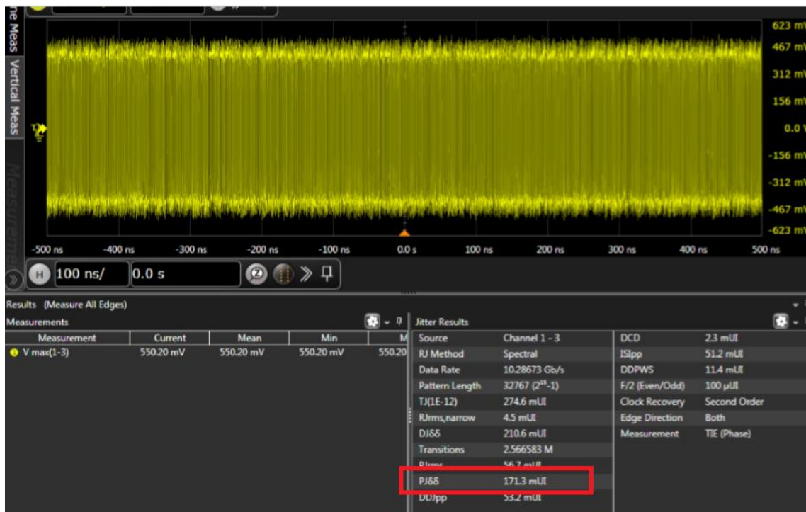
FIGURE 69. CALIBRATE SJ AMPLITUDE #2 ON KEYSIGHT SCOPE
