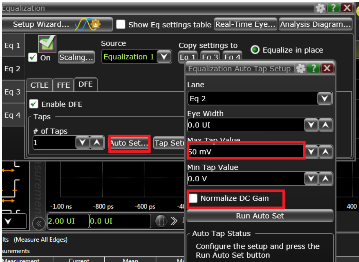
FIGURE 81. DFE SETTING
