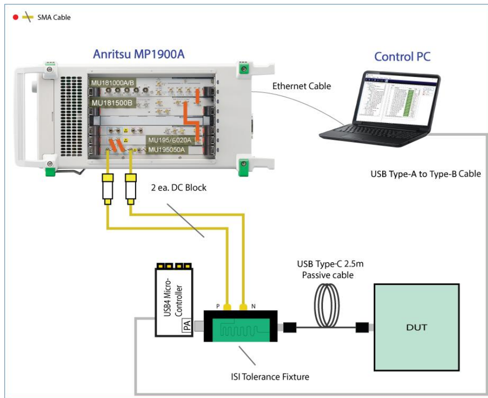
FIGURE 26. SETUP FOR TP3 Rx BER TEST AT 10G OR 10.3125G (USING USB4 MICROCONTROLLER)
