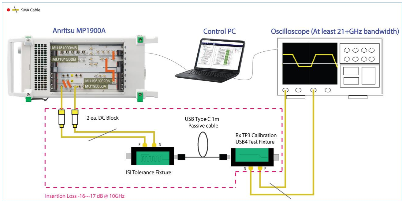
FIGURE 12. SETUP FOR TP3 (CASE 2) CALIBRATION AT 20G OR 20.625G
