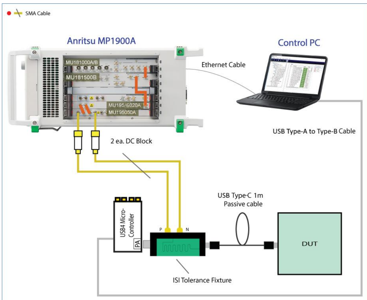
FIGURE 27. SETUP FOR TP3 Rx BER TEST AT 20G OR 20.625G (USING USB4 MICROCONTROLLER)
