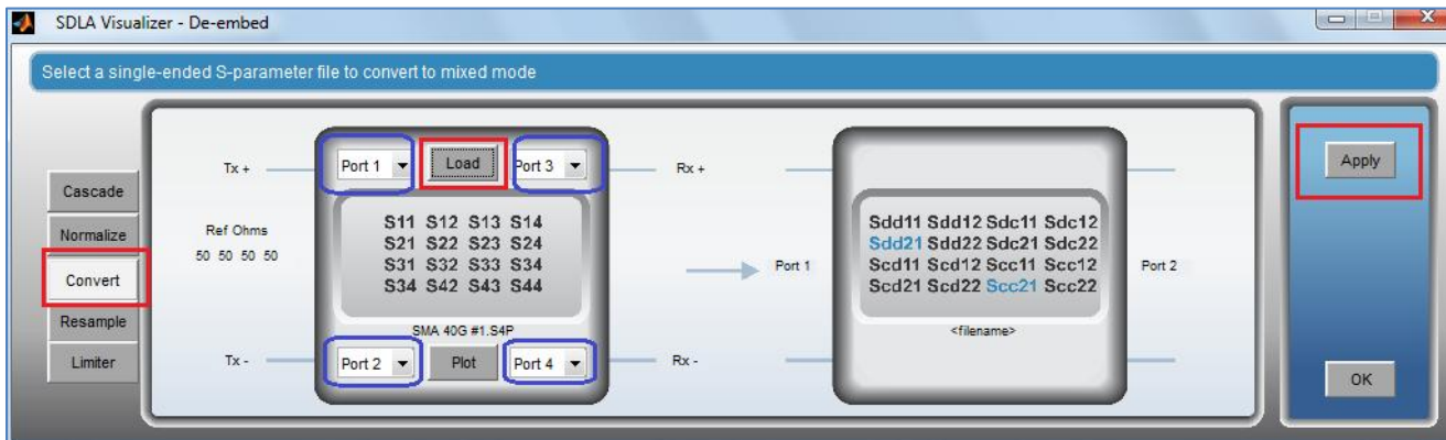
FIGURE 98. CONVERT TO MIXED MODE S-PARAMETERS
