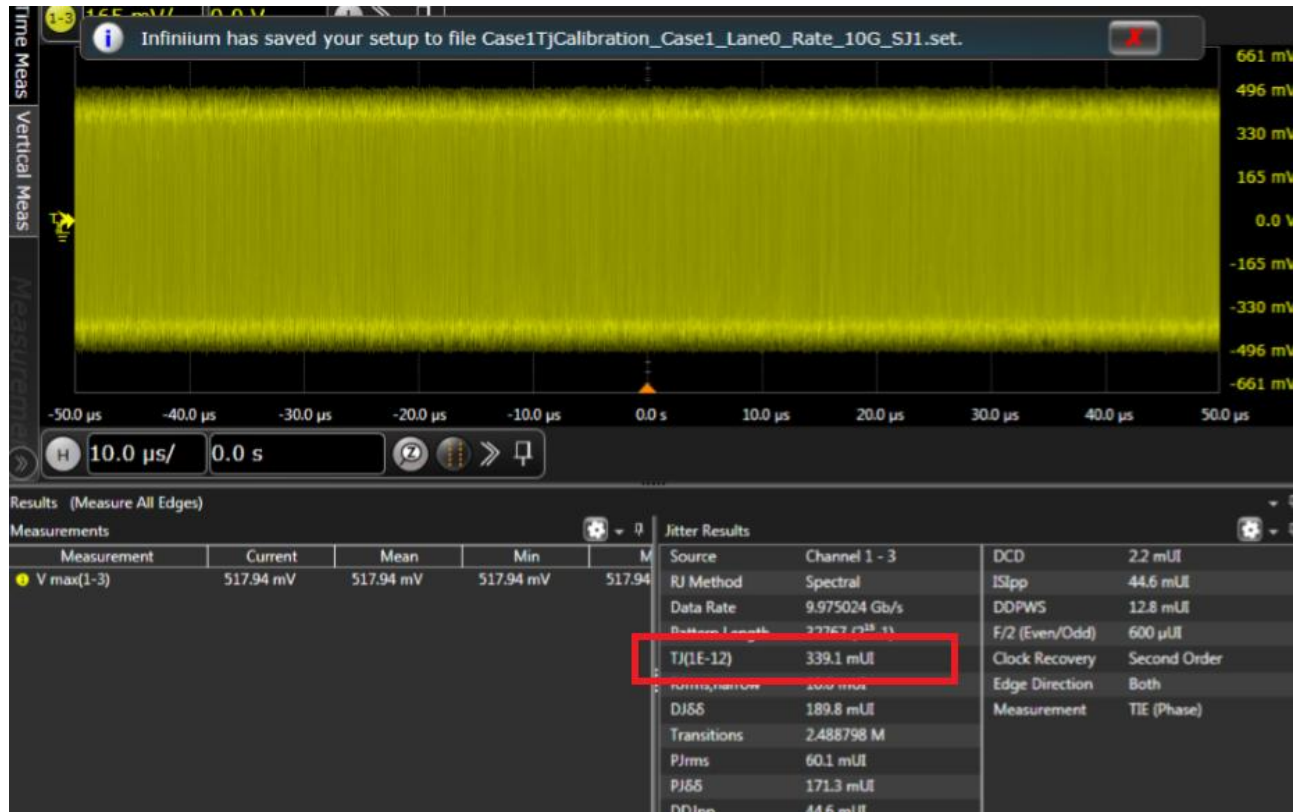
FIGURE 71. TJ MEASUREMENT ON KEYSIGHT SCOPE
