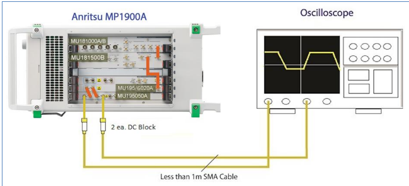
FIGURE 10. SETUP FOR TP3' (CASE 1) CALIBRATION
