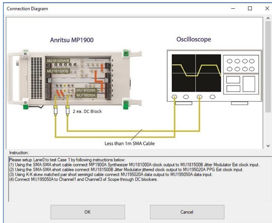
FIGURE 22. CONNECTION SETUP DIAGRAM DIALOG EXAMPLE
