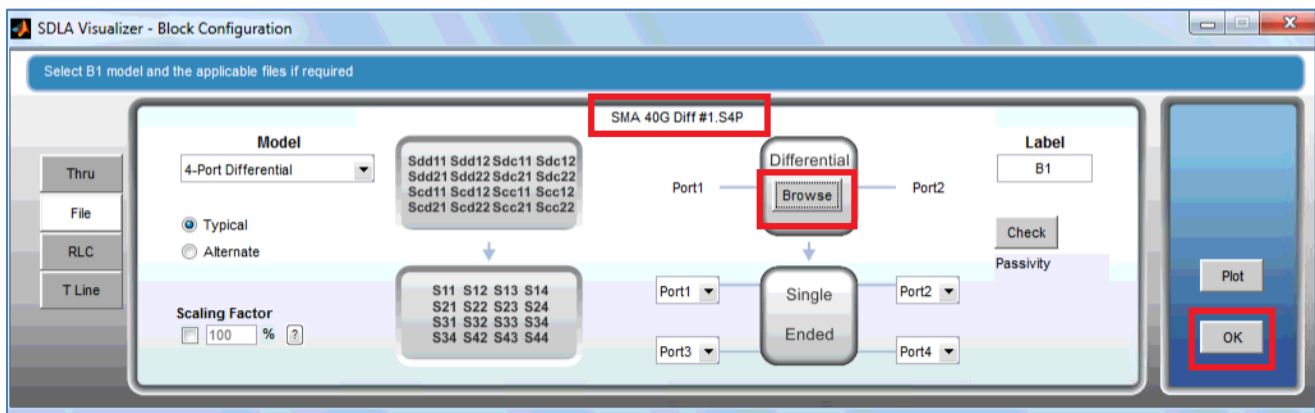
FIGURE 102. CREATE SMA CABLE DE-EMBEDDING FILES – #3
