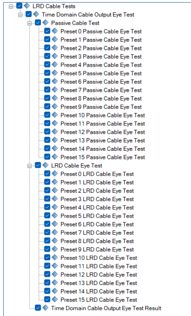
FIGURE 33. SELECT LRD CABLE TESTS TO BE RUN
