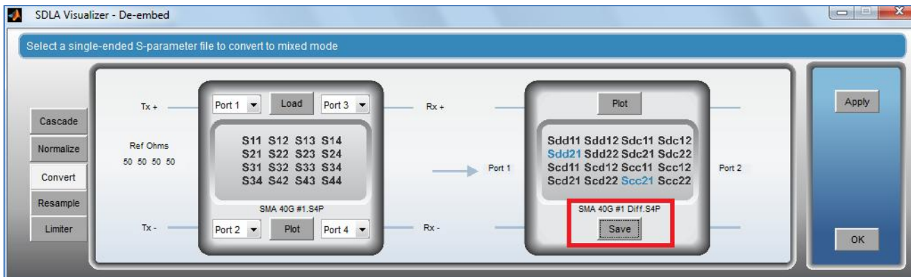
FIGURE 99. SAVE CONVERTED MIXED MODE S-PARAMETERS
