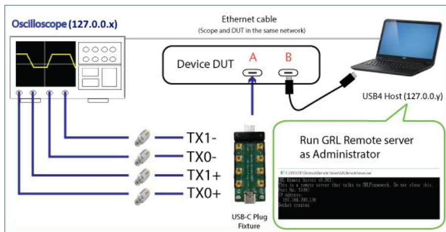
FIGURE 23. TEST SETUP FOR 2-PORT THUNDERBOLT 3 DEVICE DUT USING THUNDERBOLT 3 HOST PC AS CONTROLLER
