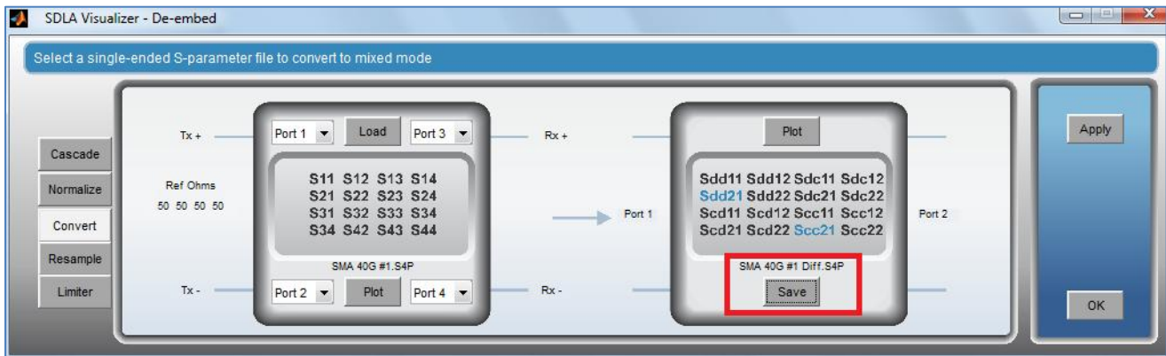
FIGURE 69. SAVE CONVERTED MIXED MODE S-PARAMETERS
