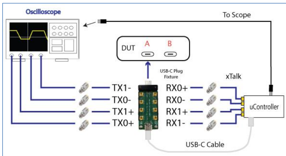
FIGURE 27. TEST SETUP WITH USB4 MICROCONTROLLER
