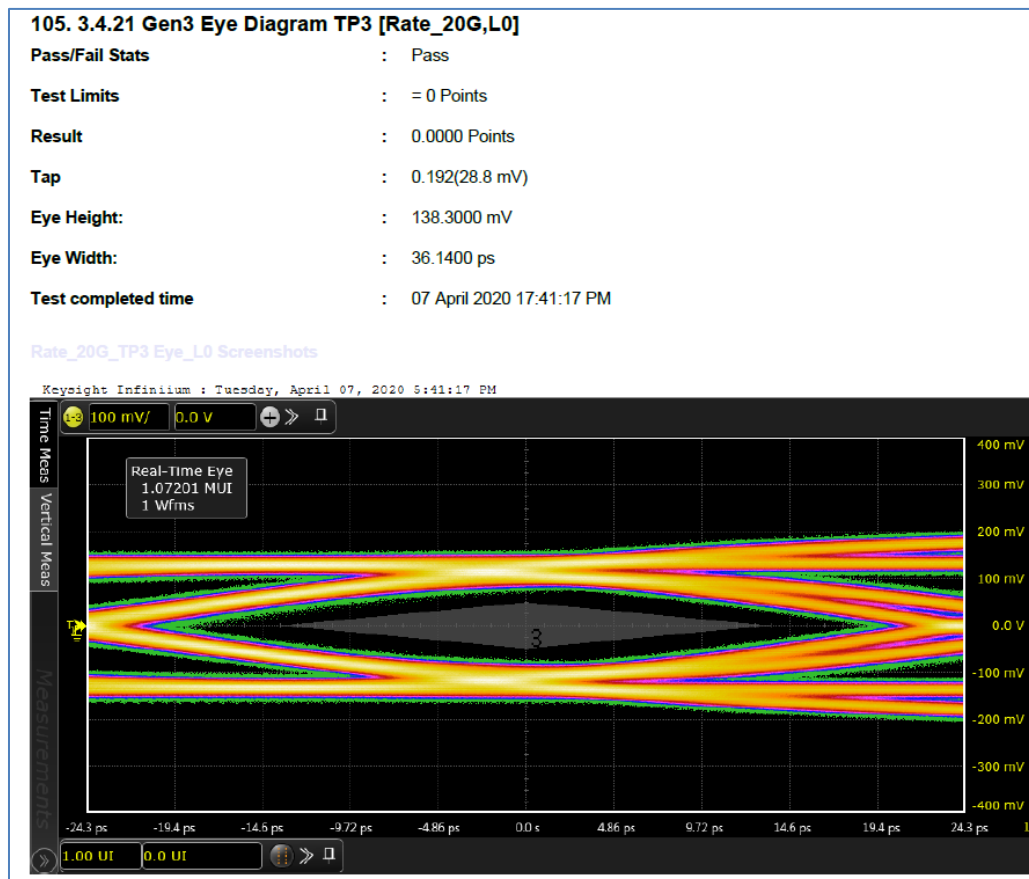
FIGURE 53. TEST RESULT DETAILS EXAMPLE
