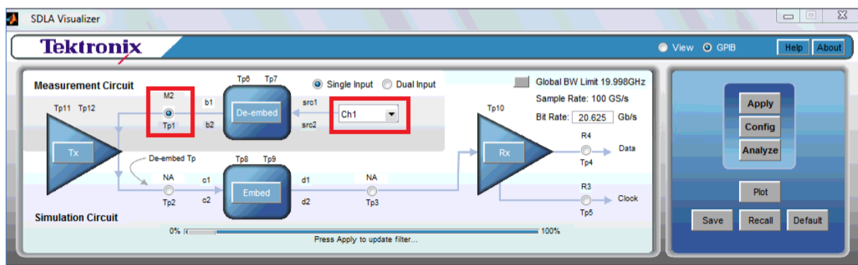
FIGURE 74. CREATE SMA CABLE DE-EMBEDDING FILES – #4
