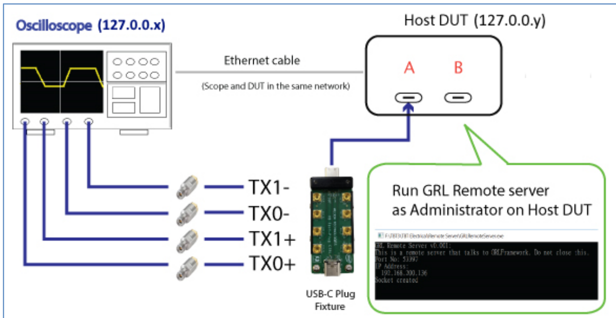
FIGURE 19. TEST SETUP FOR HOST DUT
