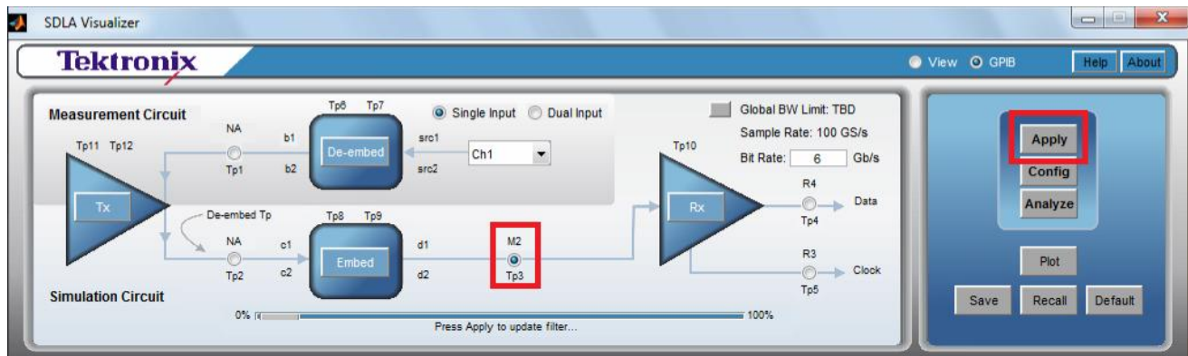
FIGURE 80. CREATE SMA CABLE DE-EMBEDDING + TP3 EMBEDDING FILES – #4
