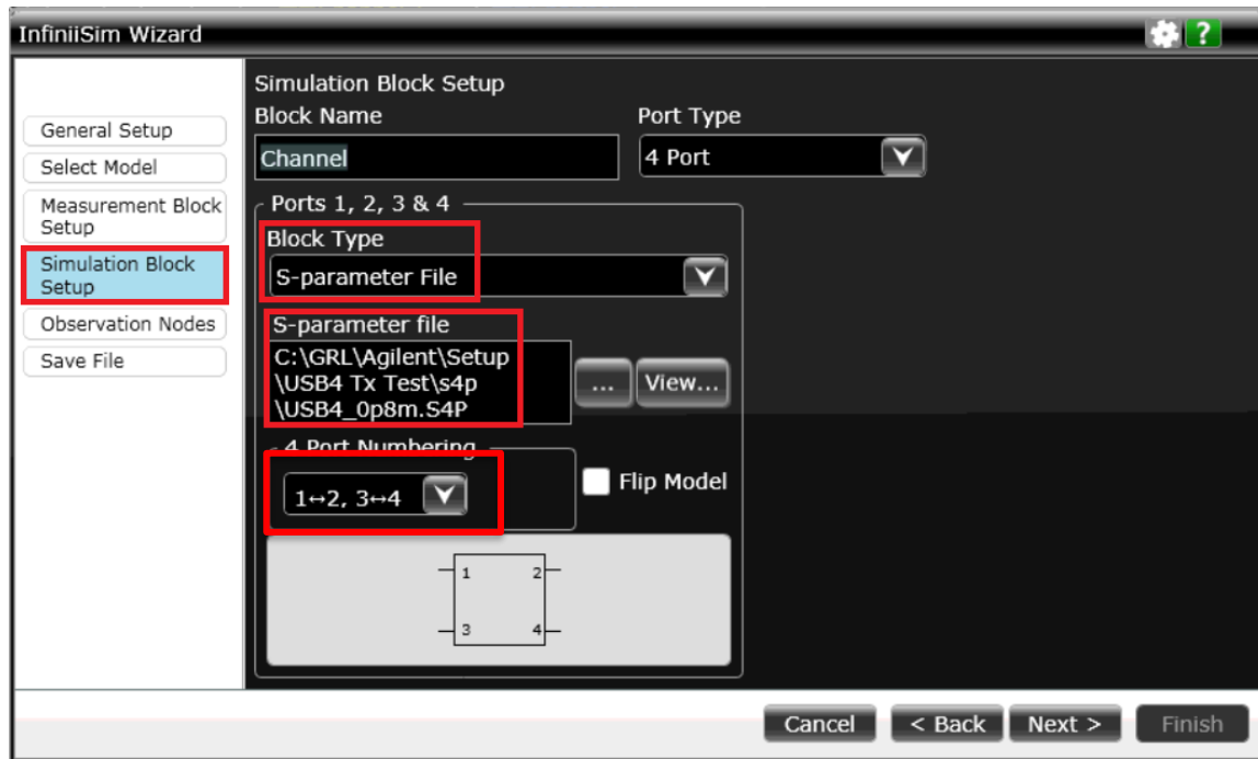
FIGURE 65. SMA CABLE TRANSFER FUNCTION- SET UP INFINIISIM ON SCOPE #7
