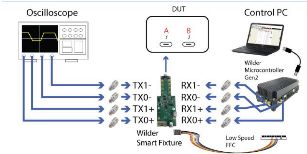
FIGURE 29. TEST SETUP WITH THUNDERBOLT 3 MICROCONTROLLER
