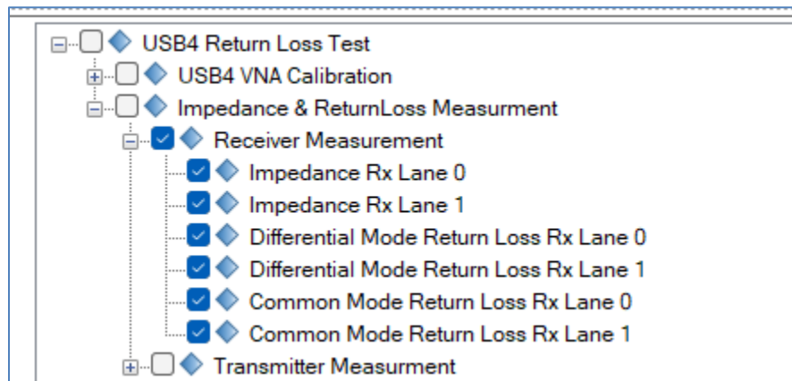
FIGURE 21. SELECT RX MEASUREMENT TESTS
