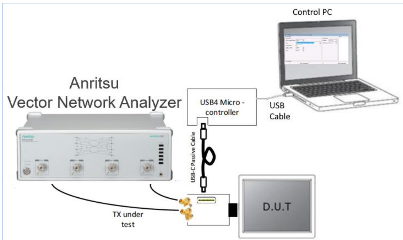
FIGURE 17. TEST SETUP FOR HOST DUT
