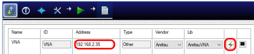
FIGURE 7. GRL TEST SOLUTION IP ADDRESSING ON VNA
